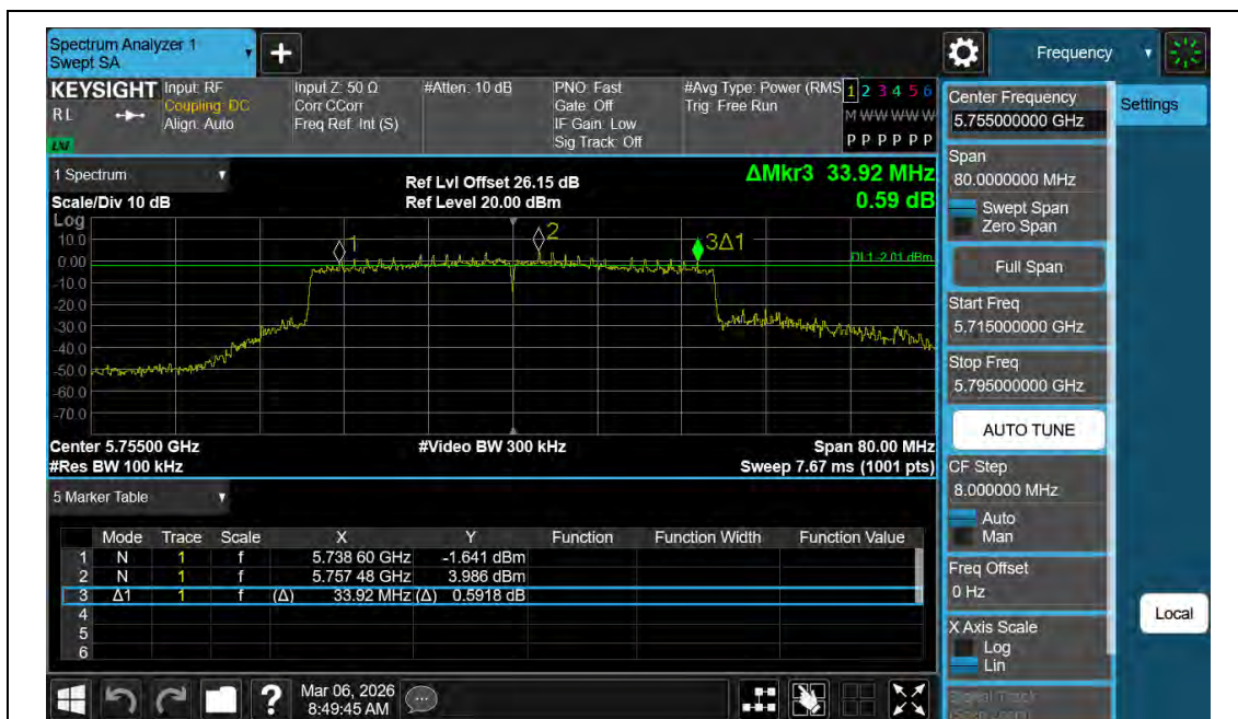
11BE40MIMO-Ant2-5755-PASS
