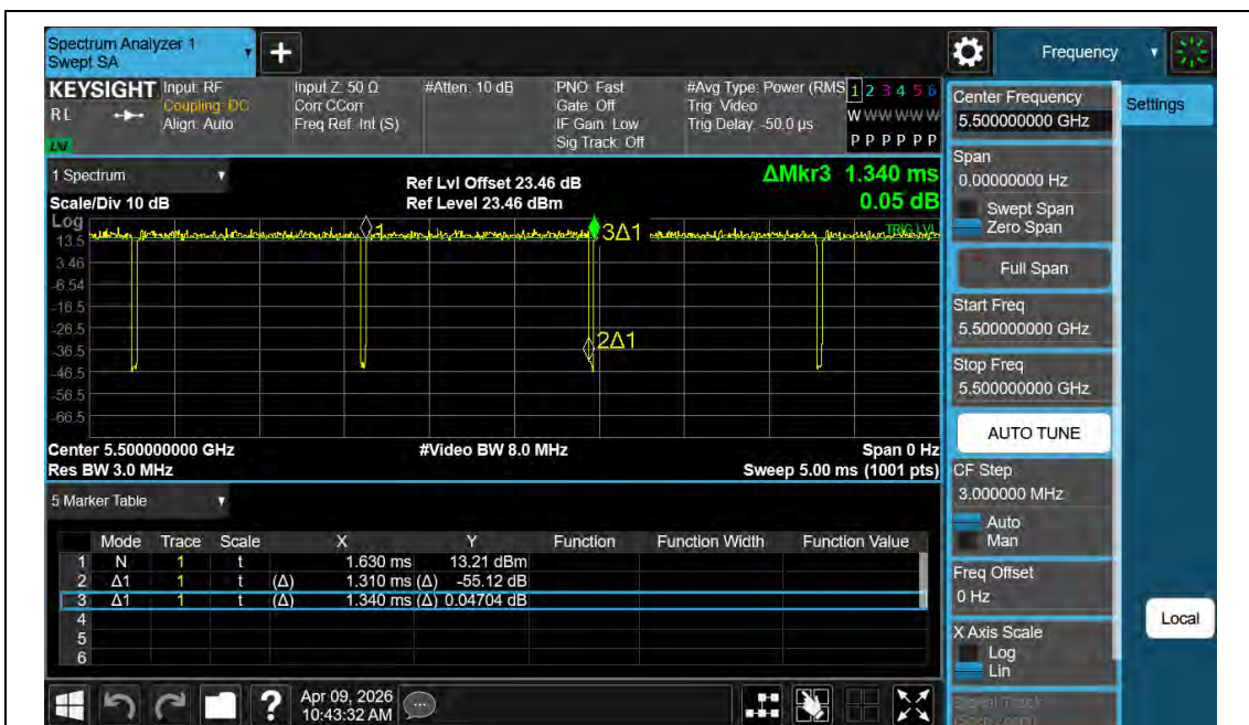
NTNV-11N20MIMO-Ant2-5500
