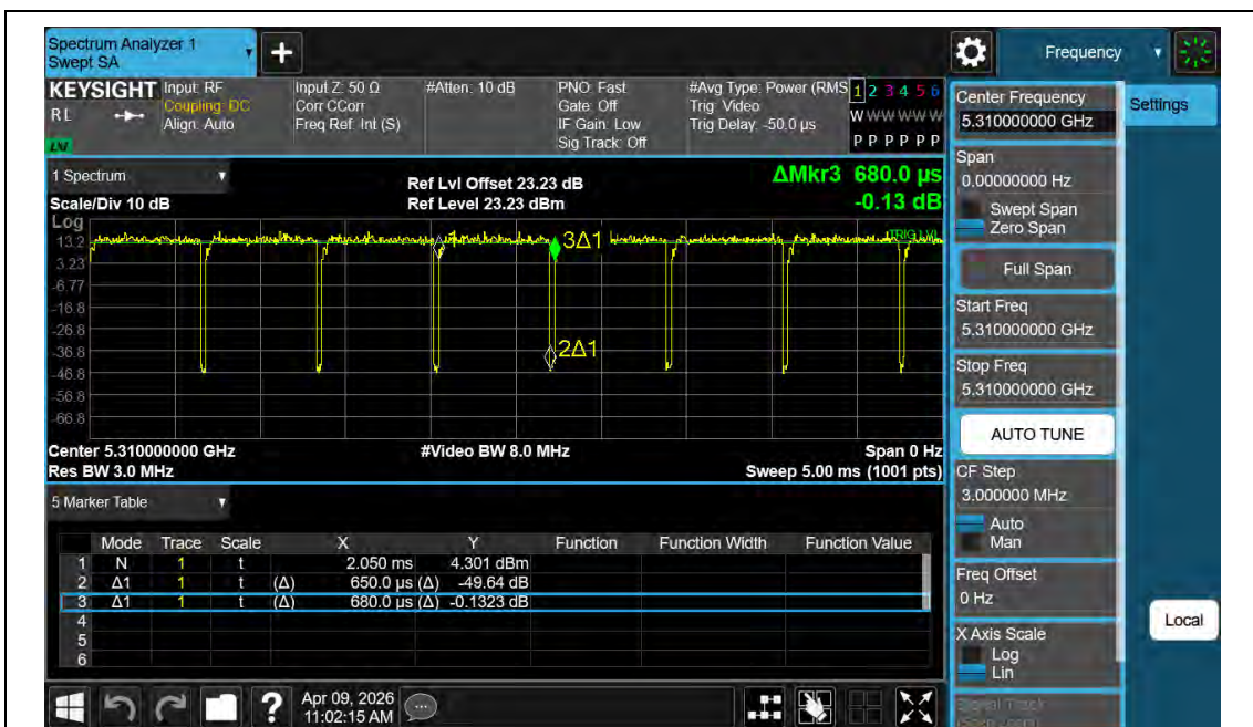
NTNV-11N40MIMO-Ant2-5310
