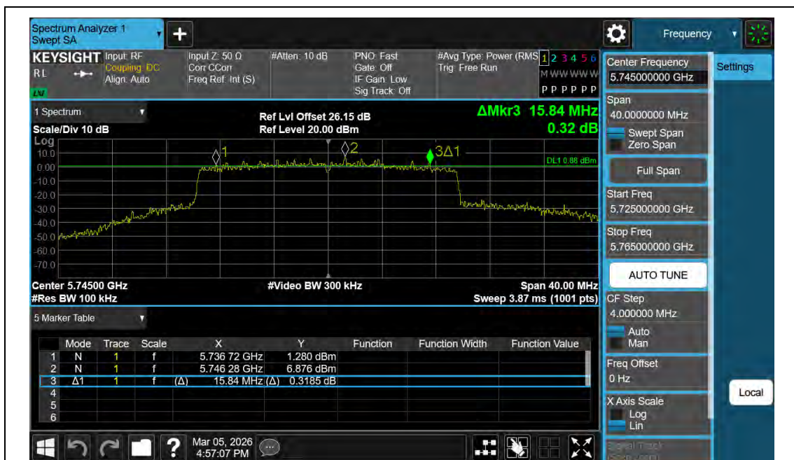
11BE20MIMO-Ant2-5745-PASS
