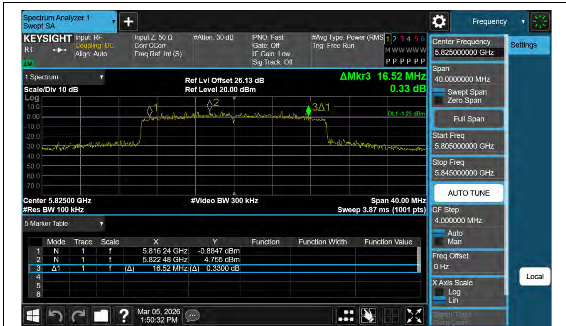
11AX20MIMO-Ant2-5825-PASS
