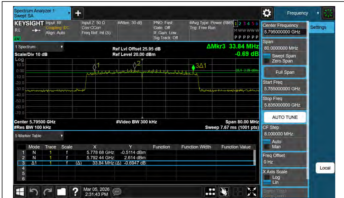
11AX40MIMO-Ant2-5795-PASS
