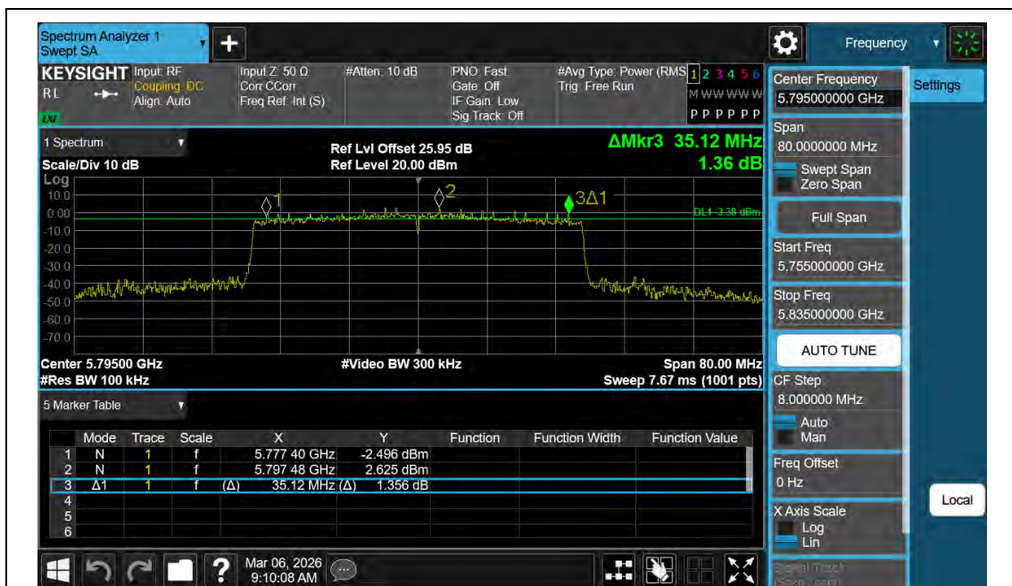
11BE40MIMO-Ant2-5795-PASS
