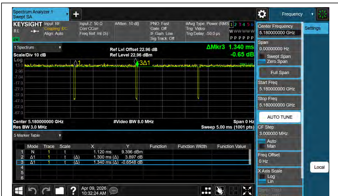
NTNV-11N20MIMO-Ant2-5180
