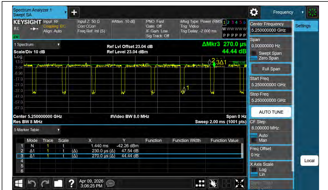
NTNV-11AC160MIMO-Ant2-5250
