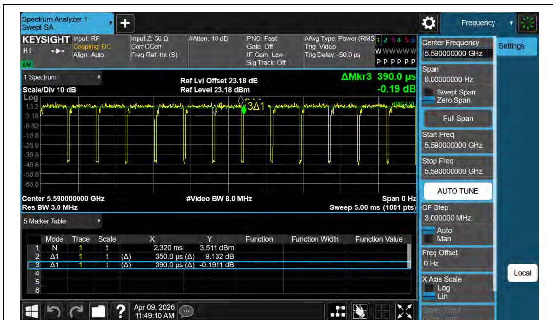
NTNV-11AC40MIMO-Ant2-5590
