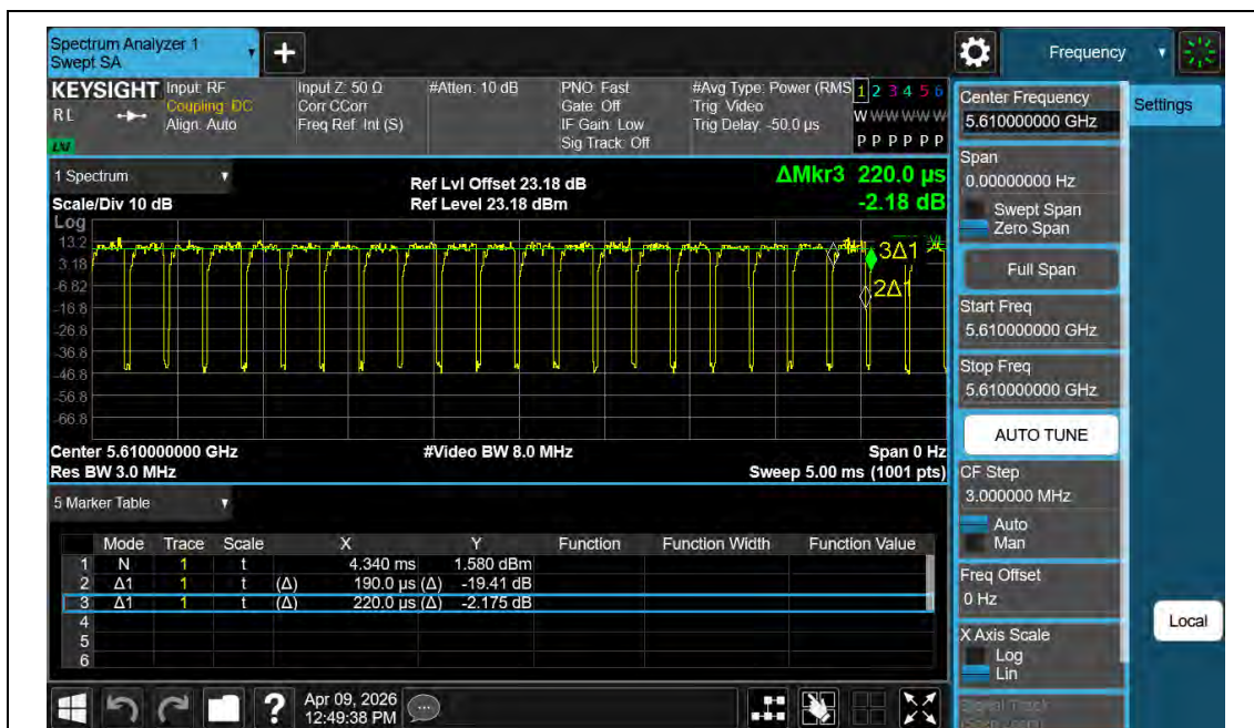
NTNV-11AC80MIMO-Ant2-5610
