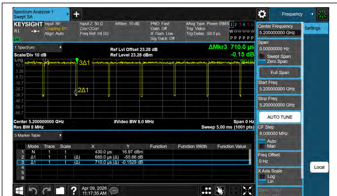
NTNV-11AC20MIMO-Ant2-5200
