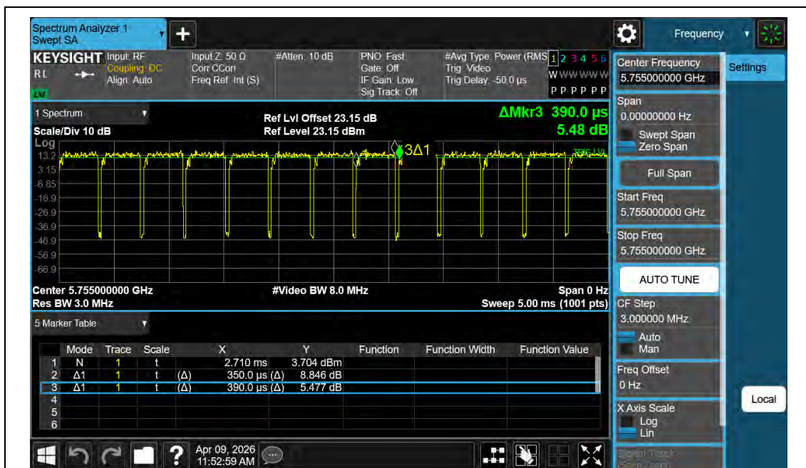
NTNV-11AC40MIMO-Ant2-5755
