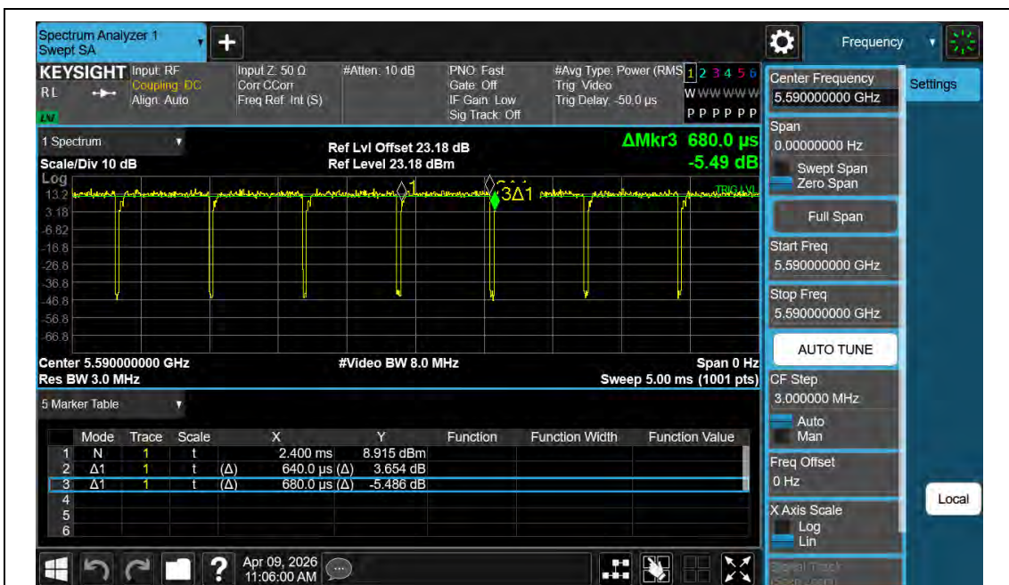
NTNV-11N40MIMO-Ant2-5590
