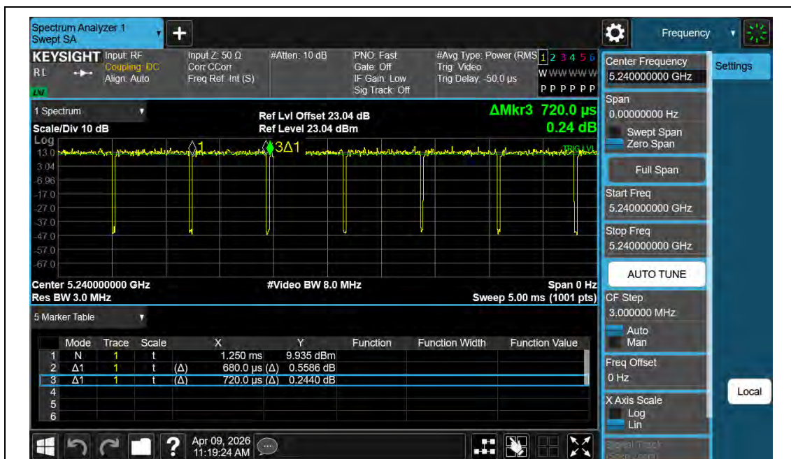
NTNV-11AC20MIMO-Ant2-5240
