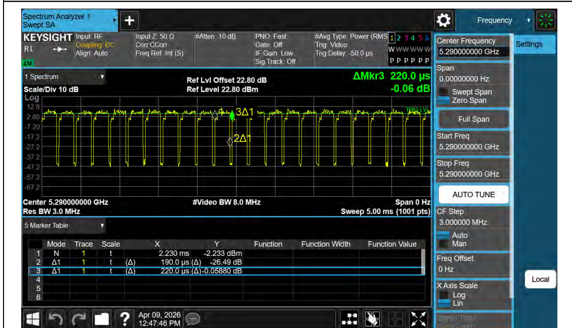
NTNV-11AC80MIMO-Ant1-5530
