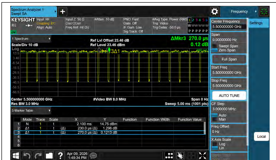
NTNV-11AX20MIMO-Ant2-5500
