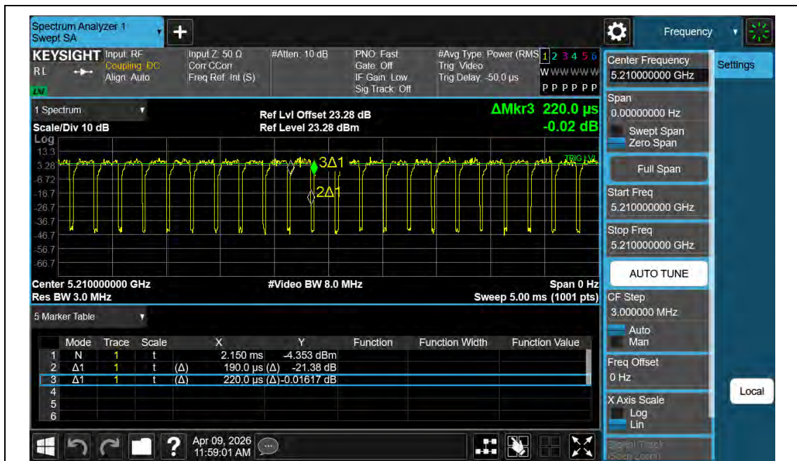
NTNV-11AC80MIMO-Ant2-5210
