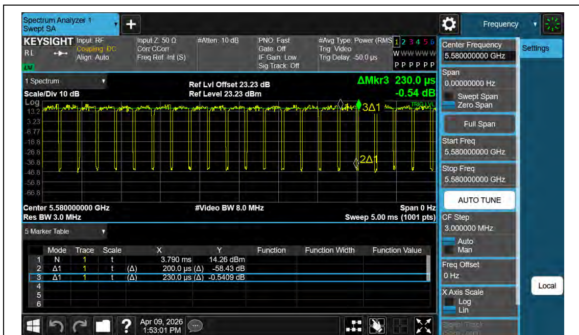
NTNV-11AX20MIMO-Ant2-5580
