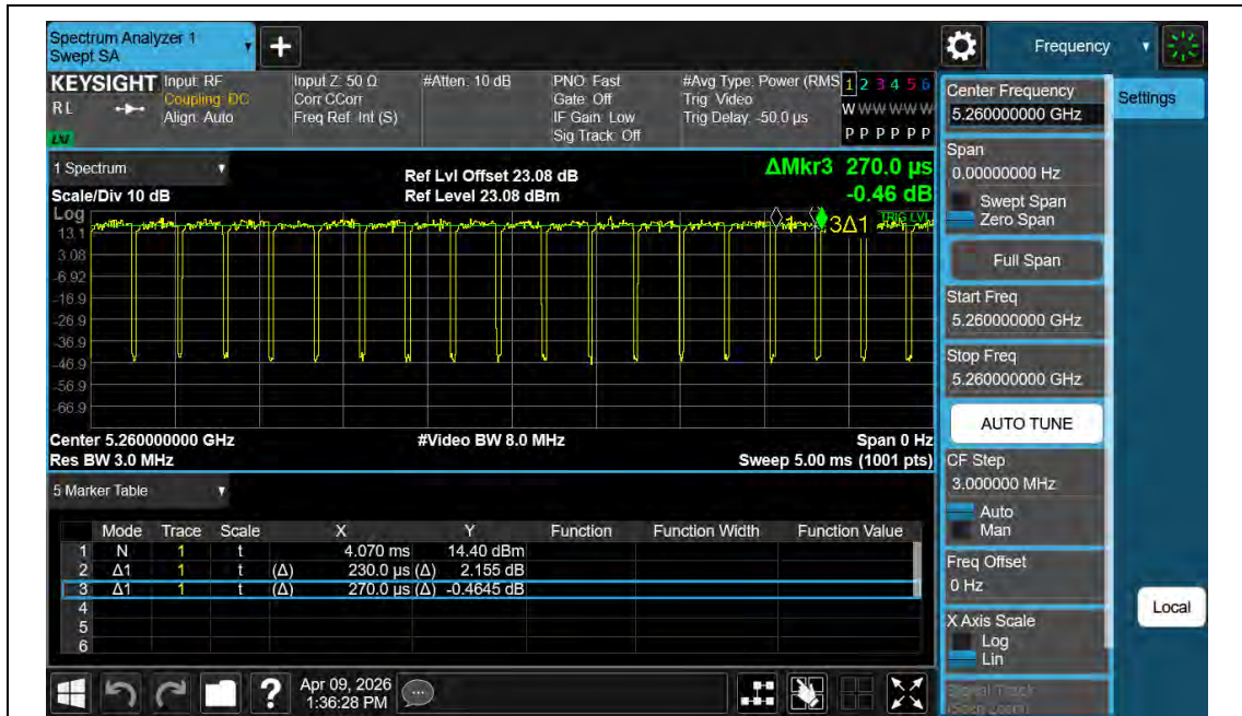
NTNV-11AX20MIMO-Ant2-5260
