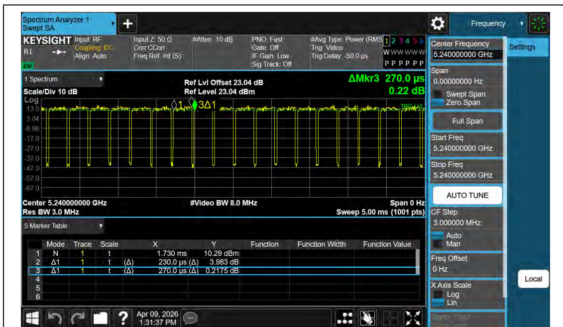
NTNV-11AX20MIMO-Ant2-5240
