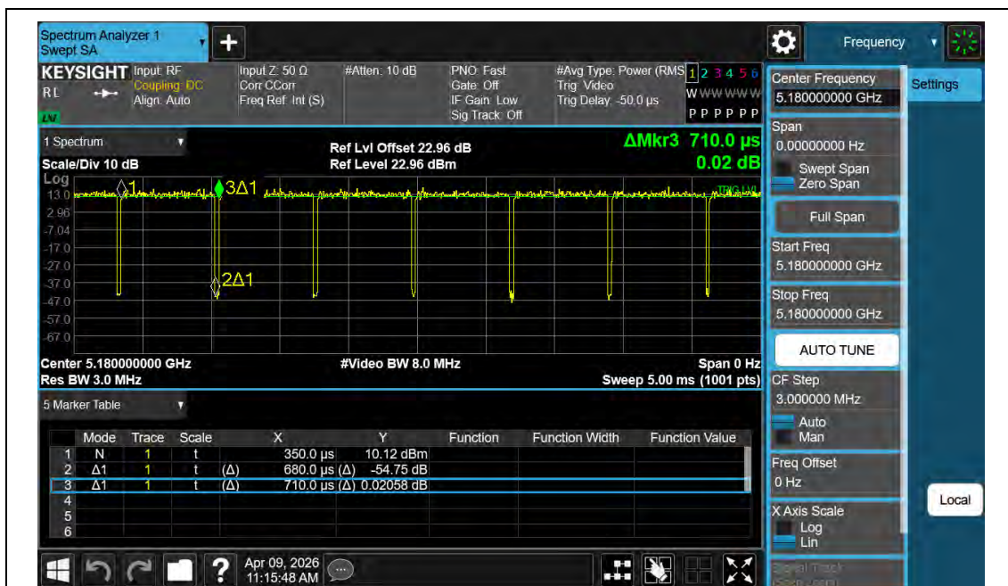
NTNV-11AC20MIMO-Ant2-5180
