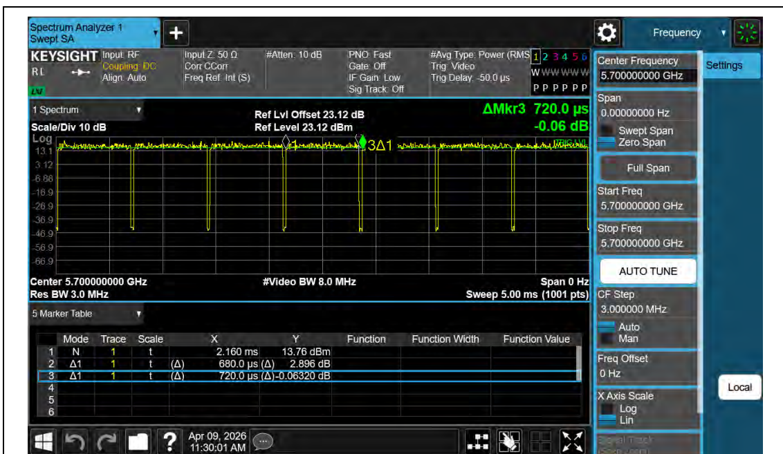
NTNV-11AC20MIMO-Ant2-5700
