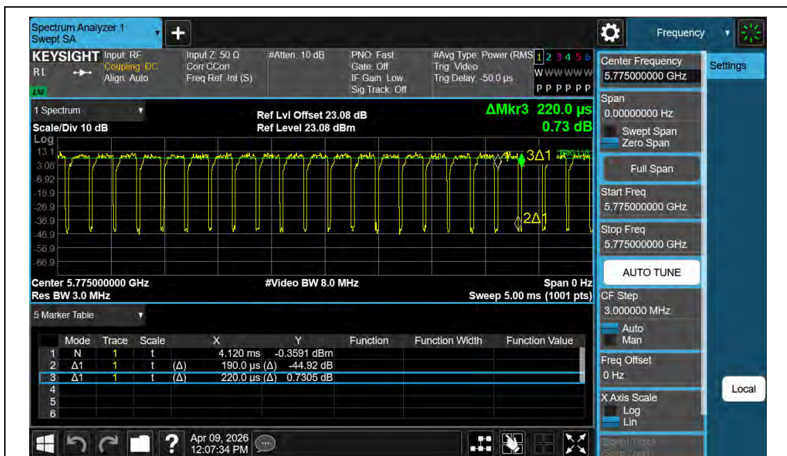
NTNV-11AC80MIMO-Ant2-5775
