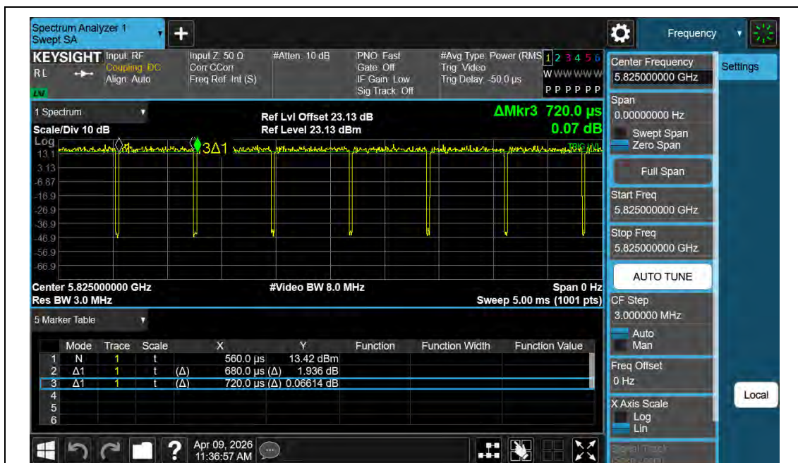
NTNV-11AC20MIMO-Ant2-5825
