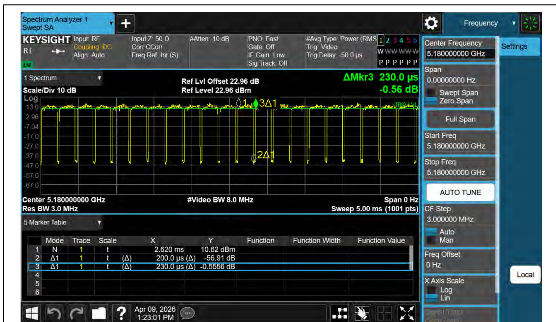
NTNV-11AX20MIMO-Ant2-5180
