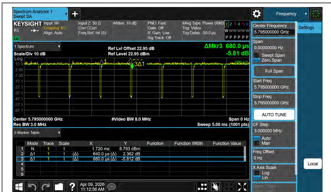
NTNV-11N40MIMO-Ant2-5795
