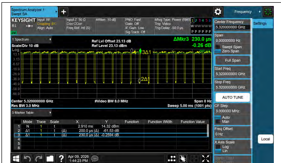
NTNV-11AX20MIMO-Ant2-5320
