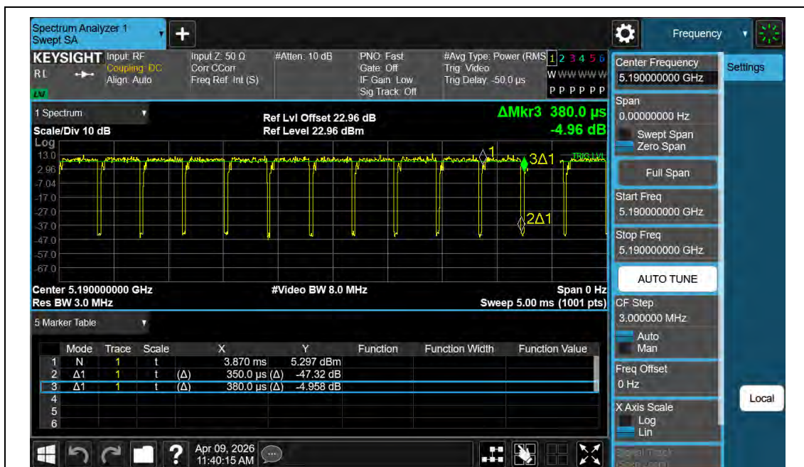
NTNV-11AC40MIMO-Ant2-5190
