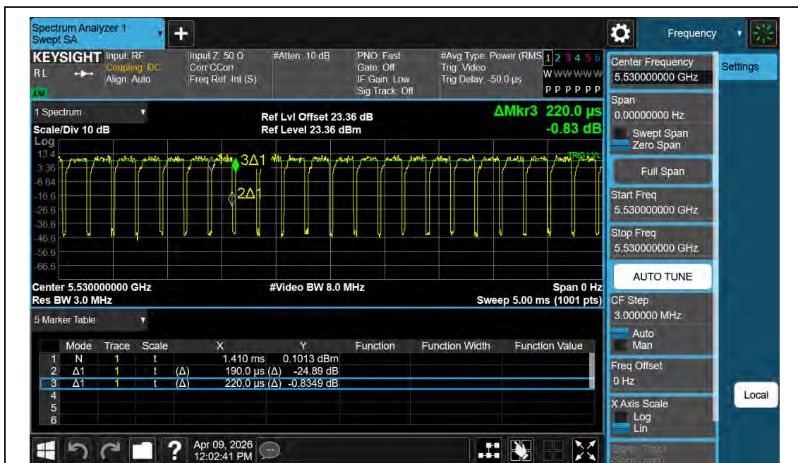
NTNV-11AC80MIMO-Ant2-5530
