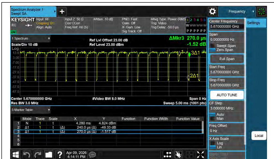
NTNV-11BE40MIMO-Ant2-5670
