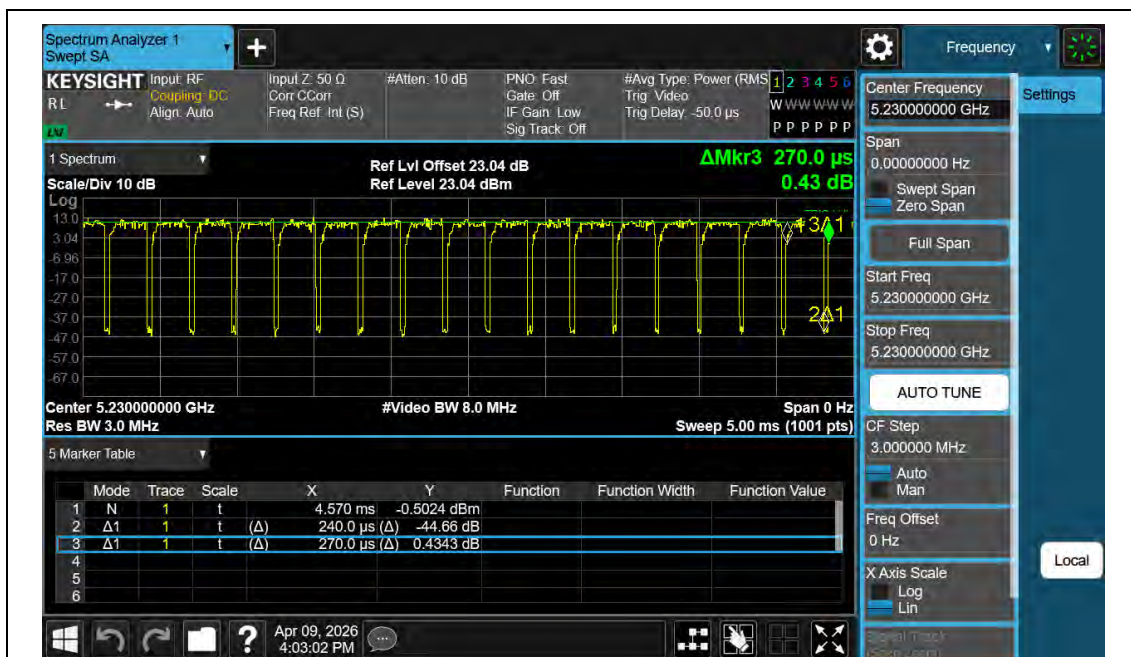
NTNV-11BE40MIMO-Ant2-5230
