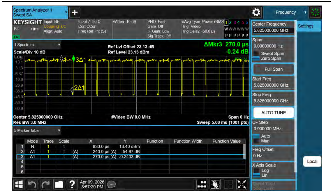
NTNV-11BE20MIMO-Ant2-5825
