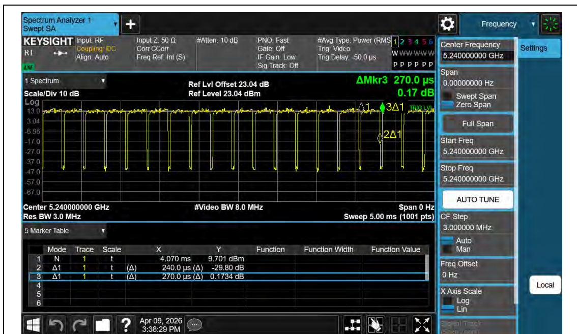
NTNV-11BE20MIMO-Ant2-5240
