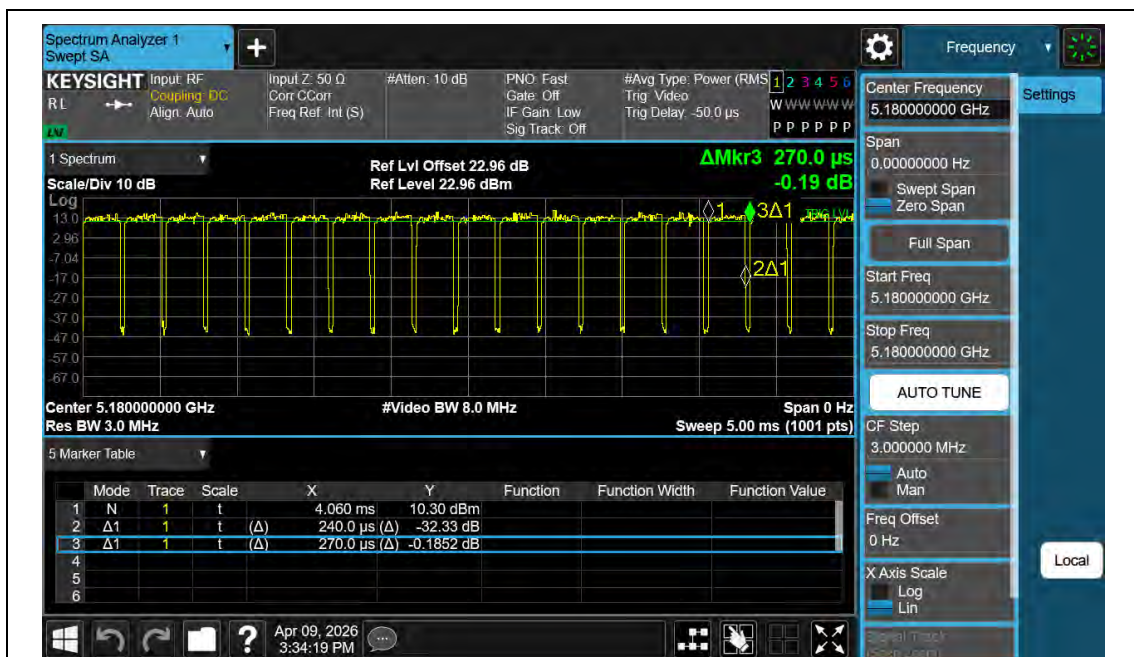
NTNV-11BE20MIMO-Ant2-5180
