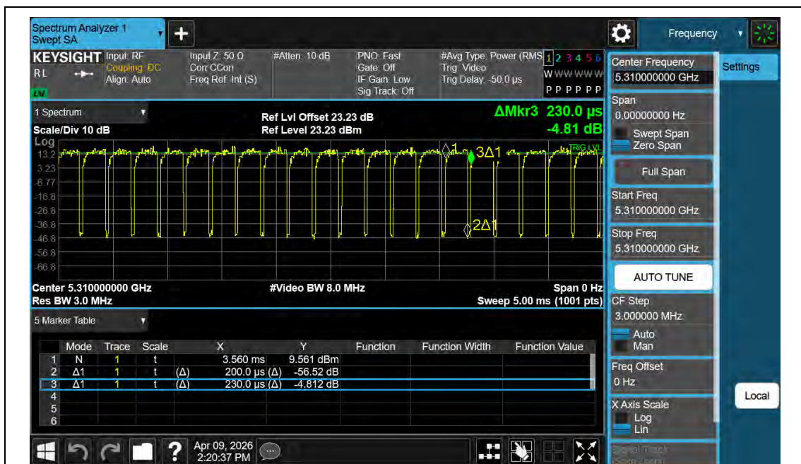
NTNV-11AX40MIMO-Ant2-5310
