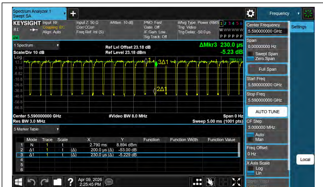
NTNV-11AX40MIMO-Ant2-5590
