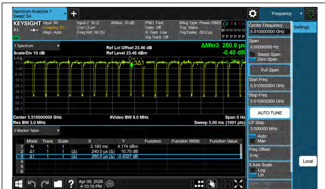
NTNV-11BE40MIMO-Ant2-5510
