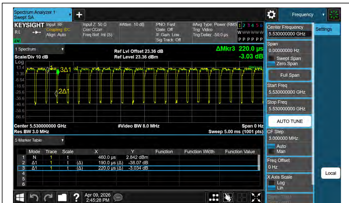
NTNV-11AX80MIMO-Ant2-5530
