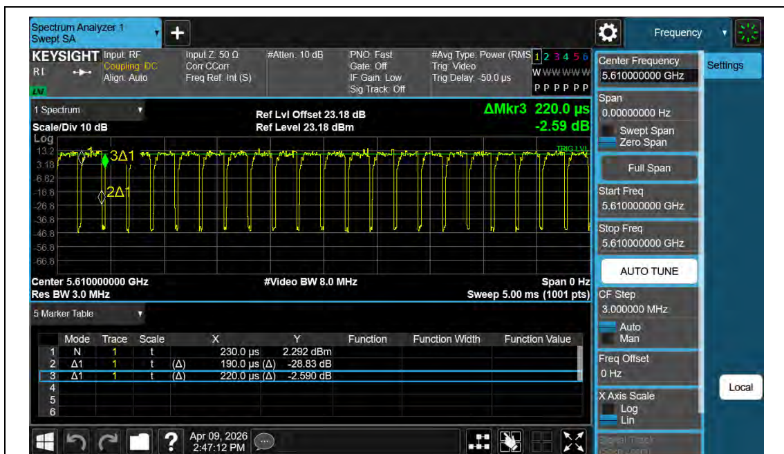
NTNV-11AX80MIMO-Ant2-5610
