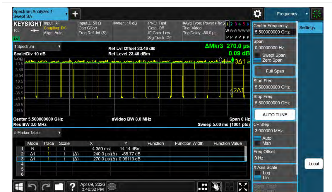
NTNV-11BE20MIMO-Ant2-5500
