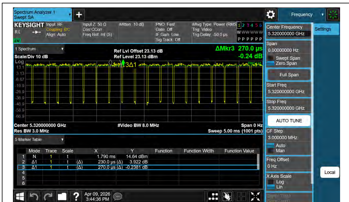
NTNV-11BE20MIMO-Ant2-5320
