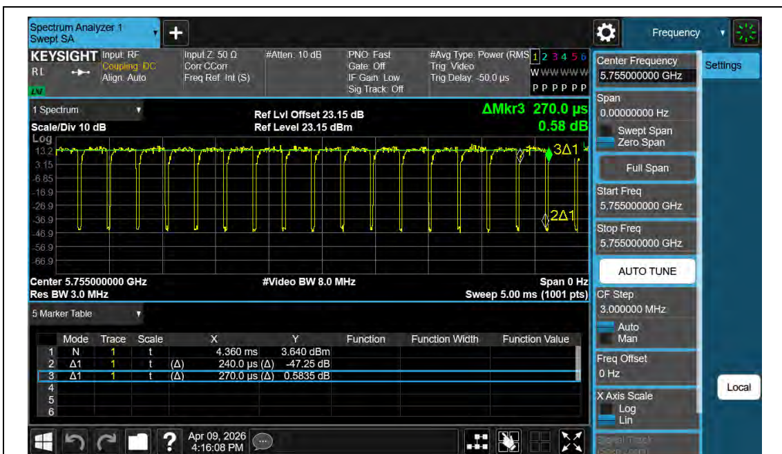
NTNV-11BE40MIMO-Ant2-5755
