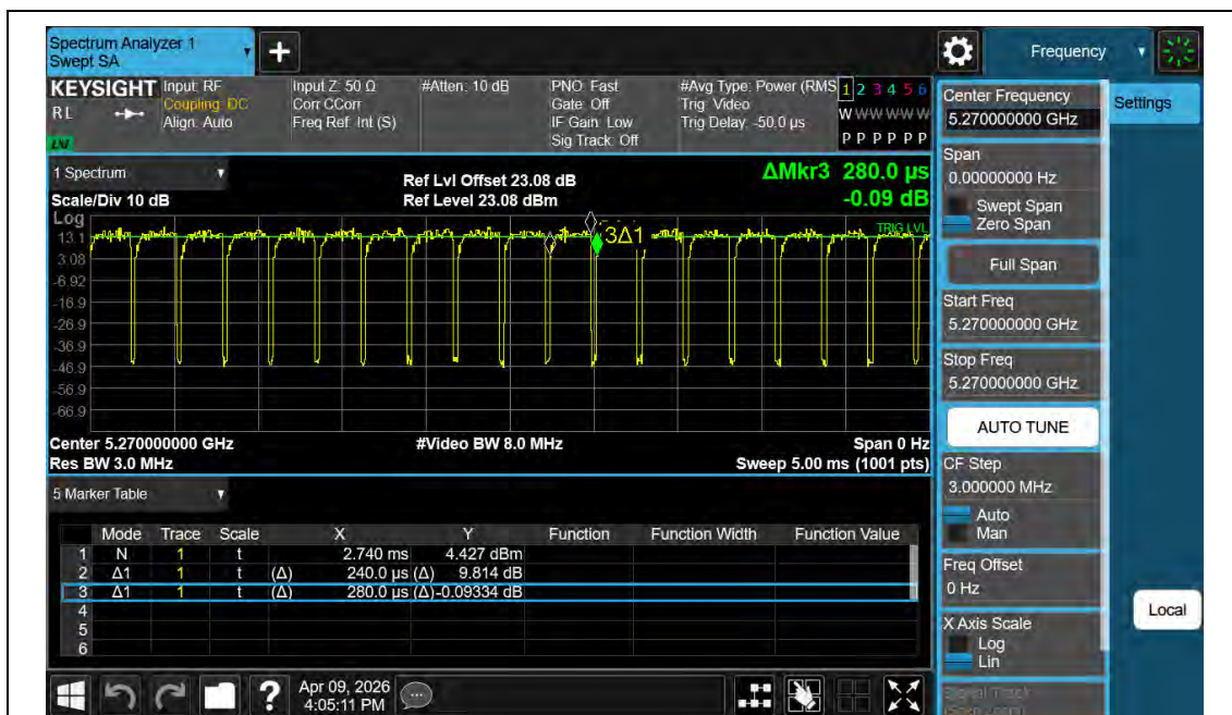
NTNV-11BE40MIMO-Ant2-5270
