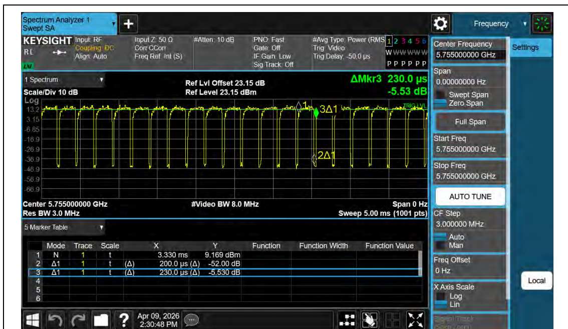
NTNV-11AX40MIMO-Ant2-5755
