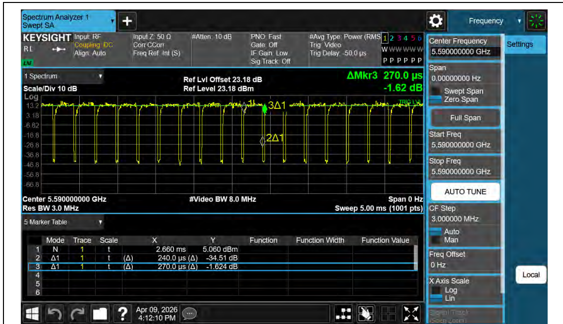
NTNV-11BE40MIMO-Ant2-5590
