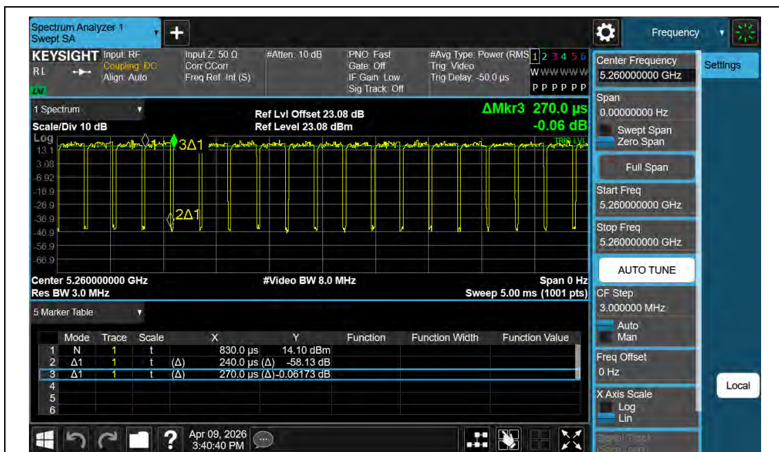
NTNV-11BE20MIMO-Ant2-5260
