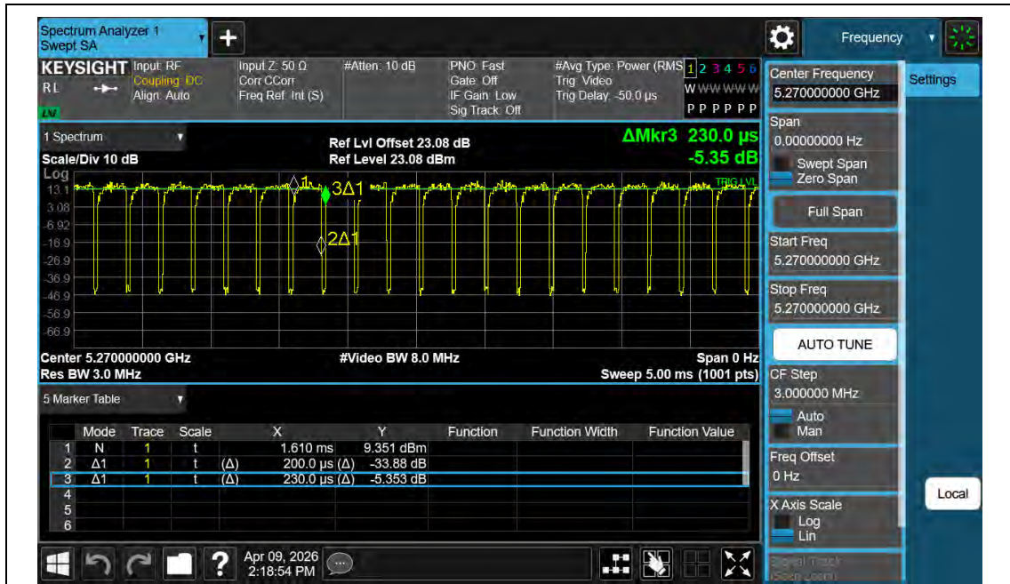
NTNV-11AX40MIMO-Ant2-5270
