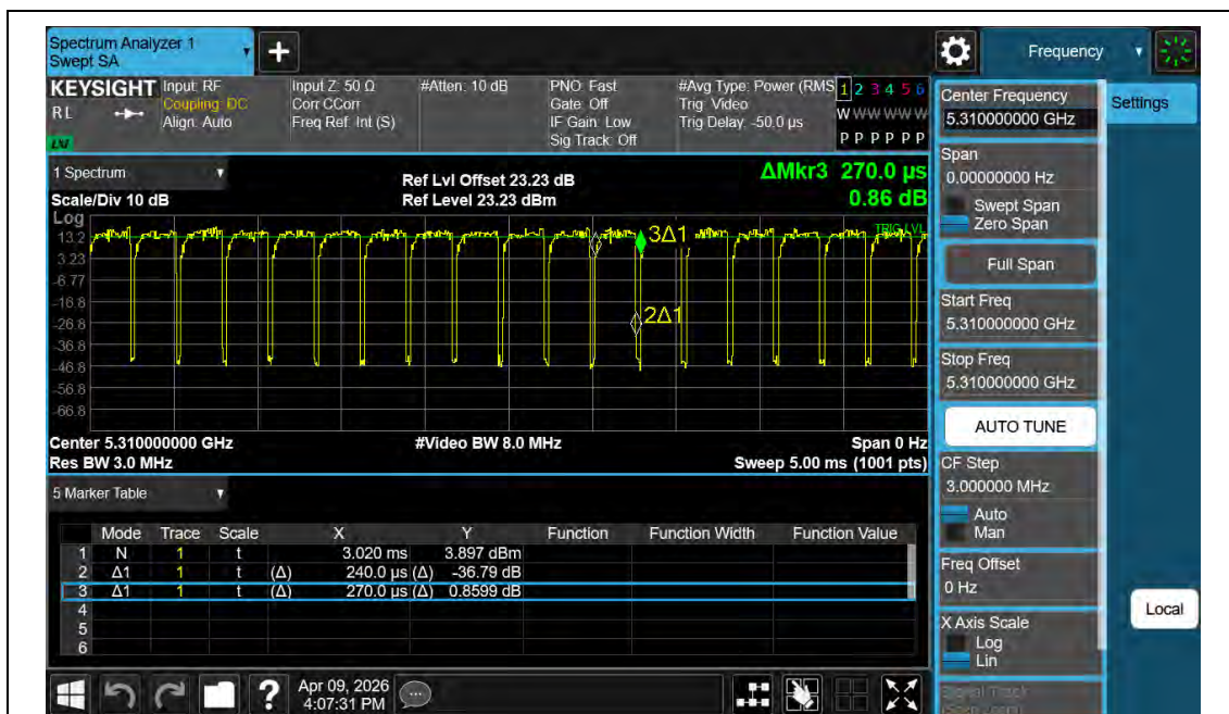
NTNV-11BE40MIMO-Ant2-5310
