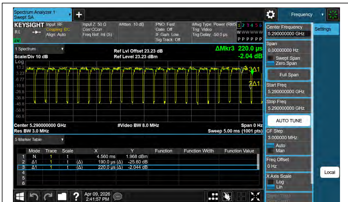
NTNV-11AX80MIMO-Ant2-5290
