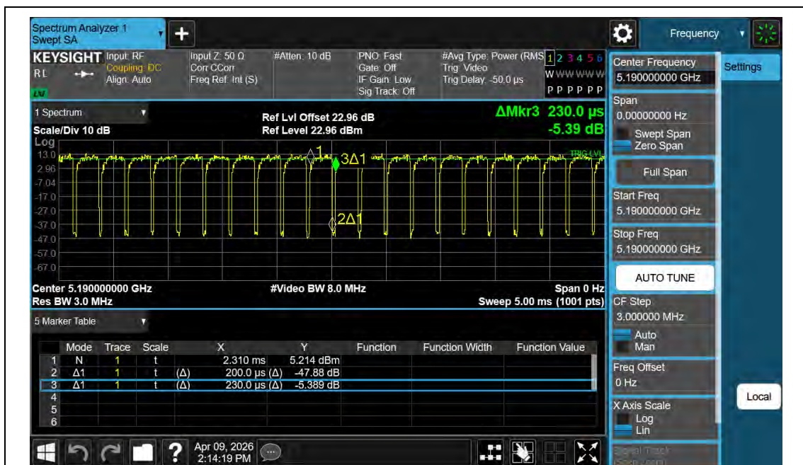
NTNV-11AX40MIMO-Ant2-5190
