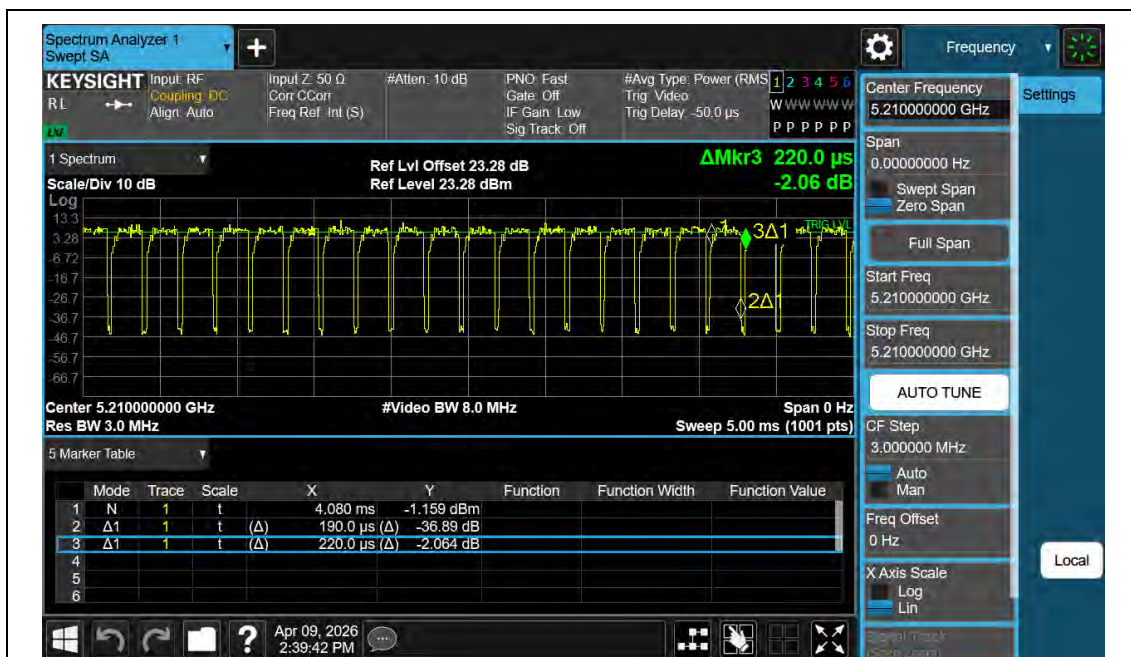
NTNV-11AX80MIMO-Ant2-5210
