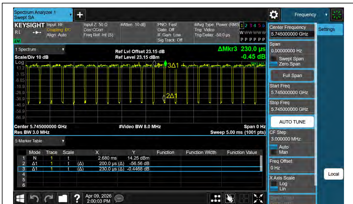
NTNV-11AX20MIMO-Ant2-5745
