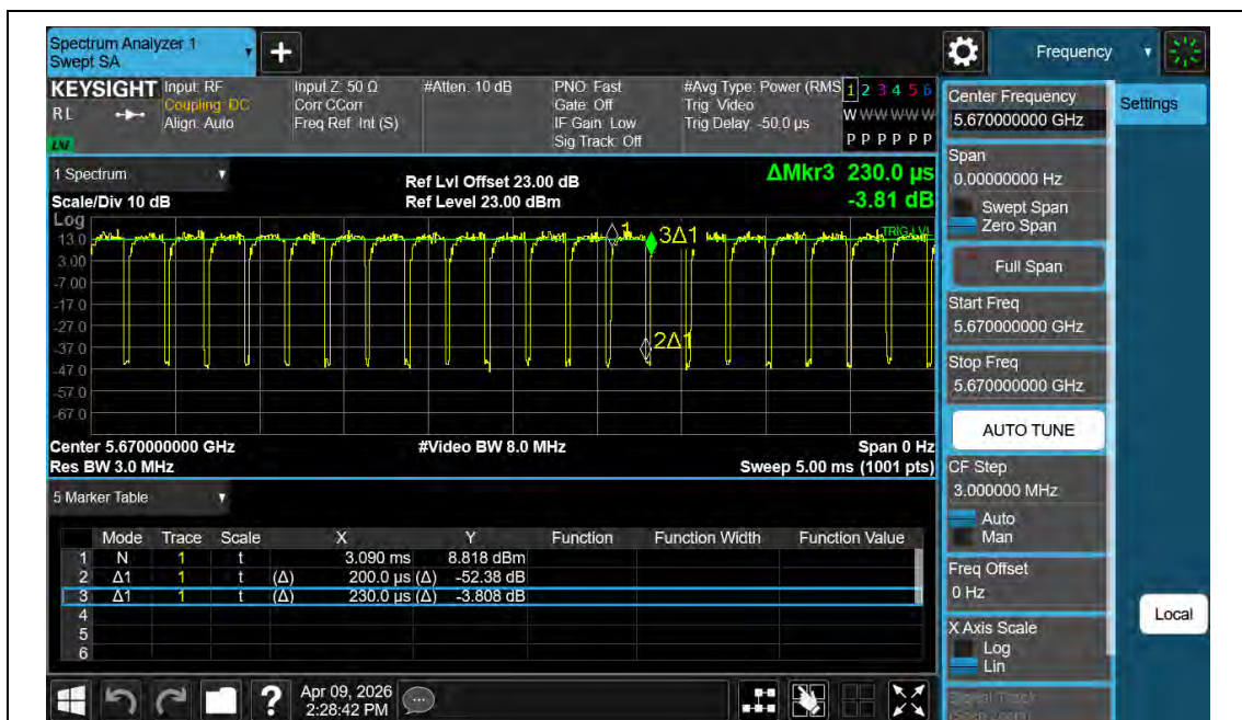
NTNV-11AX40MIMO-Ant2-5670
