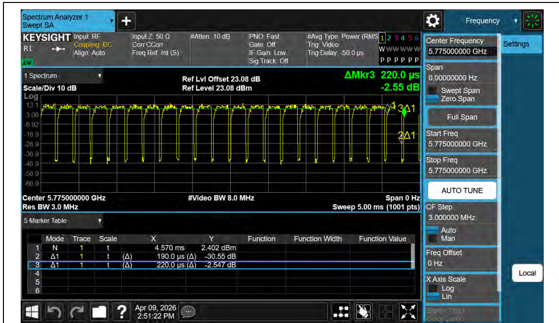
NTNV-11AX80MIMO-Ant2-5775
