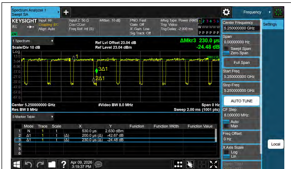
NTNV-11AX160MIMO-Ant2-5250
