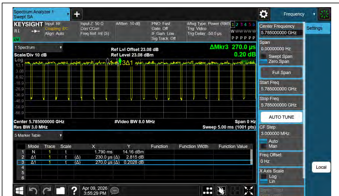
NTNV-11BE20MIMO-Ant2-5785
