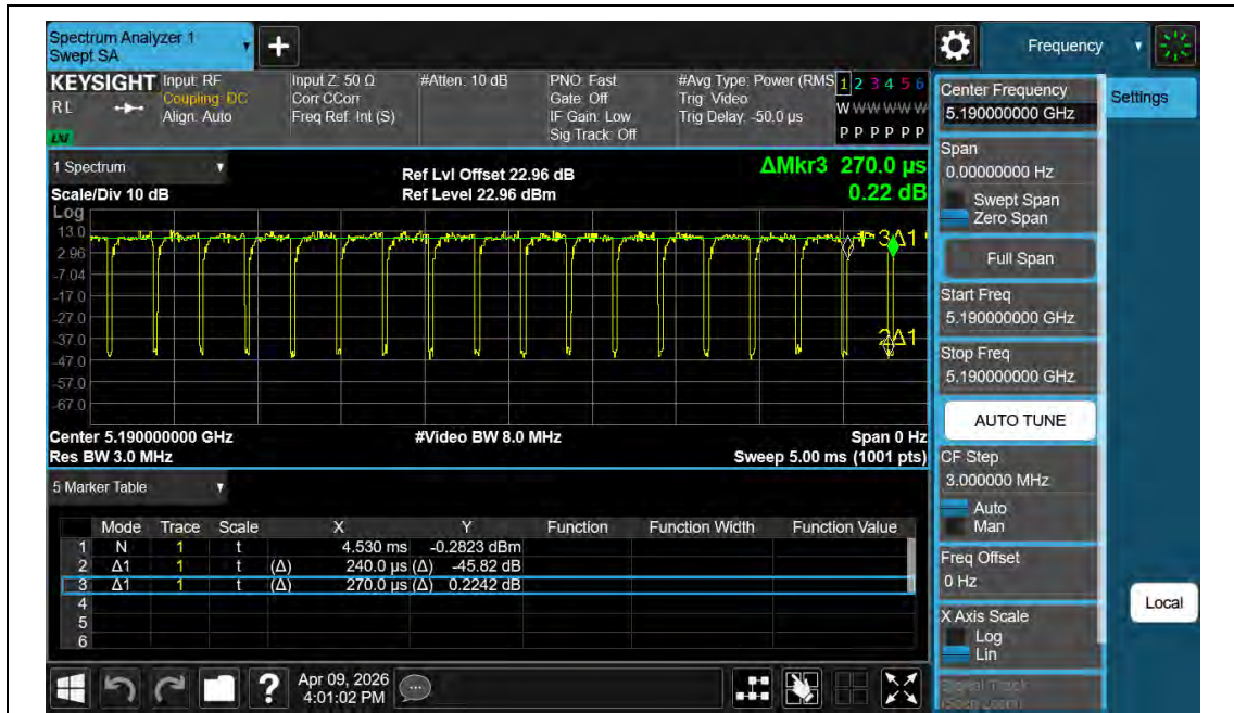
NTNV-11BE40MIMO-Ant2-5190
