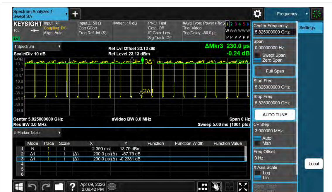
NTNV-11AX20MIMO-Ant2-5825
