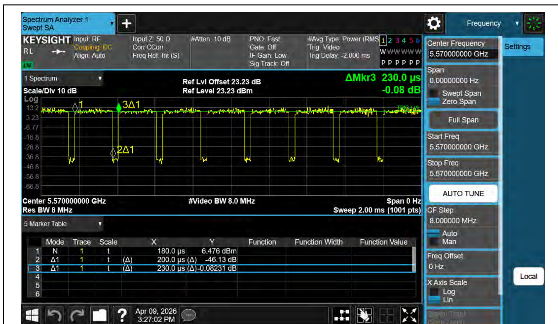
NTNV-11AX160MIMO-Ant2-5570
