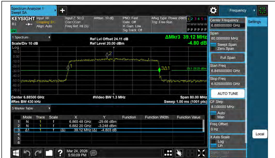
11AX40MIMO-Ant2-6885
