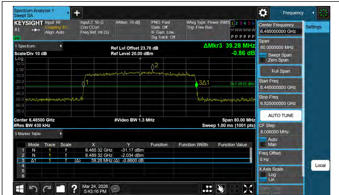
11AX40MIMO-Ant2-6485
