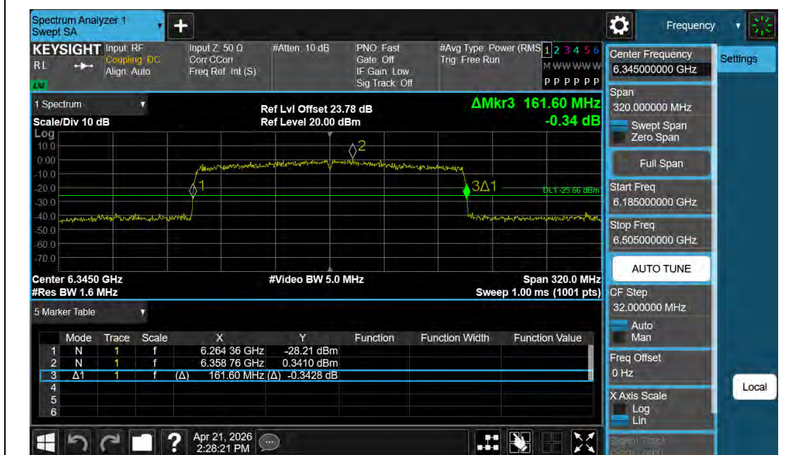
11AX160MIMO-Ant1-6505
