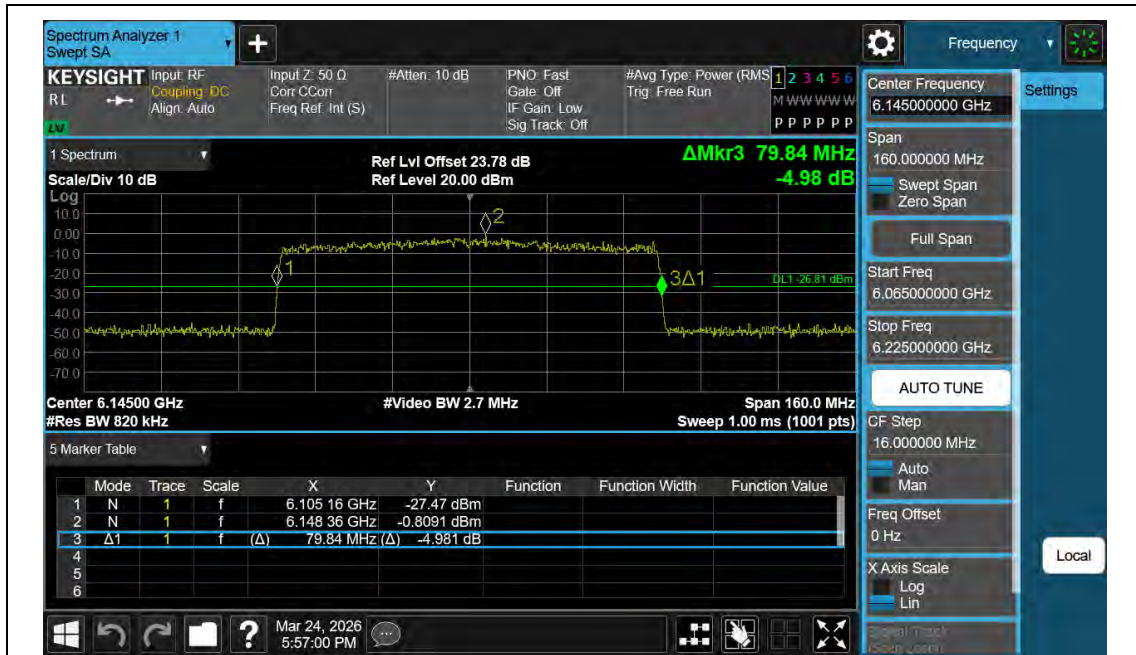
11AX80MIMO-Ant2-6145
