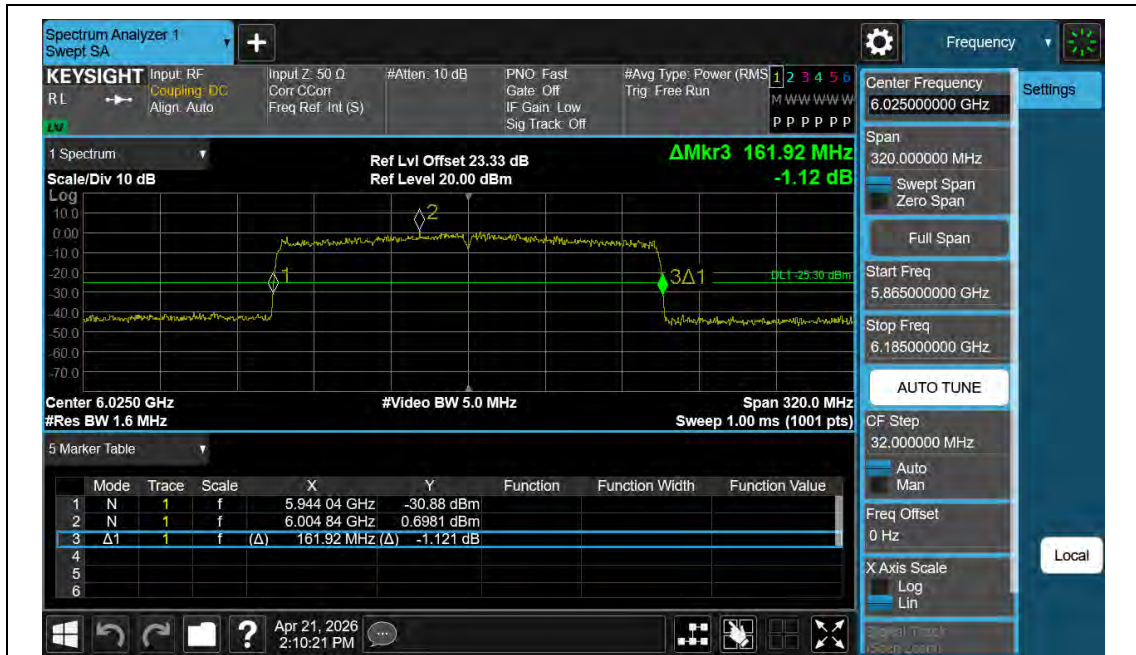
11AX160MIMO-Ant2-6025
