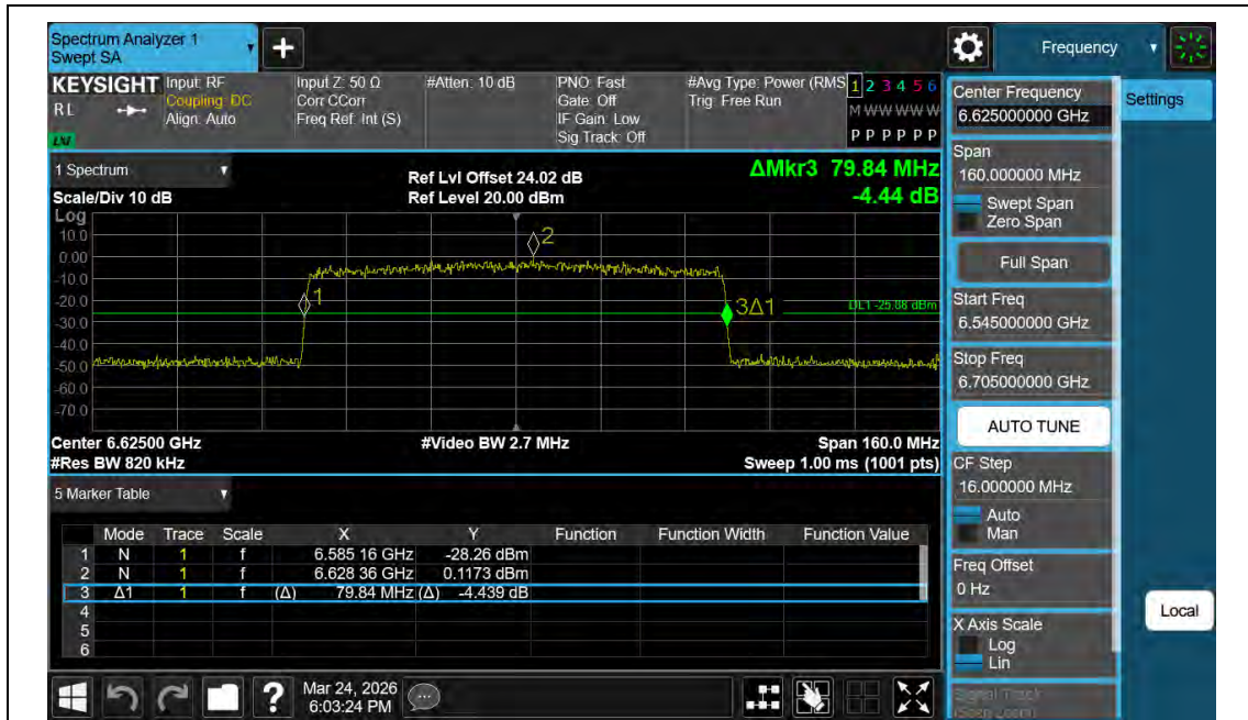
11AX80MIMO-Ant2-6625
