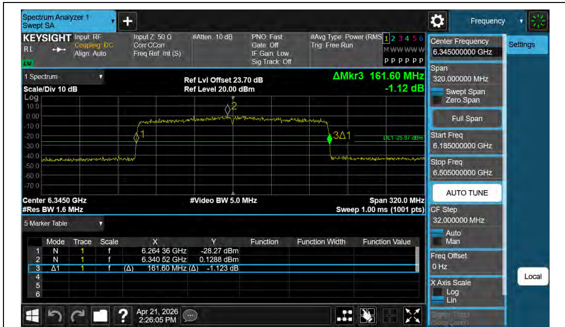
11AX160MIMO-Ant2-6345
