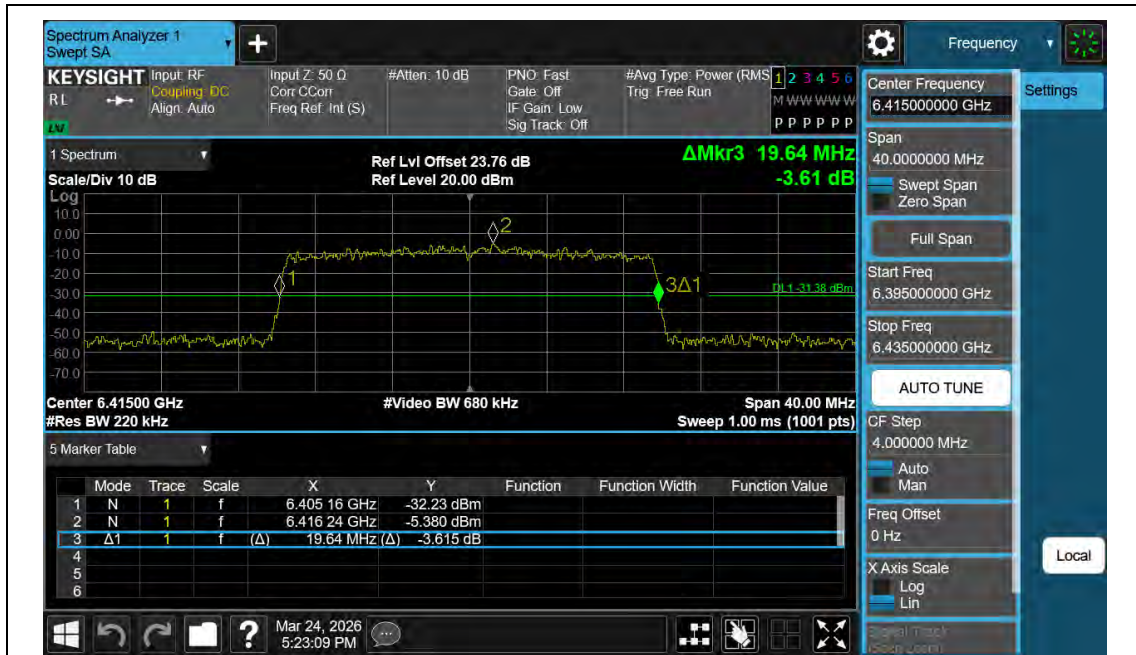
11AX20MIMO-Ant2-6415
