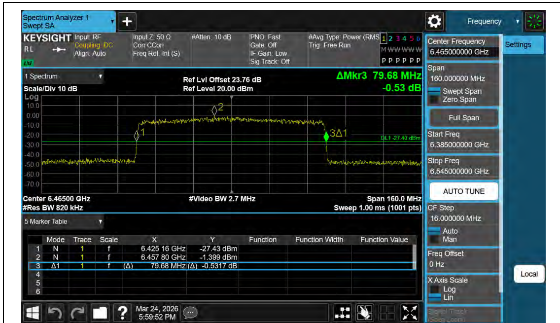
11AX80MIMO-Ant2-6465
