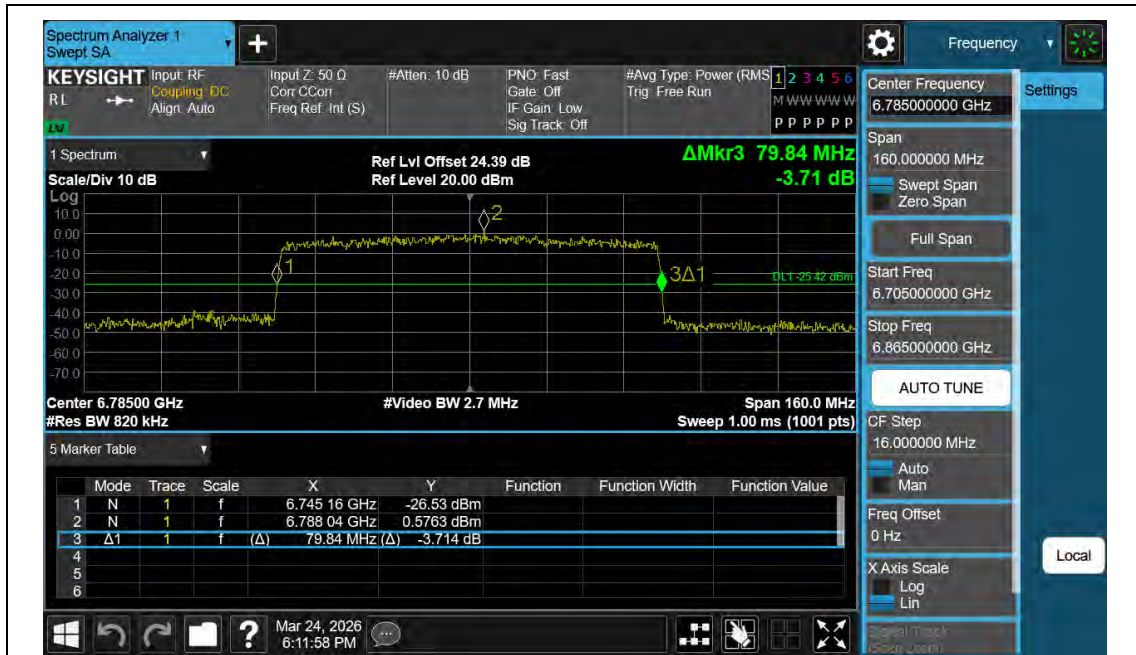
11AX80MIMO-Ant2-6785
