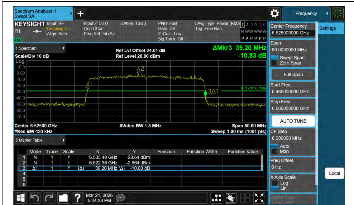
11AX40MIMO-Ant2-6525
