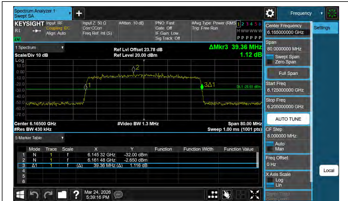
11AX40MIMO-Ant2-6165
