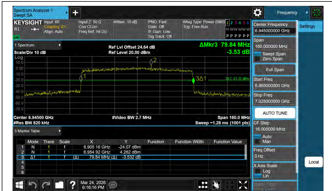
11AX80MIMO-Ant2-6945
