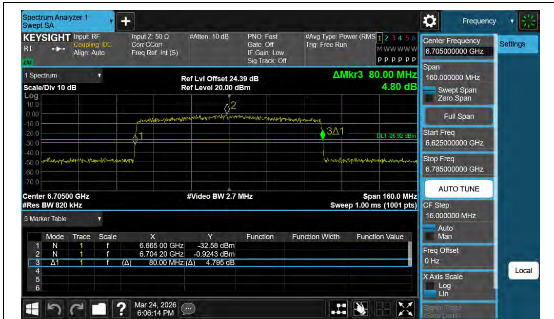
11AX80MIMO-Ant2-6705
