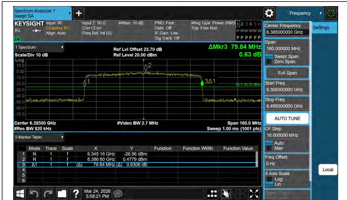
11AX80MIMO-Ant2-6385
