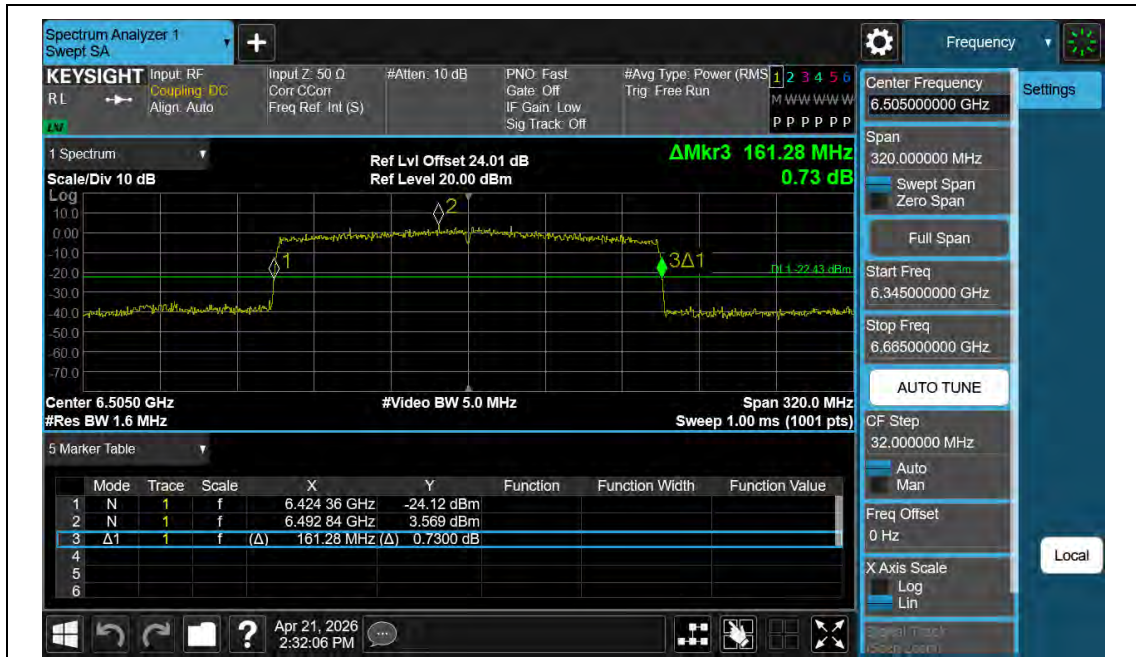
11AX160MIMO-Ant2-6505
