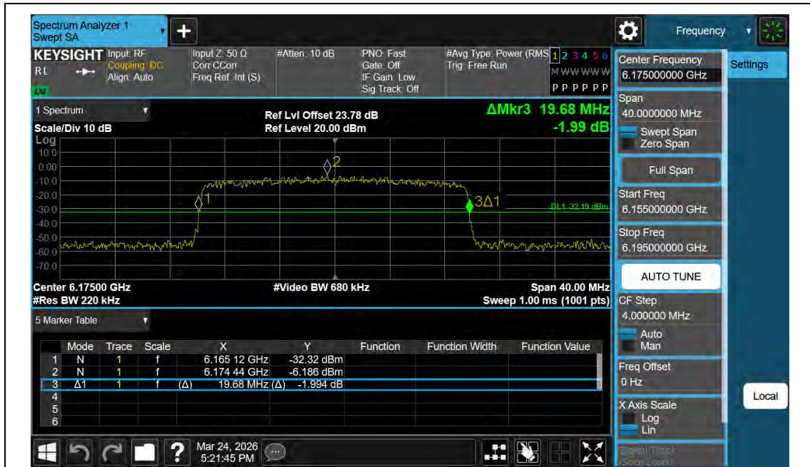
11AX20MIMO-Ant2-6175
