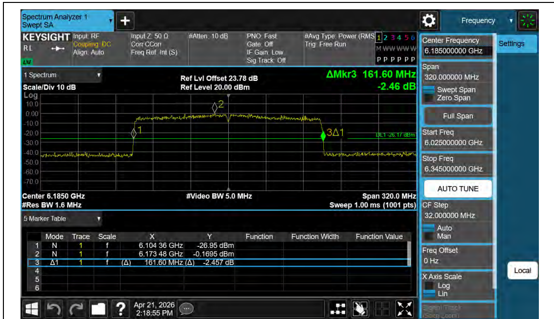
11AX160MIMO-Ant2-6185
