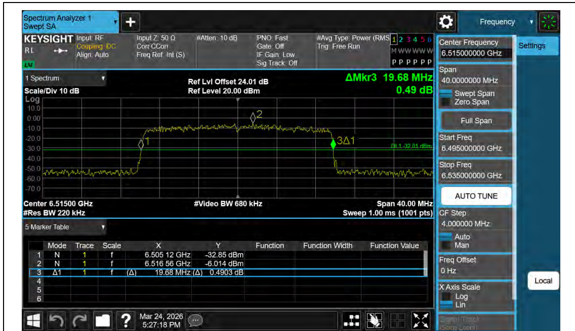
11AX20MIMO-Ant2-6515
