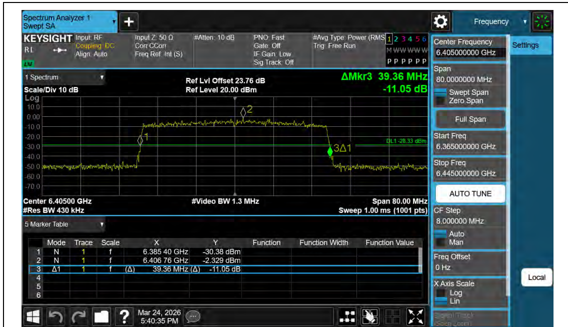
11AX40MIMO-Ant2-6405
