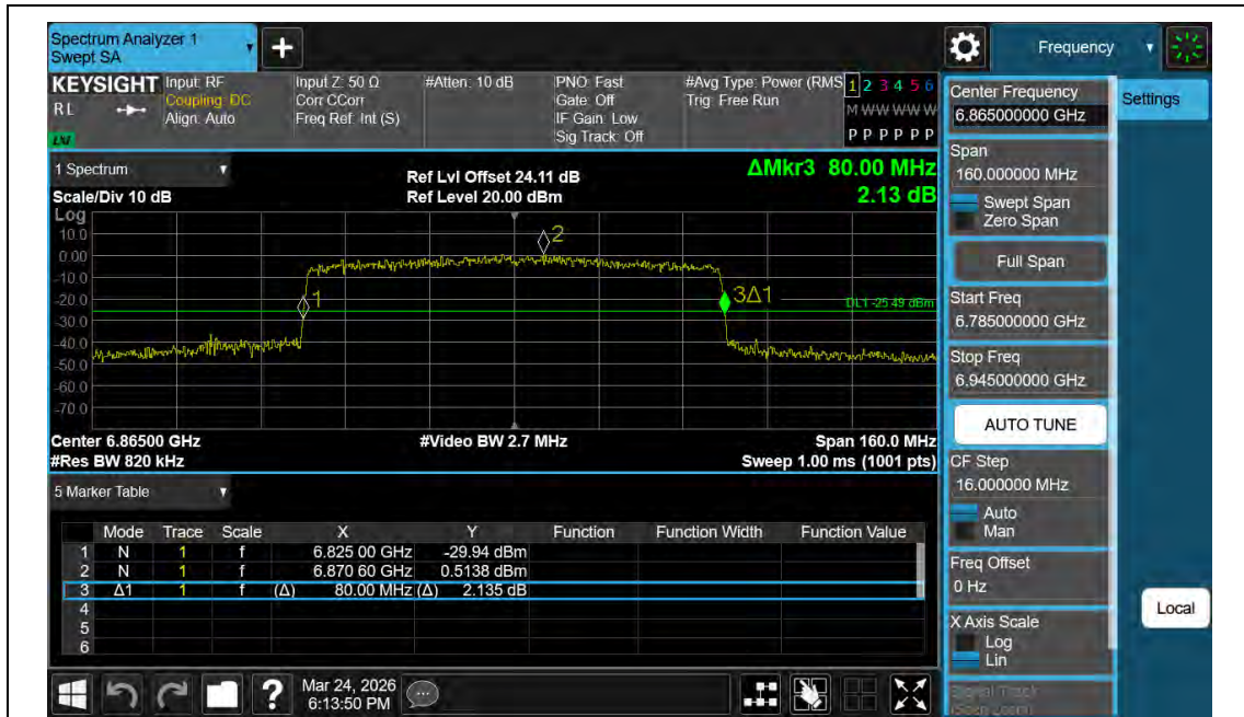
11AX80MIMO-Ant2-6865
