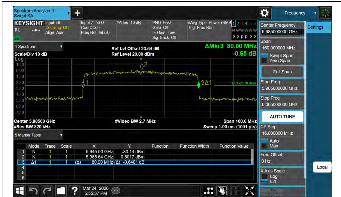
11AX80MIMO-Ant2-5985
