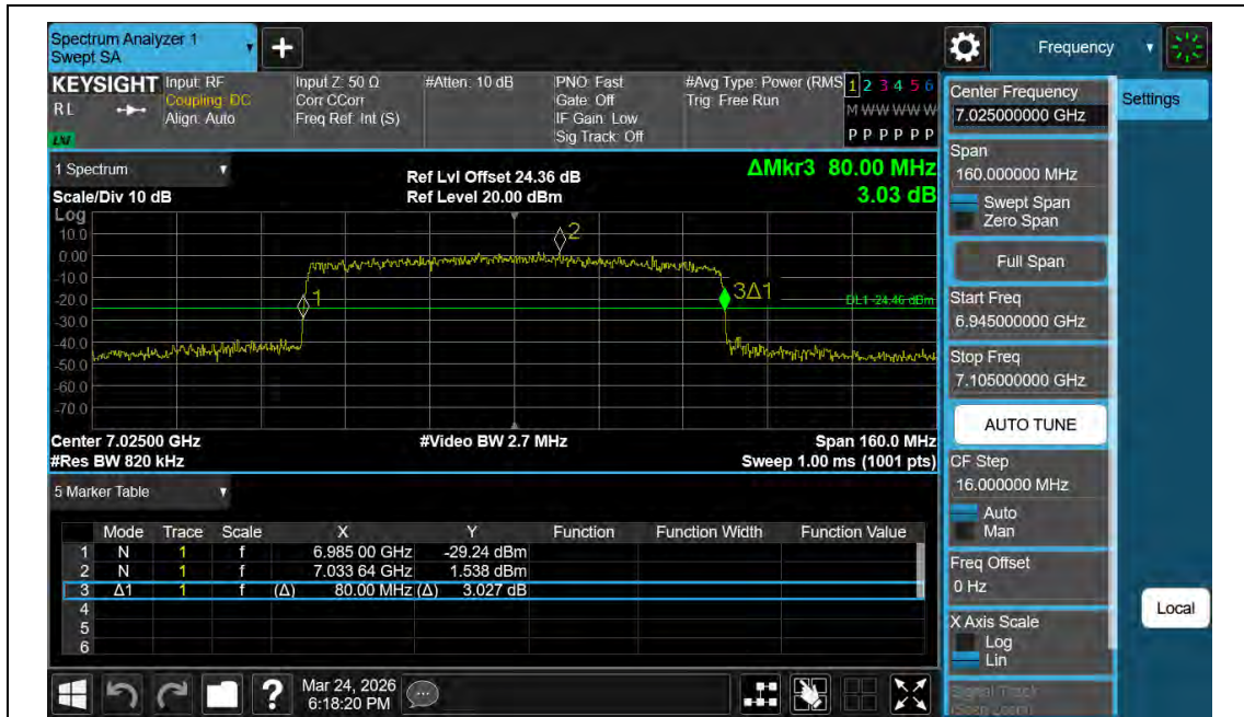
11AX80MIMO-Ant2-7025
