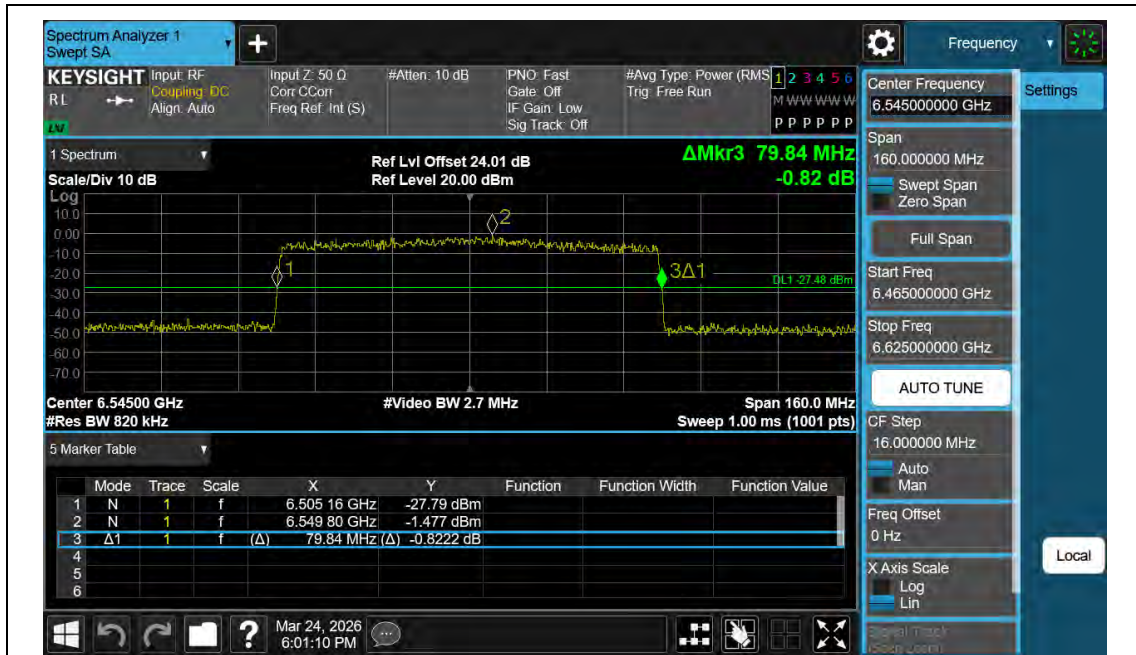
11AX80MIMO-Ant2-6545
