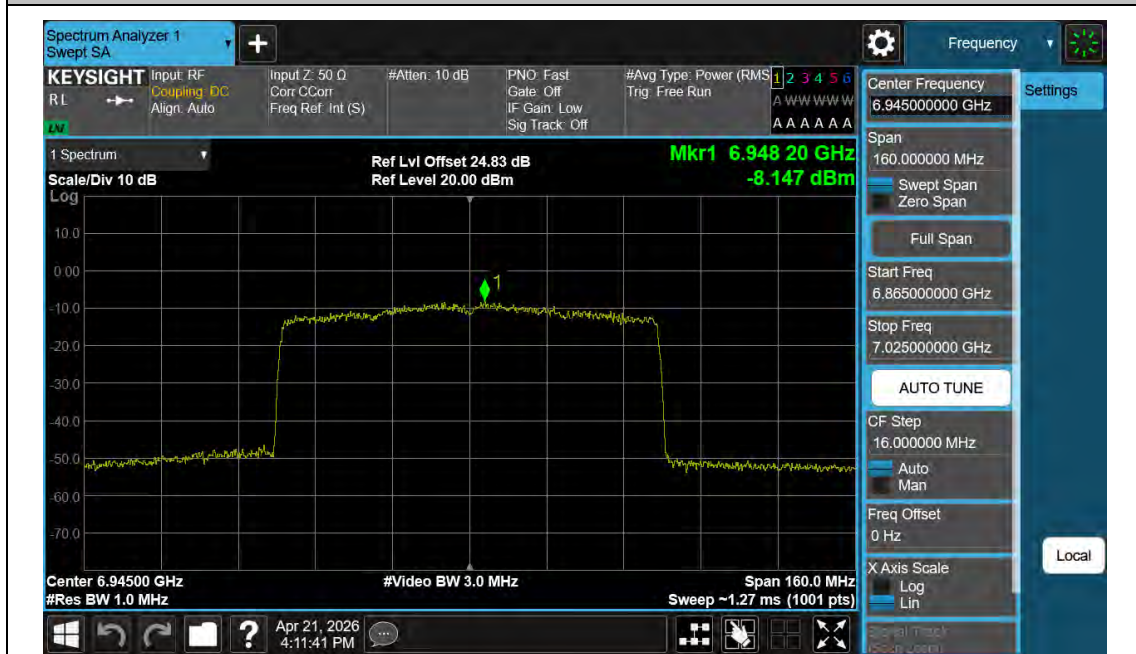
11AX80MIMO-Ant1-7025-PASS
