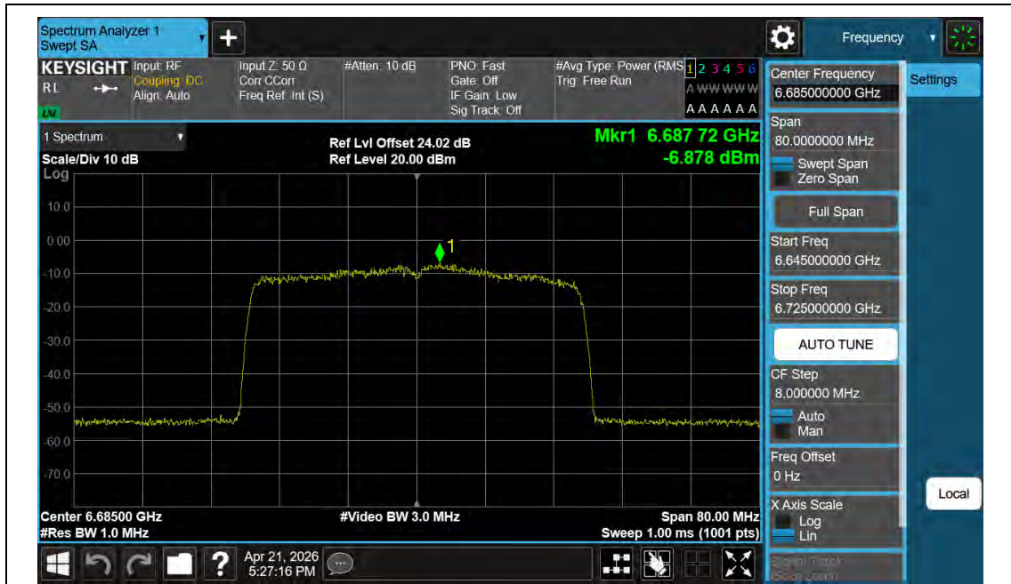
11BE40MIMO-Ant2-6685-PASS
