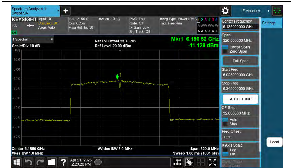
11AX160MIMO-Ant2-6185-PASS
