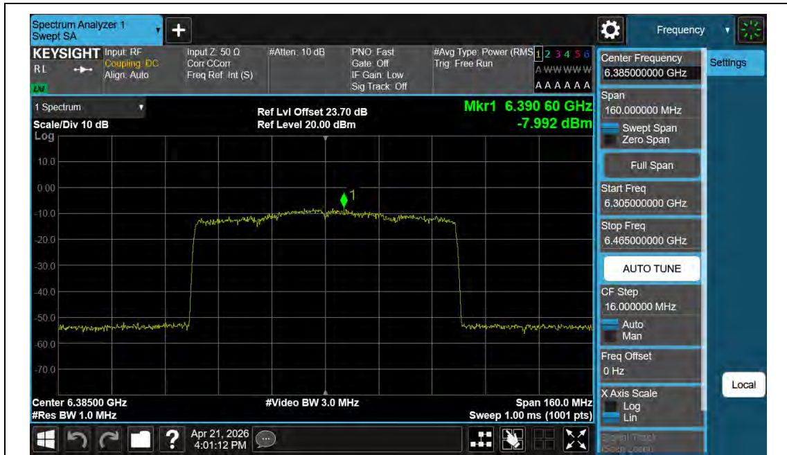
11AX80MIMO-Ant2-6385-PASS
