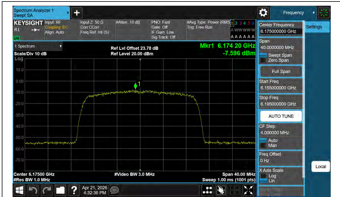
11BE20MIMO-Ant2-6175-PASS
