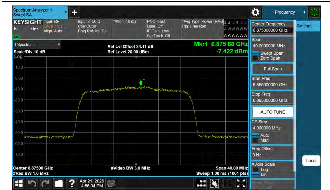
11BE20MIMO-Ant2-6875-PASS
