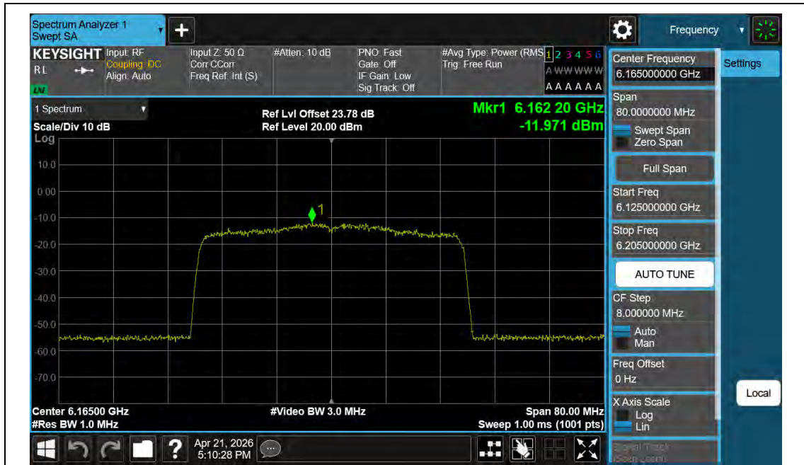
11BE40MIMO-Ant2-6165-PASS
