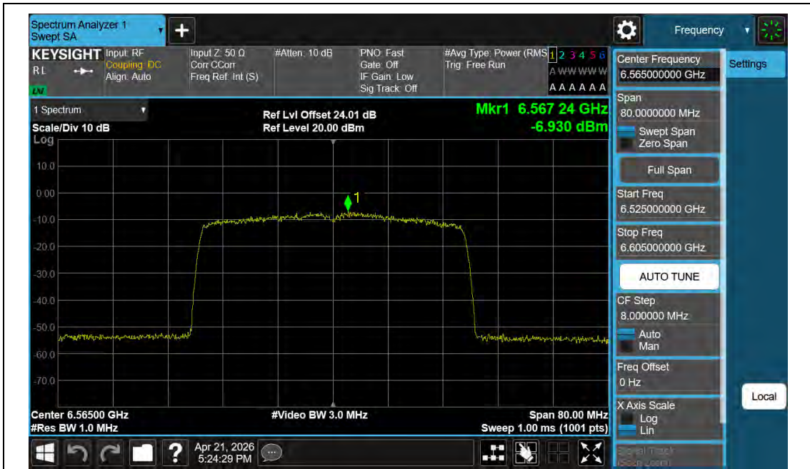
11BE40MIMO-Ant2-6565-PASS
