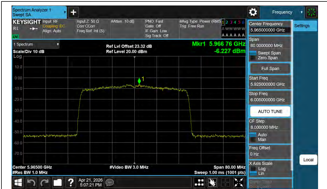
11BE40MIMO-Ant2-5965-PASS
