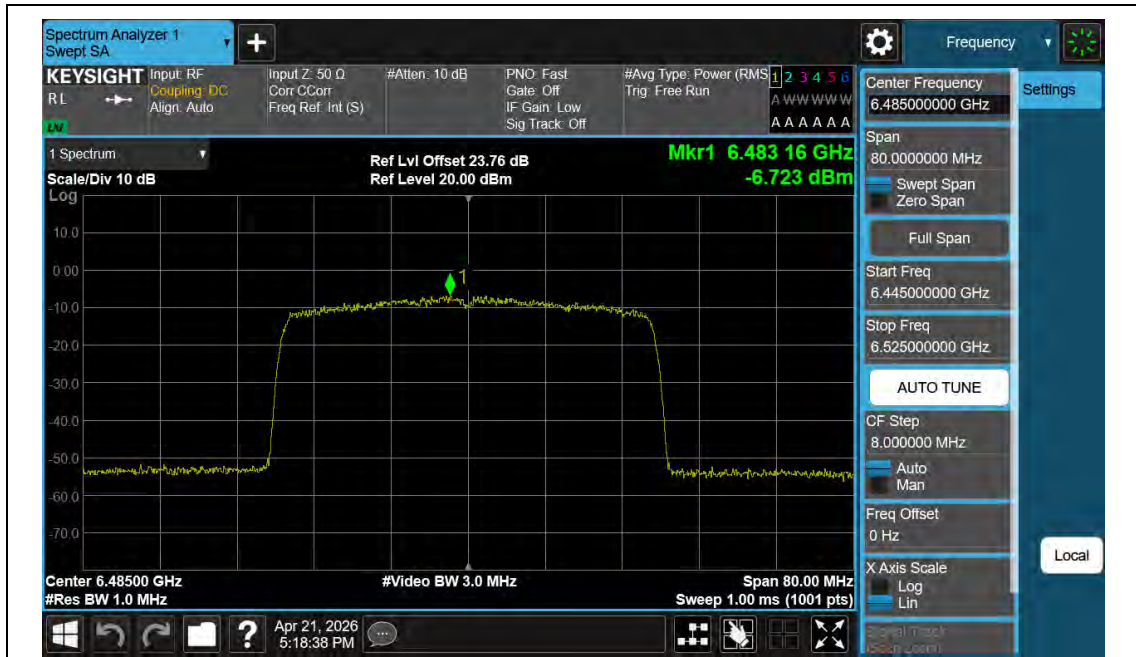
11BE40MIMO-Ant2-6485-PASS
