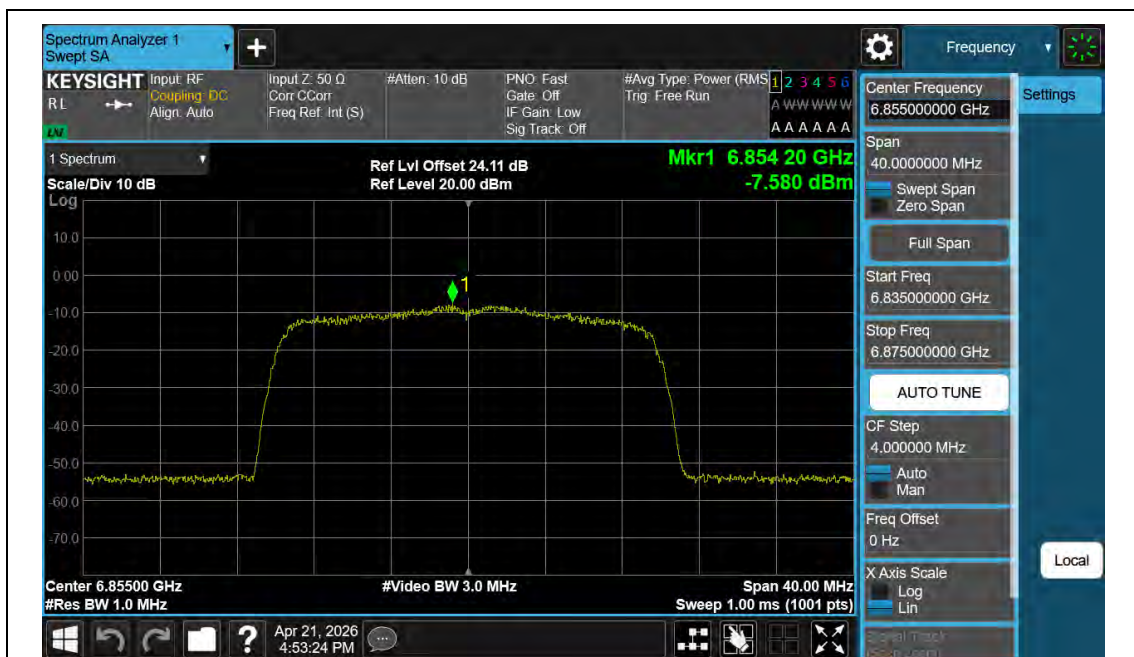
11BE20MIMO-Ant2-6855-PASS
