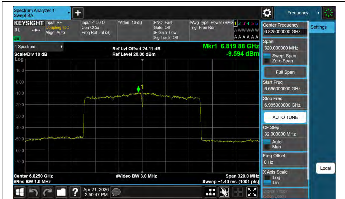
11AX160MIMO-Ant2-6825-PASS
