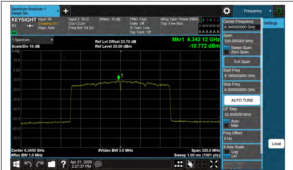
11AX160MIMO-Ant2-6345-PASS
