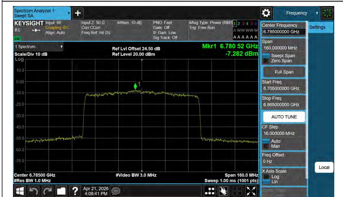
11AX80MIMO-Ant1-6865-PASS
