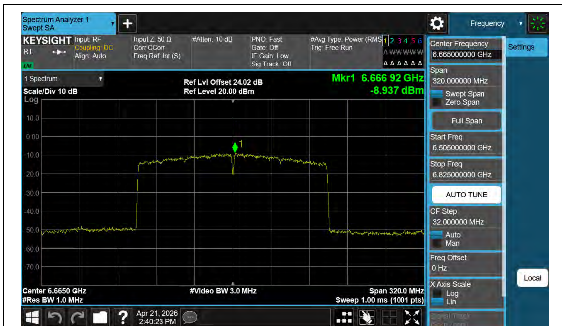
11AX160MIMO-Ant2-6665-PASS
