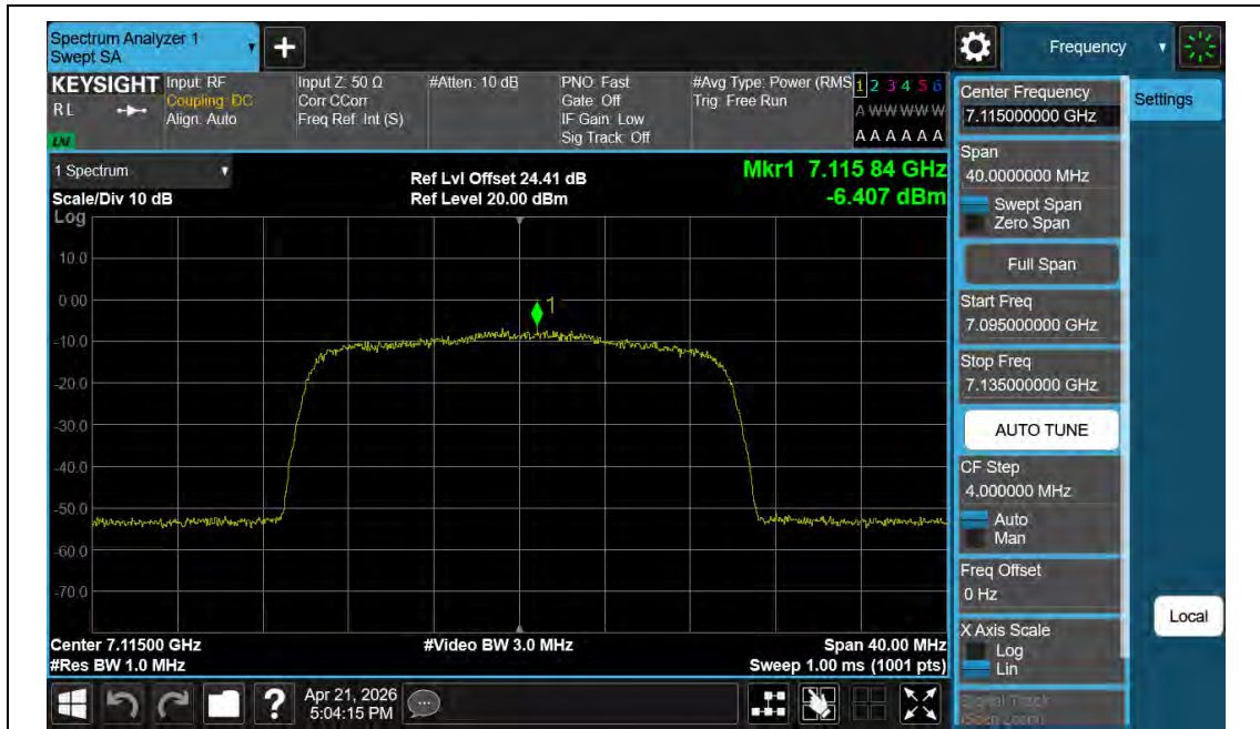
11BE20MIMO-Ant2-7115-PASS
