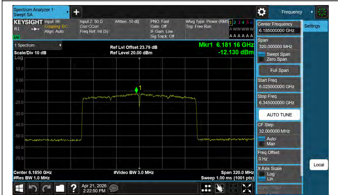
11AX160MIMO-Ant1-6345-PASS
