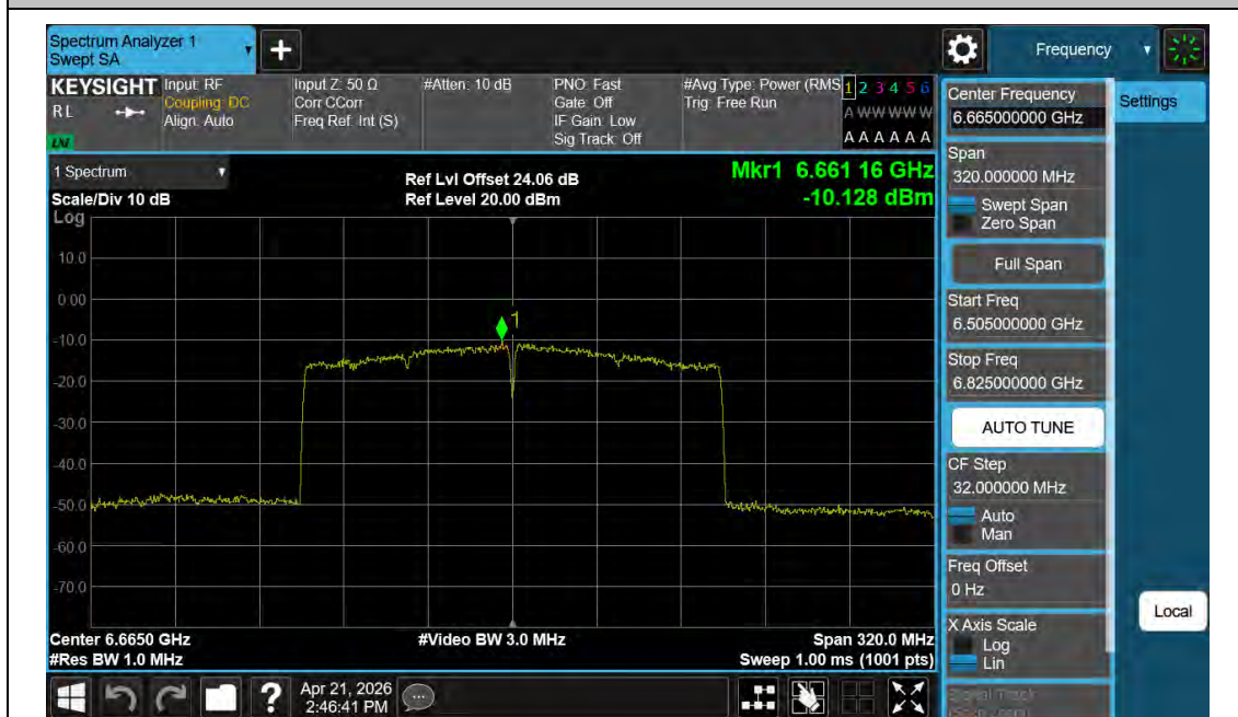
11AX160MIMO-Ant1-6825-PASS
