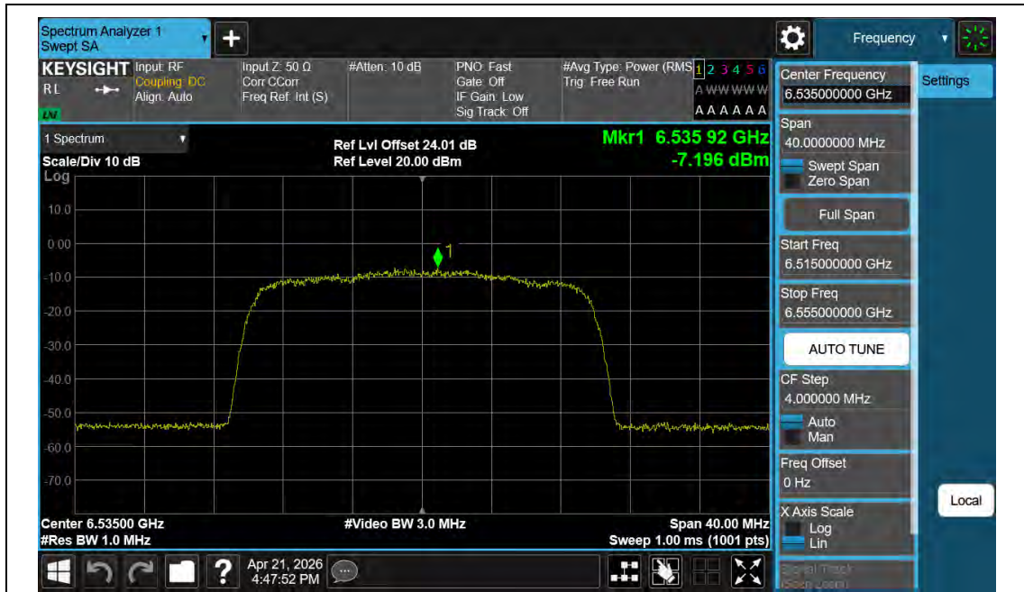
11BE20MIMO-Ant2-6535-PASS
