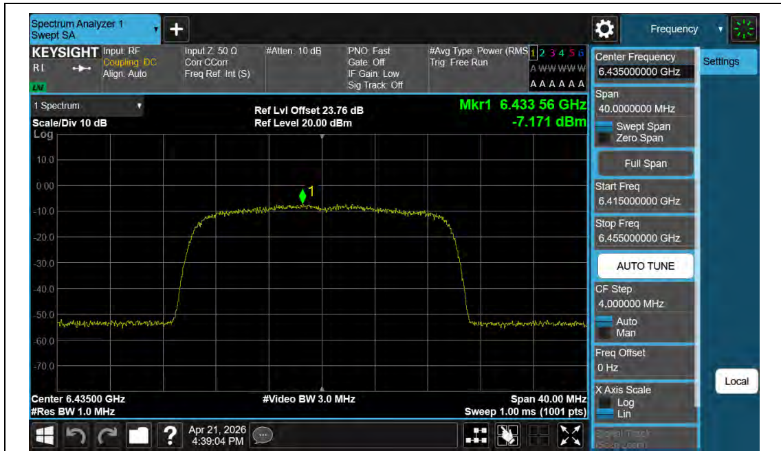
11BE20MIMO-Ant2-6435-PASS
