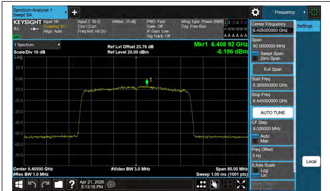
11BE40MIMO-Ant2-6405-PASS
