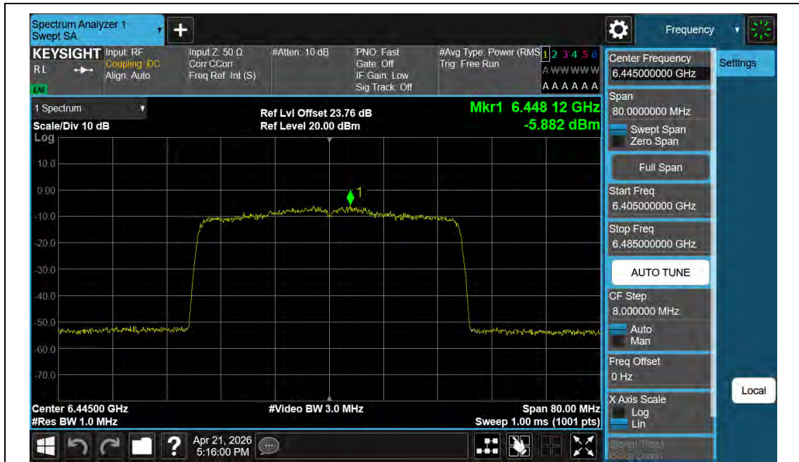
11BE40MIMO-Ant2-6445-PASS
