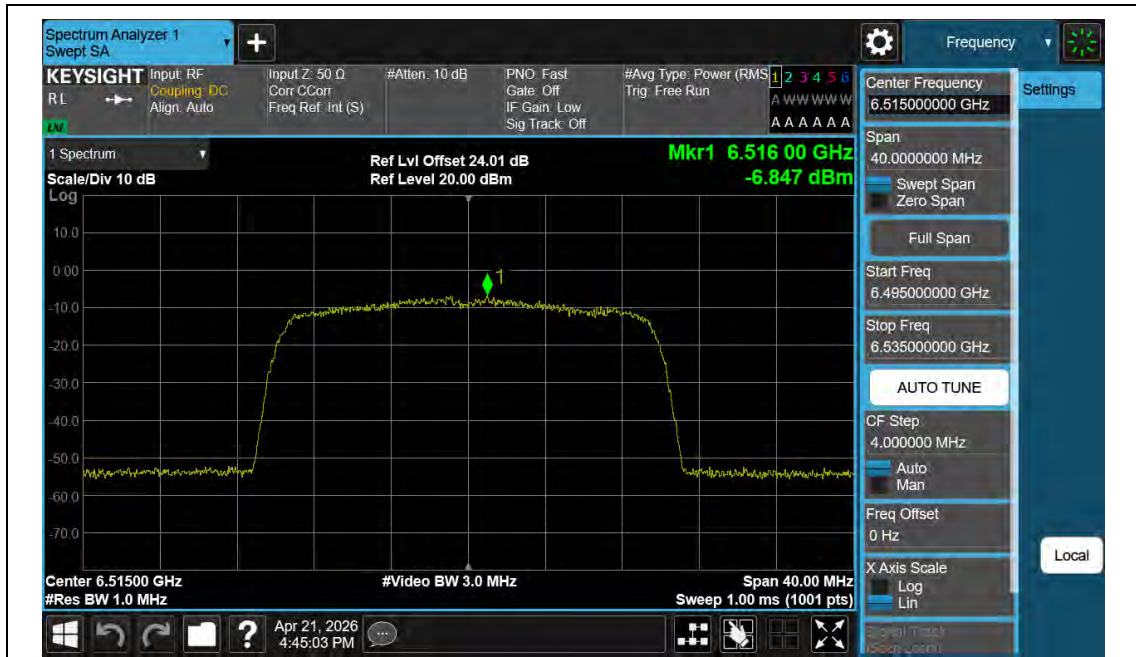
11BE20MIMO-Ant2-6515-PASS
