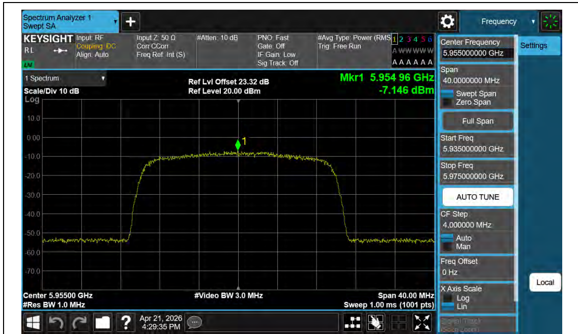
11BE20MIMO-Ant2-5955-PASS
