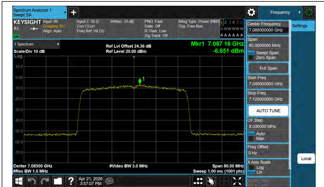
11AX40MIMO-Ant2-7085-PASS
