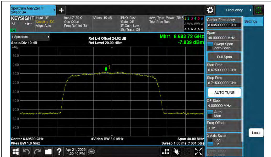
11BE20MIMO-Ant2-6695-PASS
