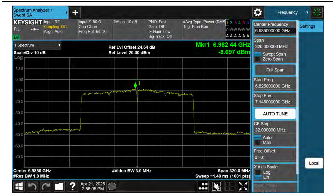
11AX160MIMO-Ant2-6985-PASS
