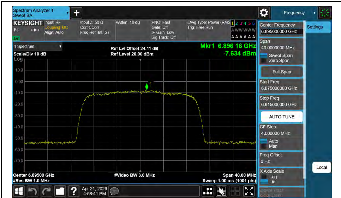
11BE20MIMO-Ant2-6895-PASS
