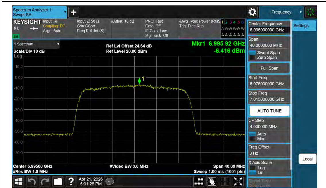
11BE20MIMO-Ant2-6995-PASS
