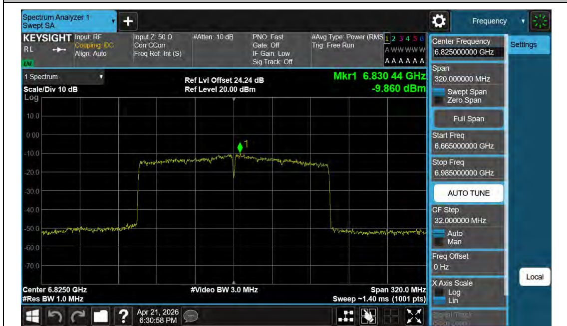
11BE160MIMO-Ant1-6985-PASS
