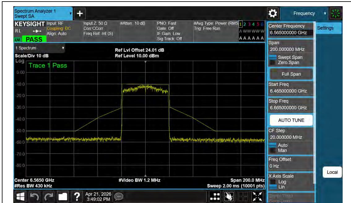
NTNV-11AX40MIMO-Ant2-6565-PASS
