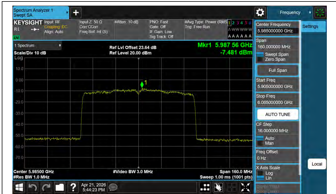
11BE80MIMO-Ant2-5985-PASS
