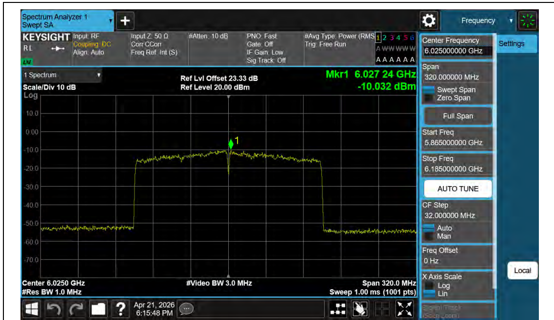
11BE160MIMO-Ant2-6025-PASS
