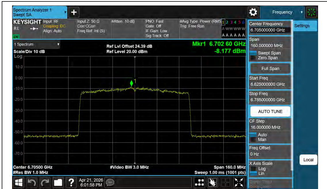
11BE80MIMO-Ant2-6705-PASS
