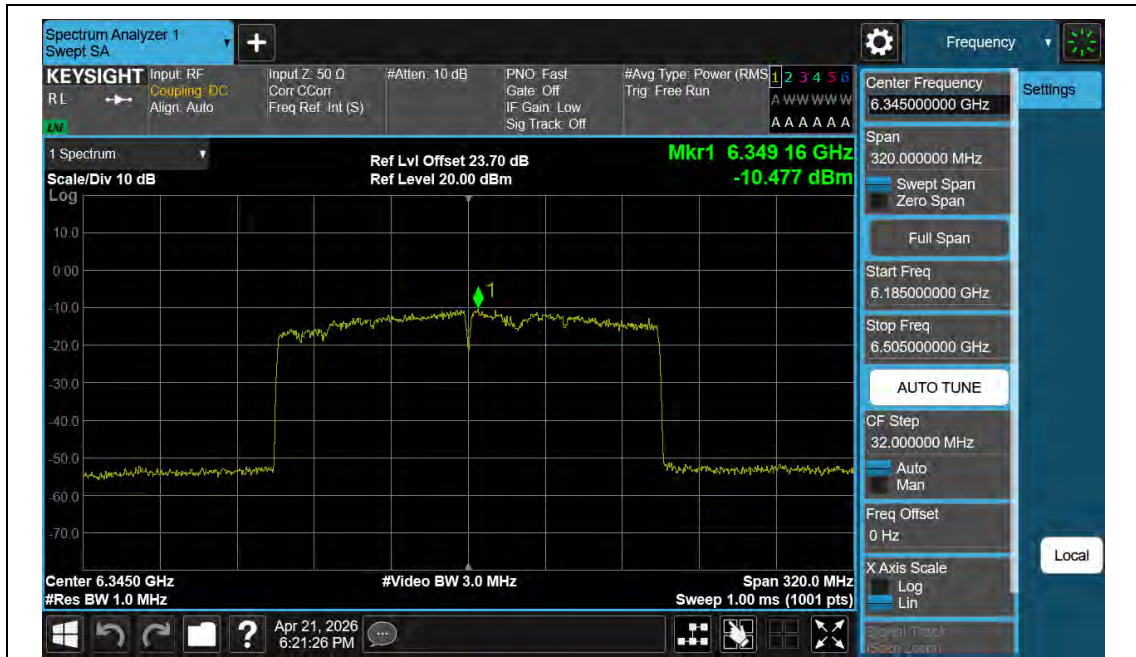
11BE160MIMO-Ant2-6345-PASS
