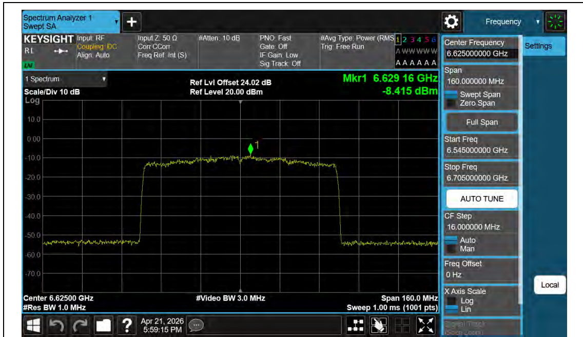
11BE80MIMO-Ant2-6625-PASS
