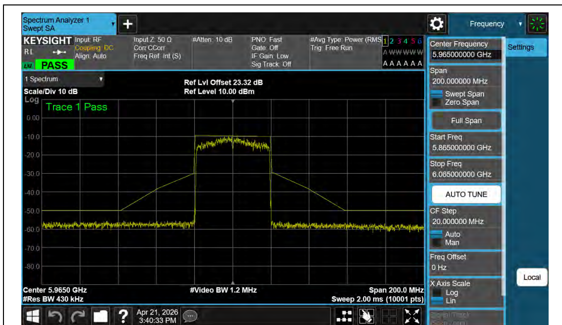
NTNV-11AX40MIMO-Ant2-5965-PASS
