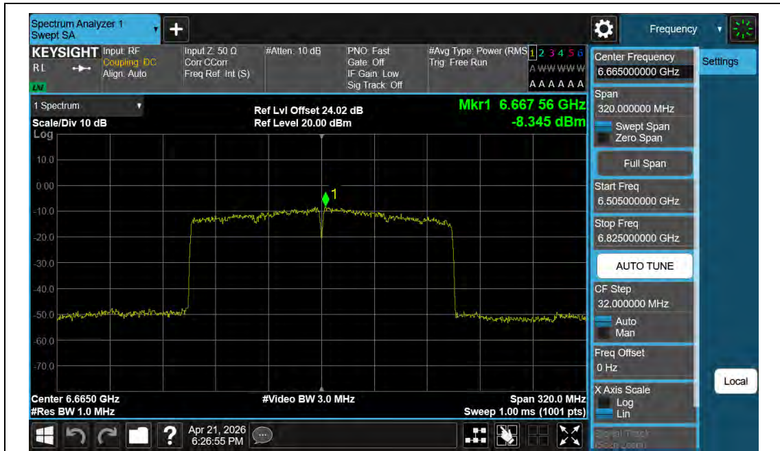
11BE160MIMO-Ant2-6665-PASS
