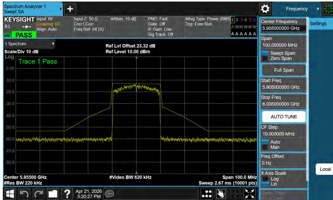
NTNV-11AX20MIMO-Ant2-5955-PASS
