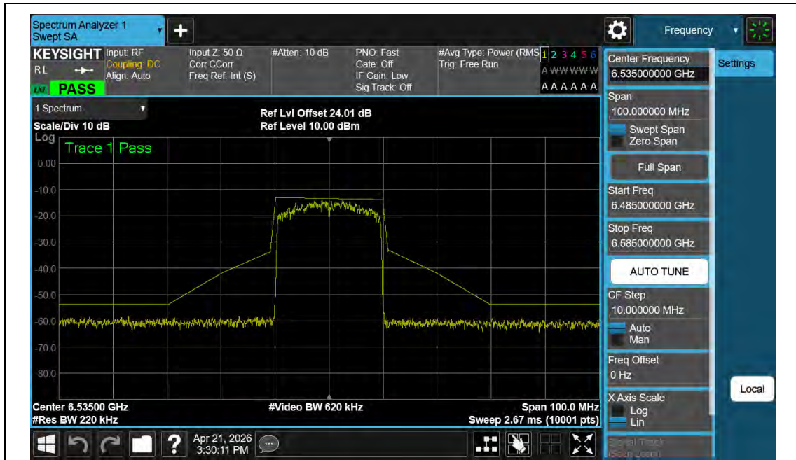
NTNV-11AX20MIMO-Ant2-6535-PASS
