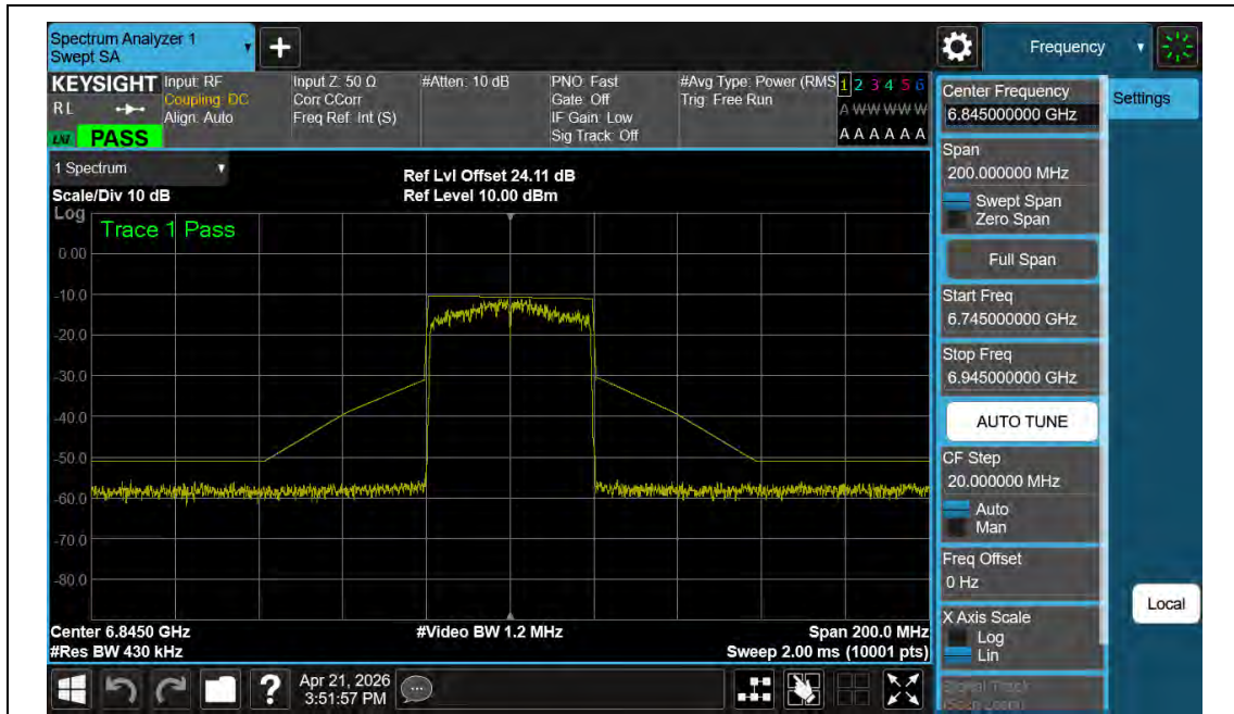
NTNV-11AX40MIMO-Ant2-6845-PASS
