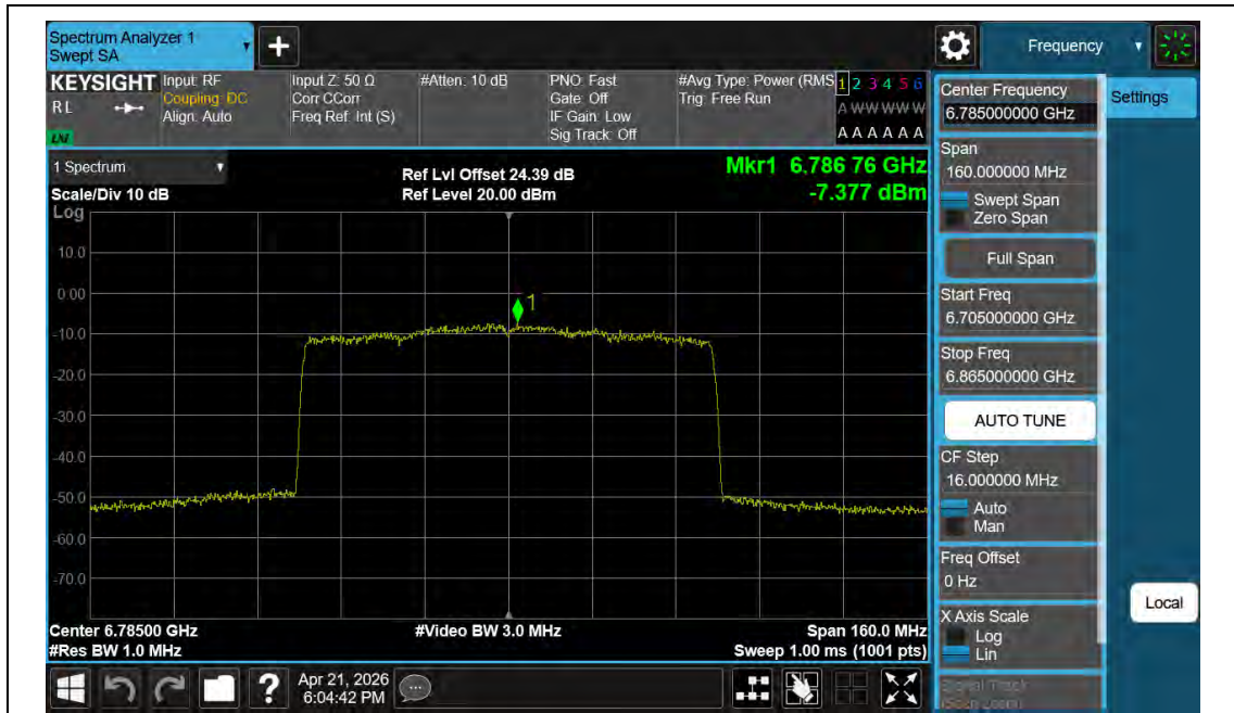
11BE80MIMO-Ant2-6785-PASS
