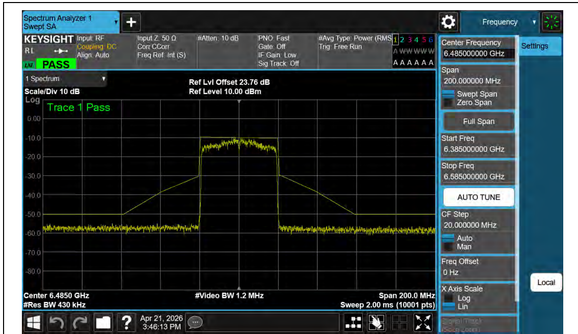
NTNV-11AX40MIMO-Ant2-6485-PASS
