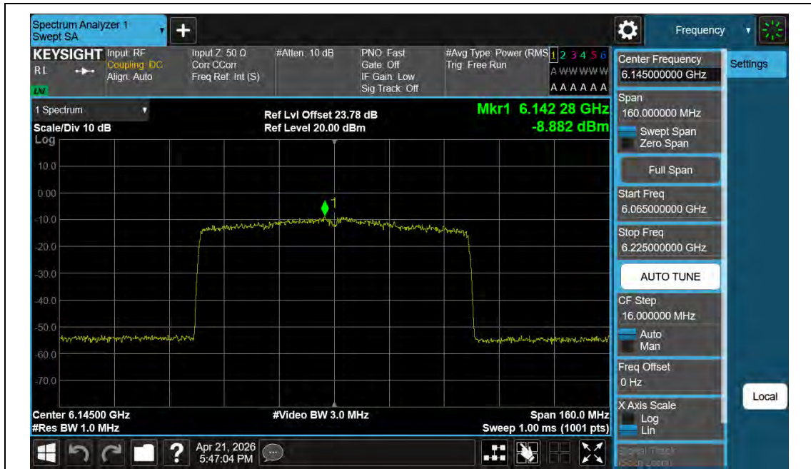
11BE80MIMO-Ant2-6145-PASS
