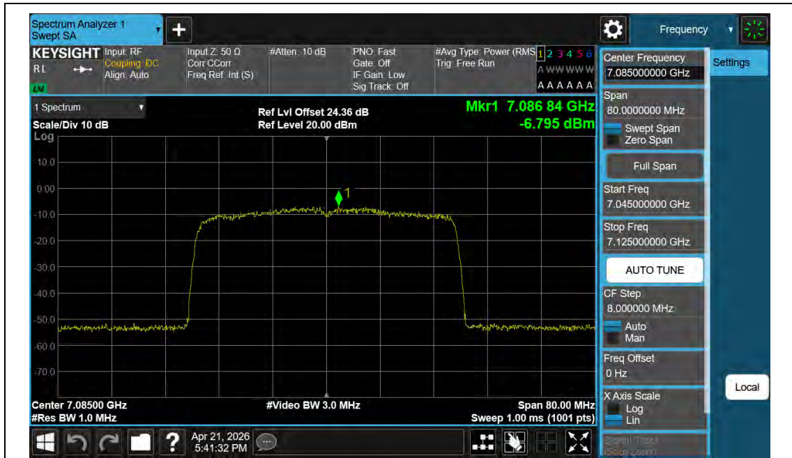
11BE40MIMO-Ant2-7085-PASS
