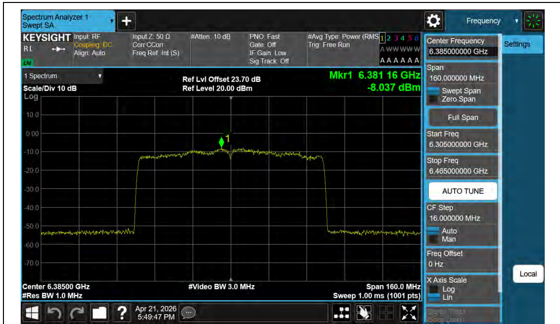
11BE80MIMO-Ant2-6385-PASS
