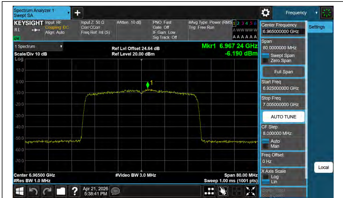
11BE40MIMO-Ant2-6965-PASS
