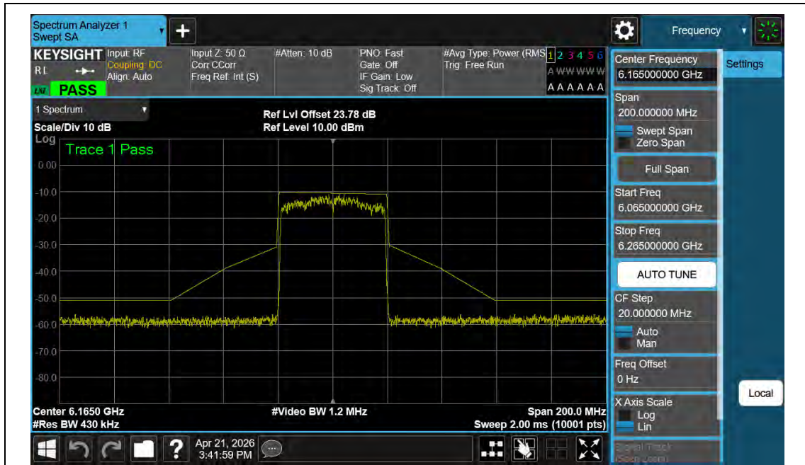
NTNV-11AX40MIMO-Ant2-6165-PASS
