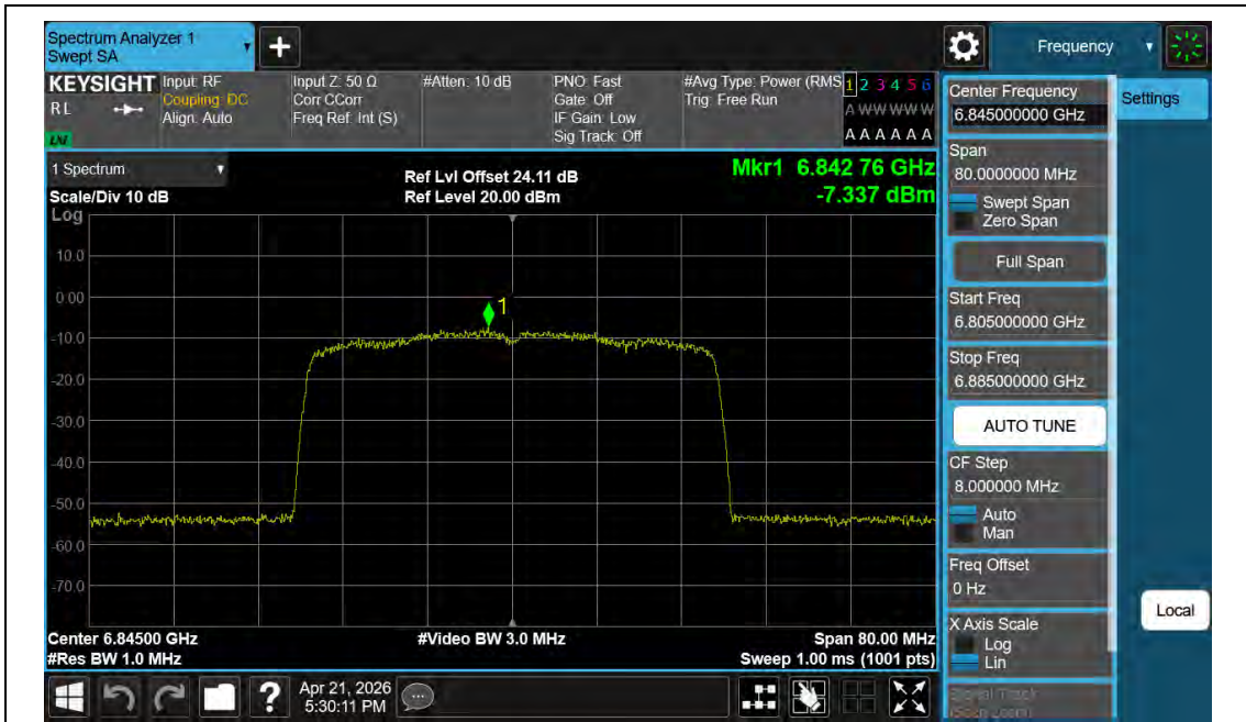
11BE40MIMO-Ant2-6845-PASS
