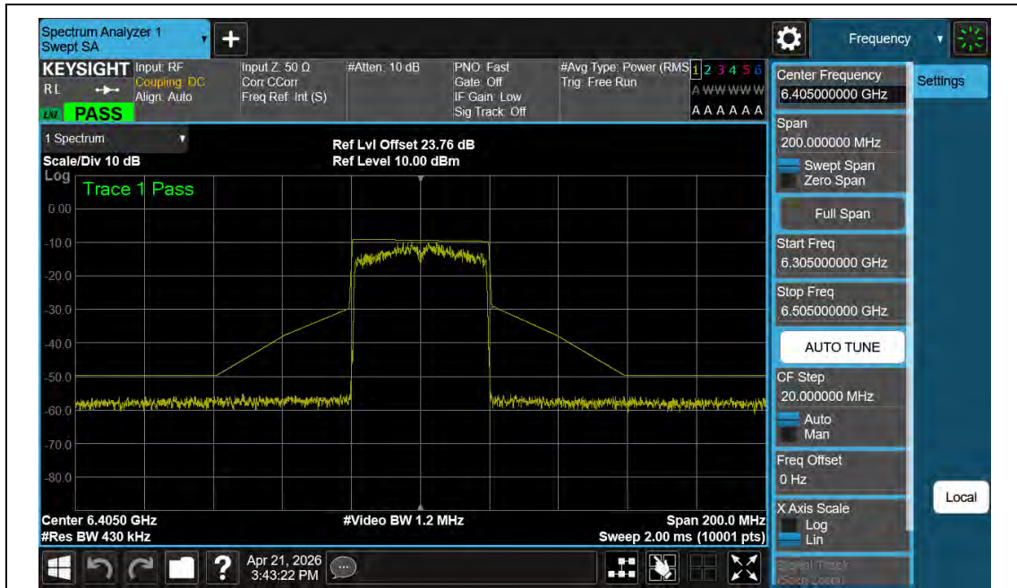
NTNV-11AX40MIMO-Ant2-6405-PASS
