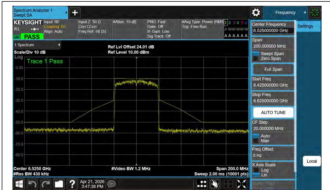
NTNV-11AX40MIMO-Ant2-6525-PASS
