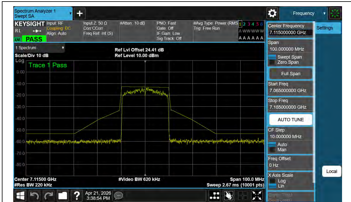
NTNV-11AX20MIMO-Ant2-7115-PASS
