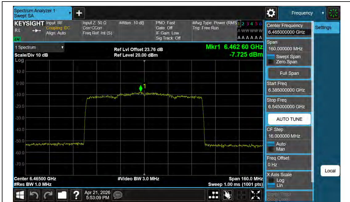
11BE80MIMO-Ant2-6465-PASS
