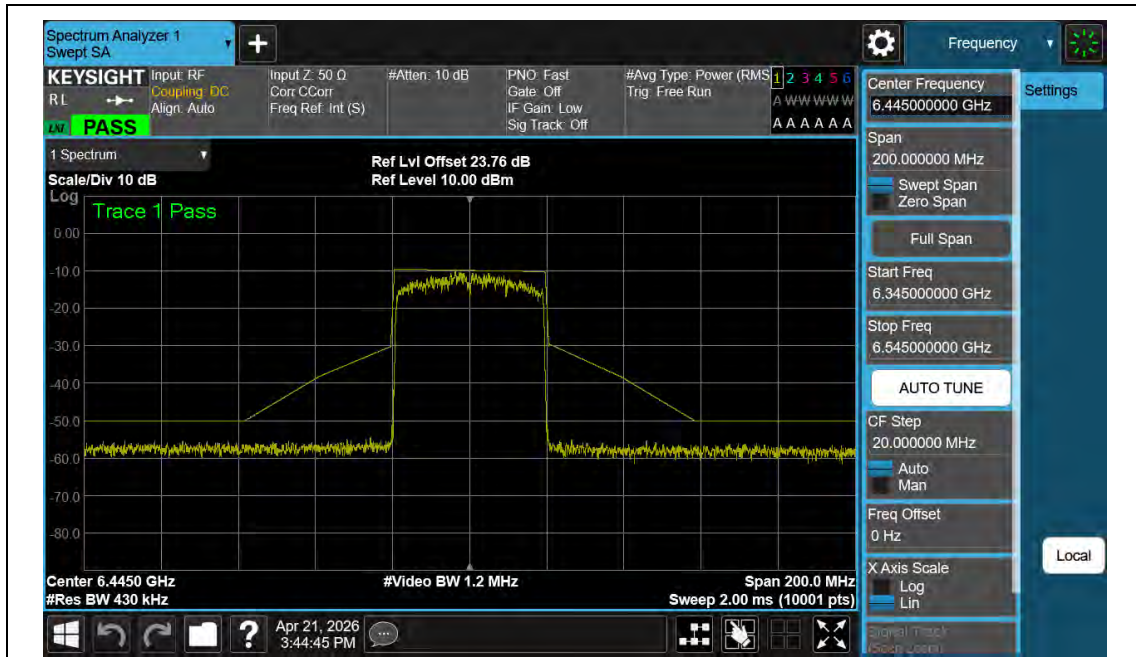
NTNV-11AX40MIMO-Ant2-6445-PASS
