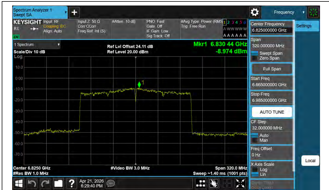
11BE160MIMO-Ant2-6825-PASS
