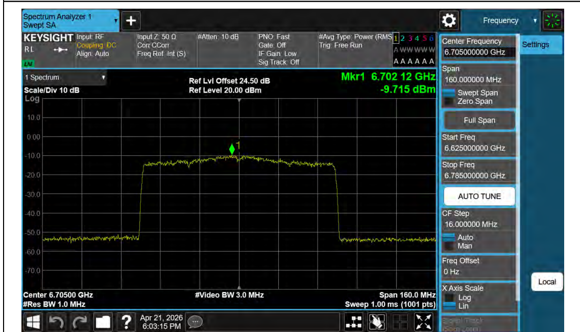
11BE80MIMO-Ant1-6785-PASS
