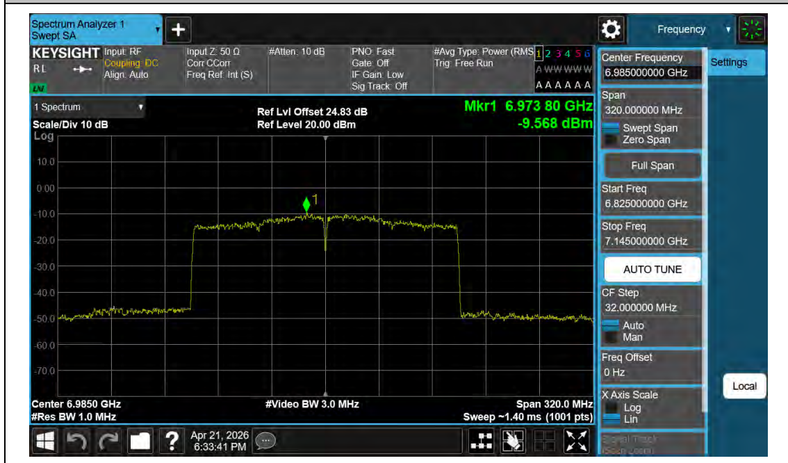
11BE160MIMO-Ant2-6985-PASS
