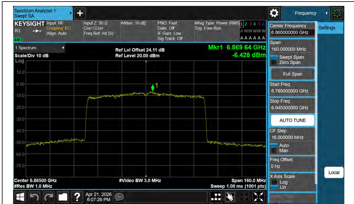
11BE80MIMO-Ant2-6865-PASS
