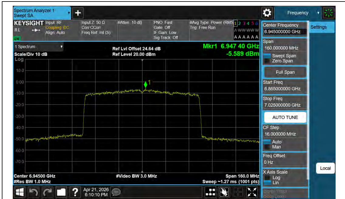
11BE80MIMO-Ant2-6945-PASS
