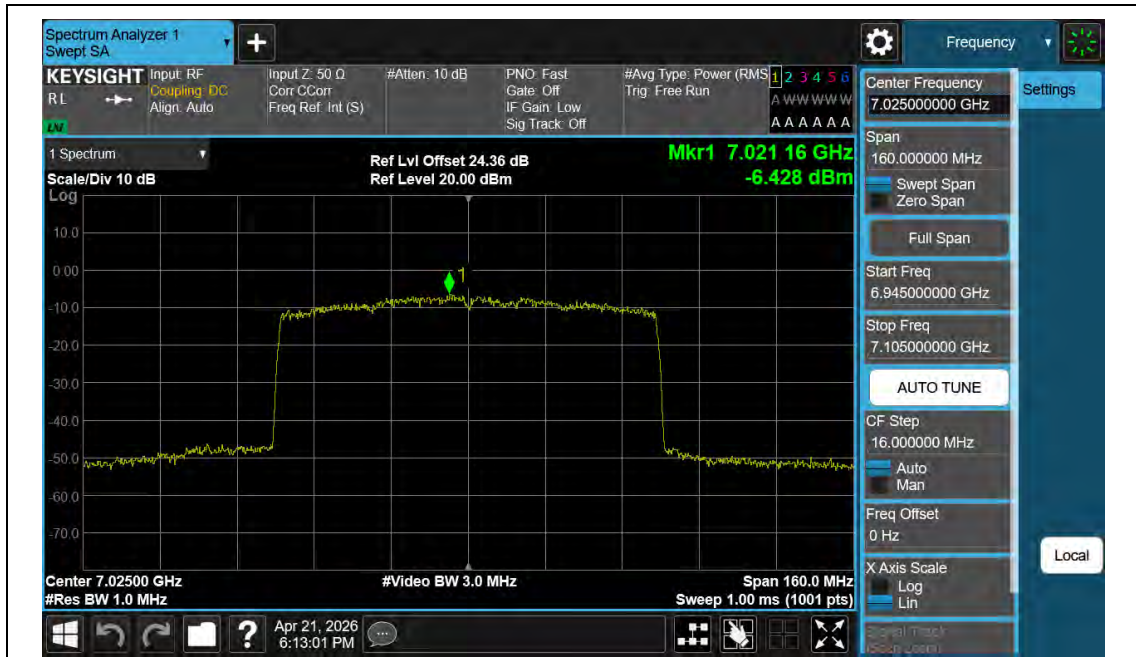
11BE80MIMO-Ant2-7025-PASS
