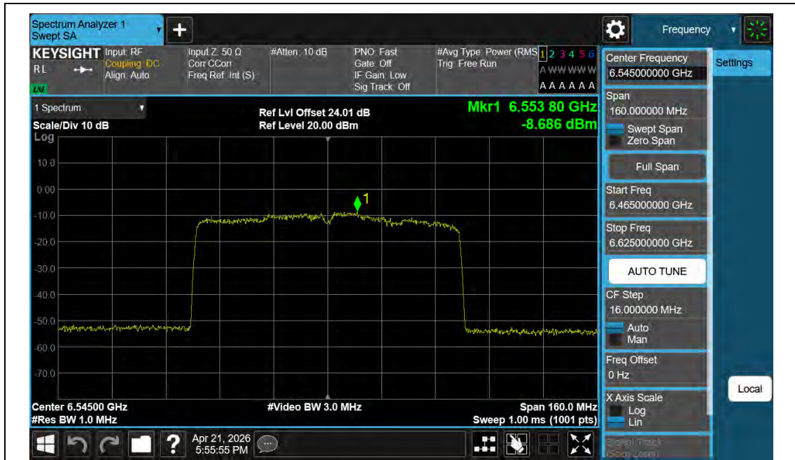
11BE80MIMO-Ant2-6545-PASS
