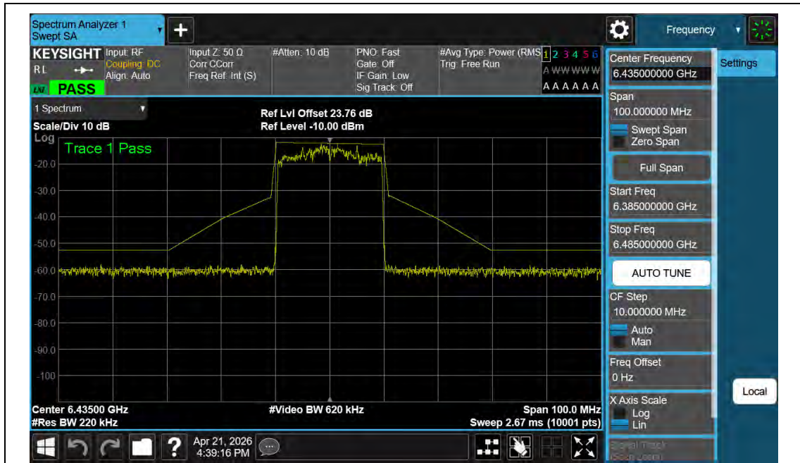
NTNV-11BE20MIMO-Ant2-6435-PASS
