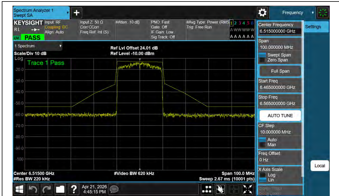
NTNV-11BE20MIMO-Ant2-6515-PASS
