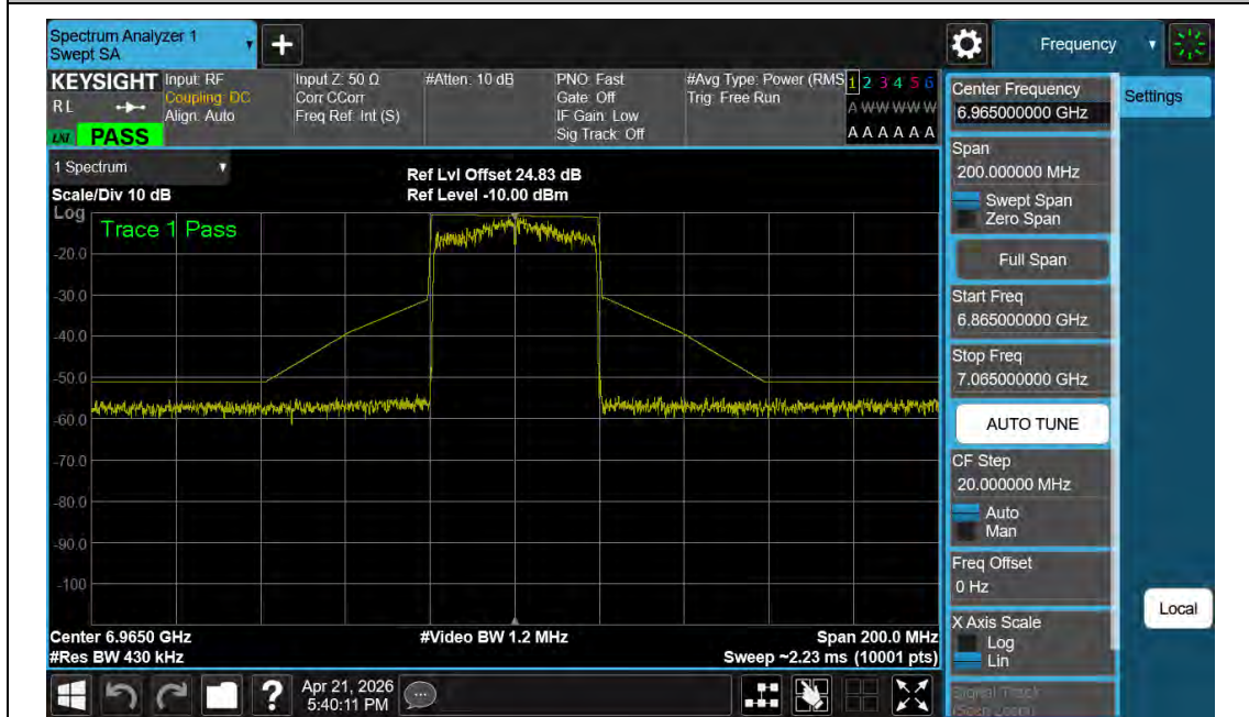
NTNV-11BE40MIMO-Ant1-7085-PASS
