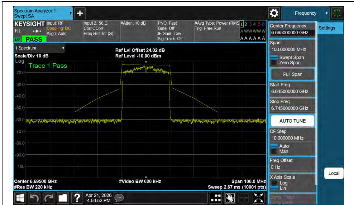
NTNV-11BE20MIMO-Ant2-6695-PASS
