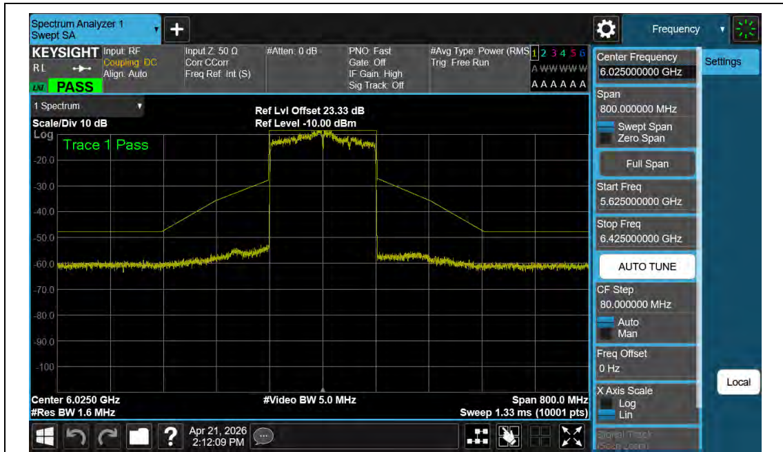
NTNV-11AX160MIMO-Ant2-6025-PASS
