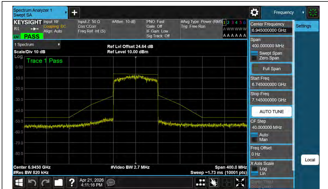
NTNV-11AX80MIMO-Ant2-6945-PASS
