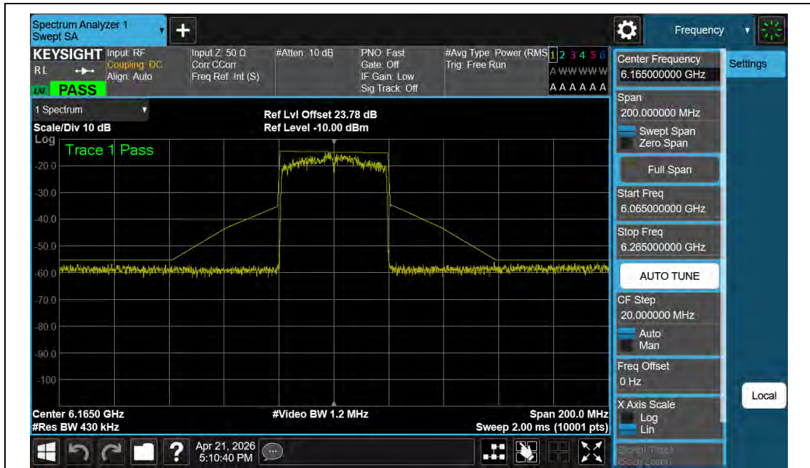
NTNV-11BE40MIMO-Ant2-6165-PASS
