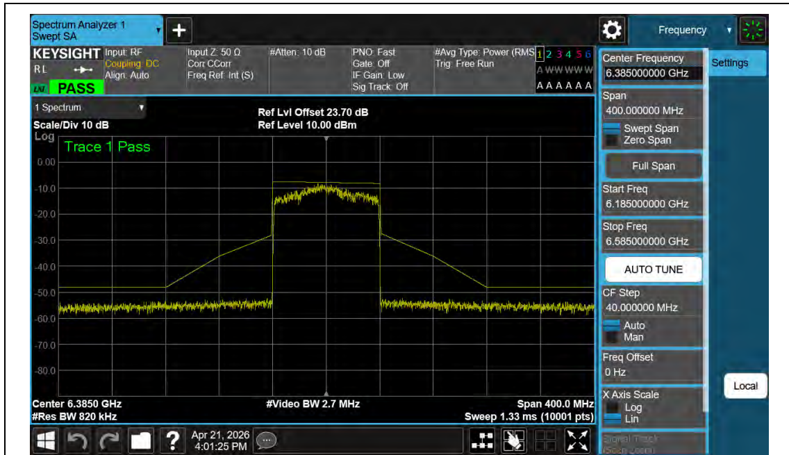
NTNV-11AX80MIMO-Ant2-6385-PASS
