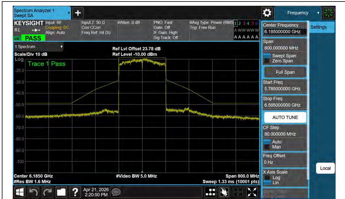
NTNV-11AX160MIMO-Ant2-6185-PASS
