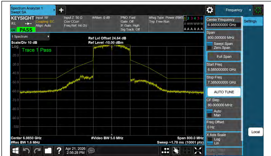
NTNV-11AX160MIMO-Ant2-6985-PASS
