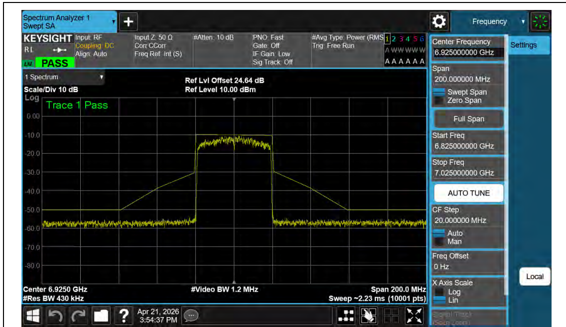
NTNV-11AX40MIMO-Ant2-6925-PASS
