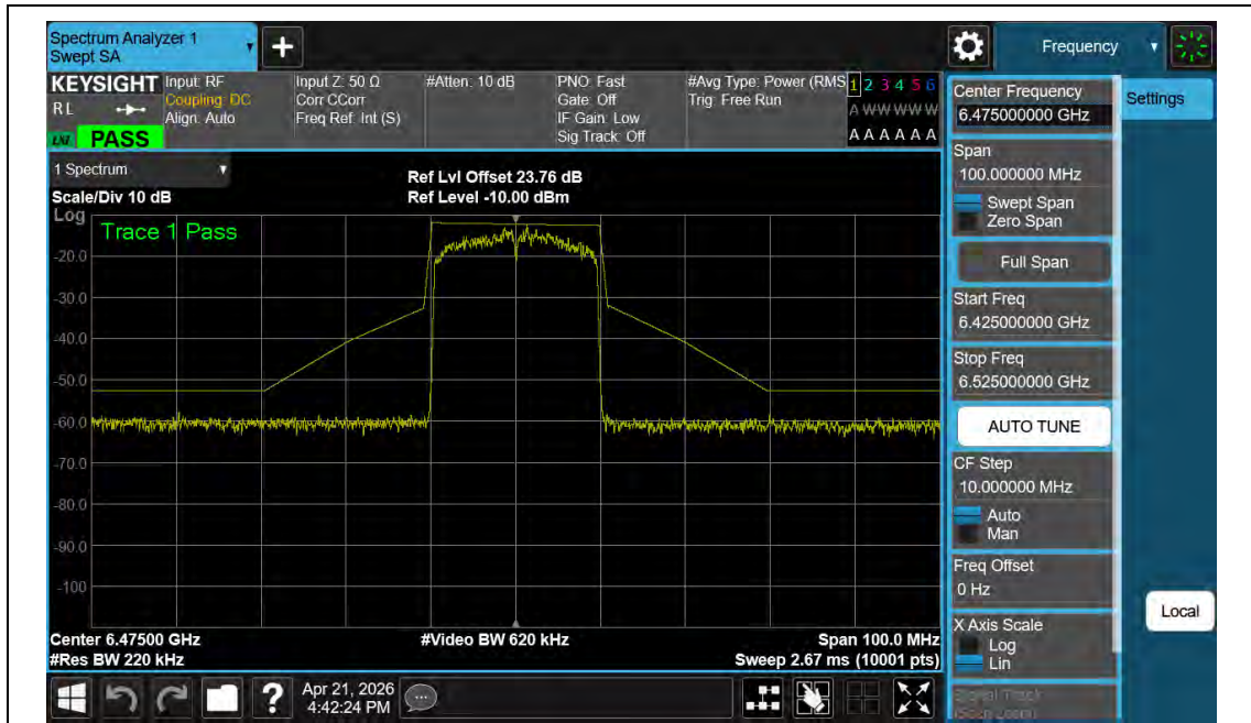
NTNV-11BE20MIMO-Ant2-6475-PASS
