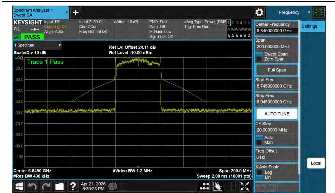
NTNV-11BE40MIMO-Ant2-6845-PASS
