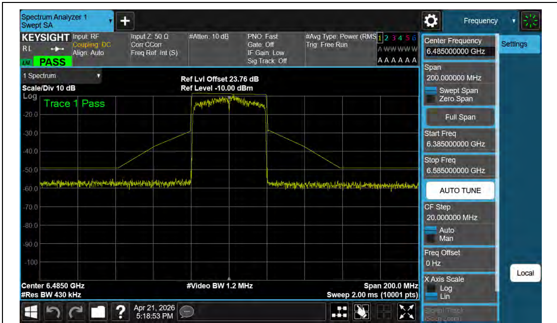
NTNV-11BE40MIMO-Ant2-6485-PASS
