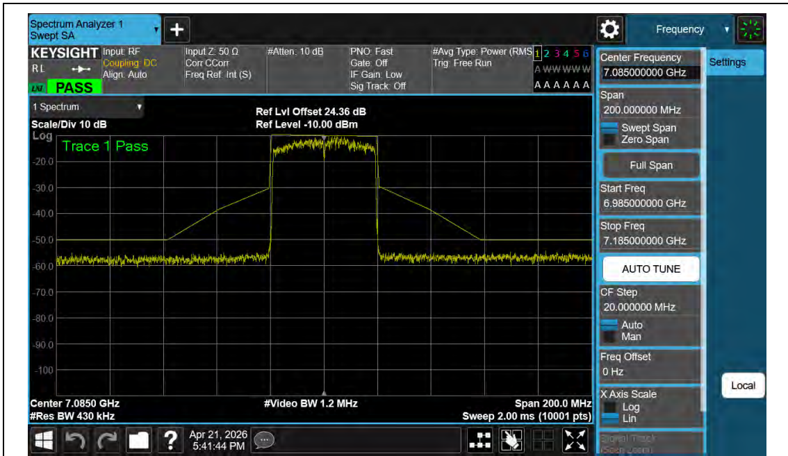
NTNV-11BE40MIMO-Ant2-7085-PASS
