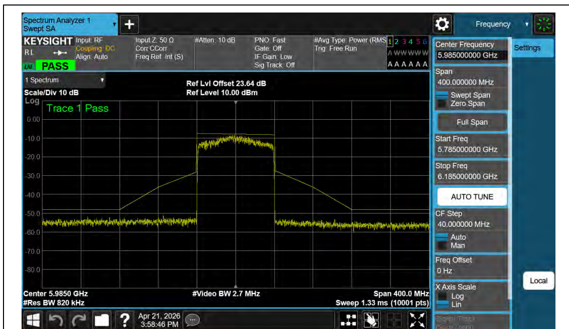
NTNV-11AX80MIMO-Ant2-5985-PASS
