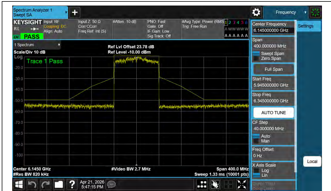
NTNV-11BE80MIMO-Ant2-6145-PASS
