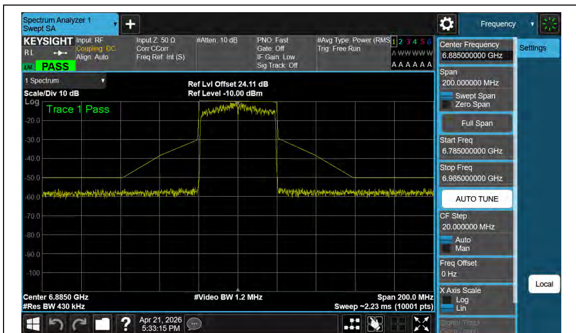
NTNV-11BE40MIMO-Ant2-6885-PASS
