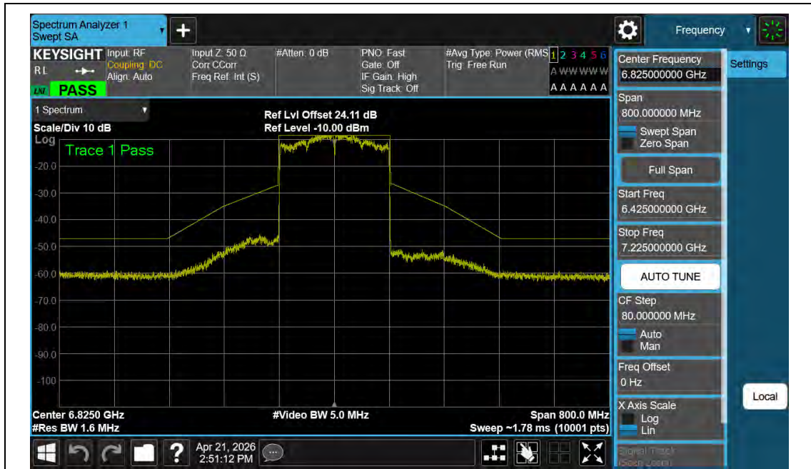
NTNV-11AX160MIMO-Ant2-6825-PASS
