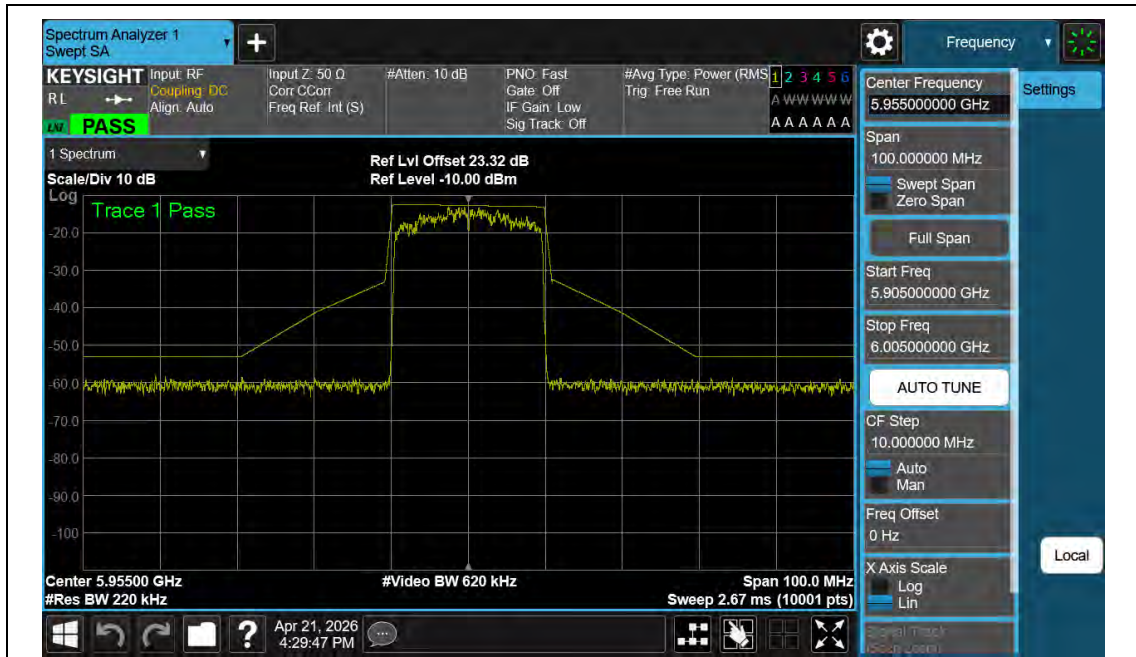
NTNV-11BE20MIMO-Ant2-5955-PASS
