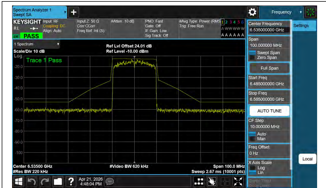
NTNV-11BE20MIMO-Ant2-6535-PASS
