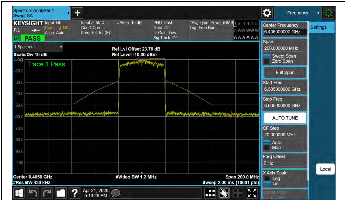
NTNV-11BE40MIMO-Ant2-6405-PASS
