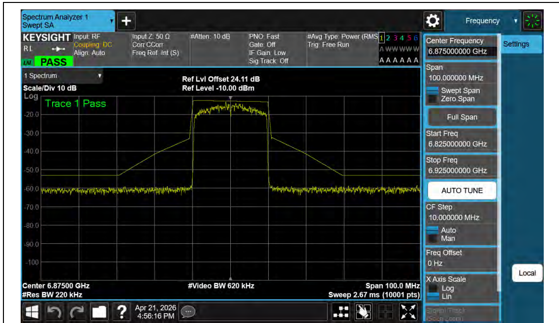
NTNV-11BE20MIMO-Ant2-6875-PASS
