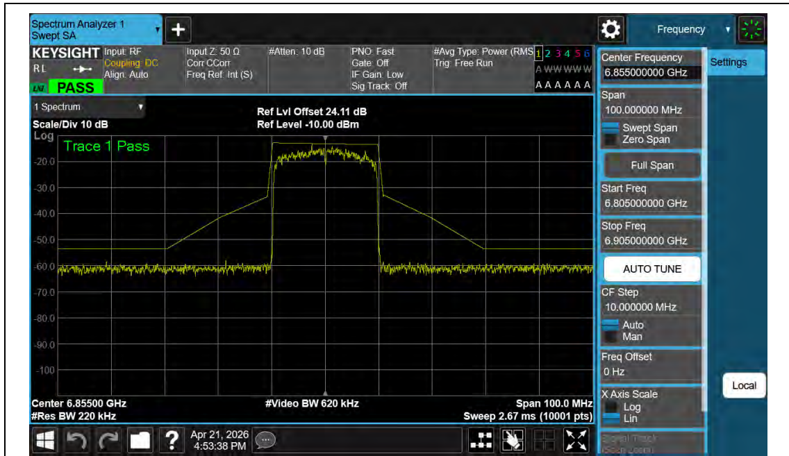
NTNV-11BE20MIMO-Ant2-6855-PASS
