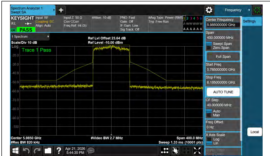
NTNV-11BE80MIMO-Ant2-5985-PASS
