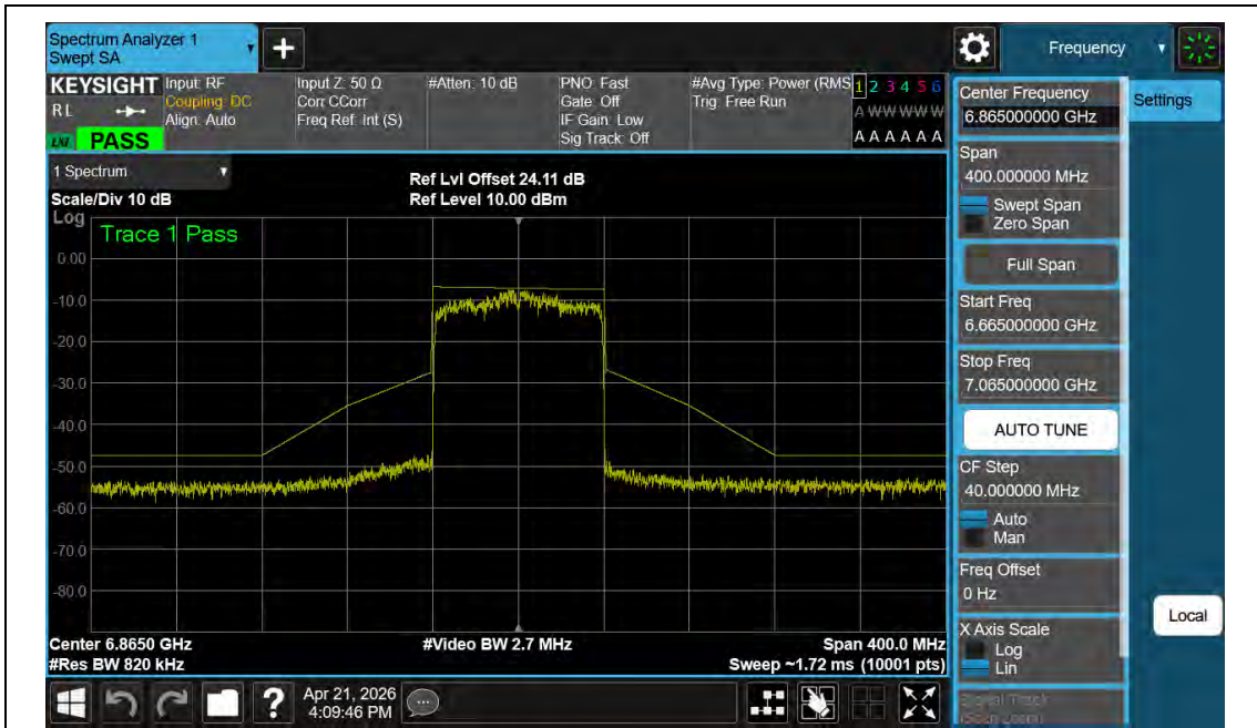
NTNV-11AX80MIMO-Ant2-6865-PASS
