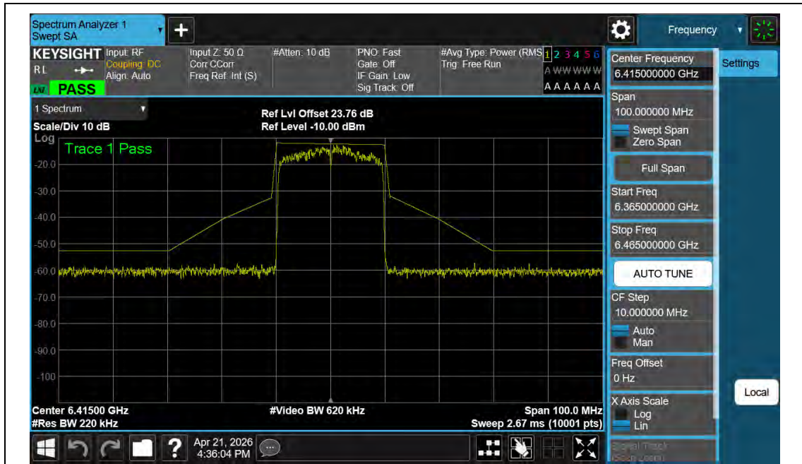
NTNV-11BE20MIMO-Ant2-6415-PASS
