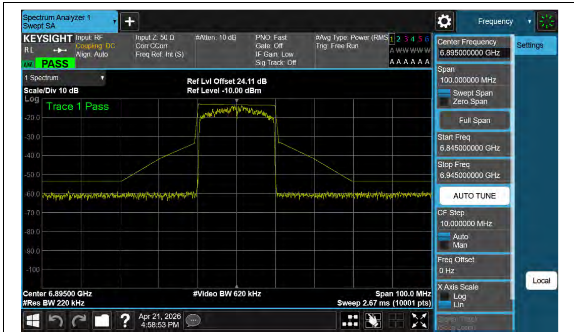
NTNV-11BE20MIMO-Ant2-6895-PASS
