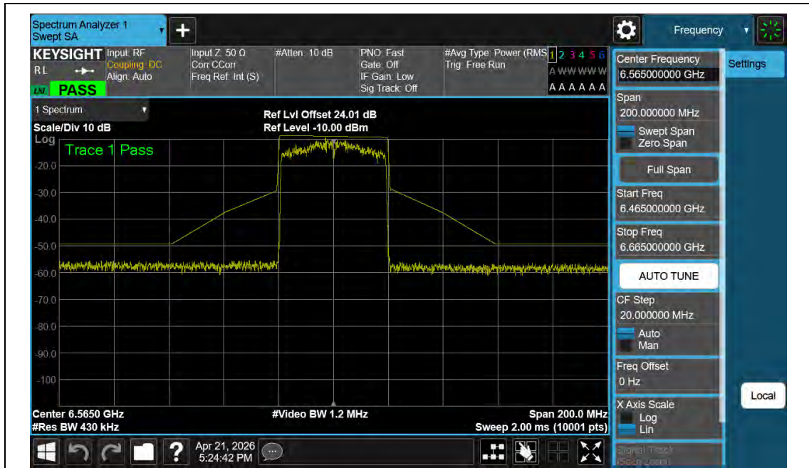
NTNV-11BE40MIMO-Ant2-6565-PASS
