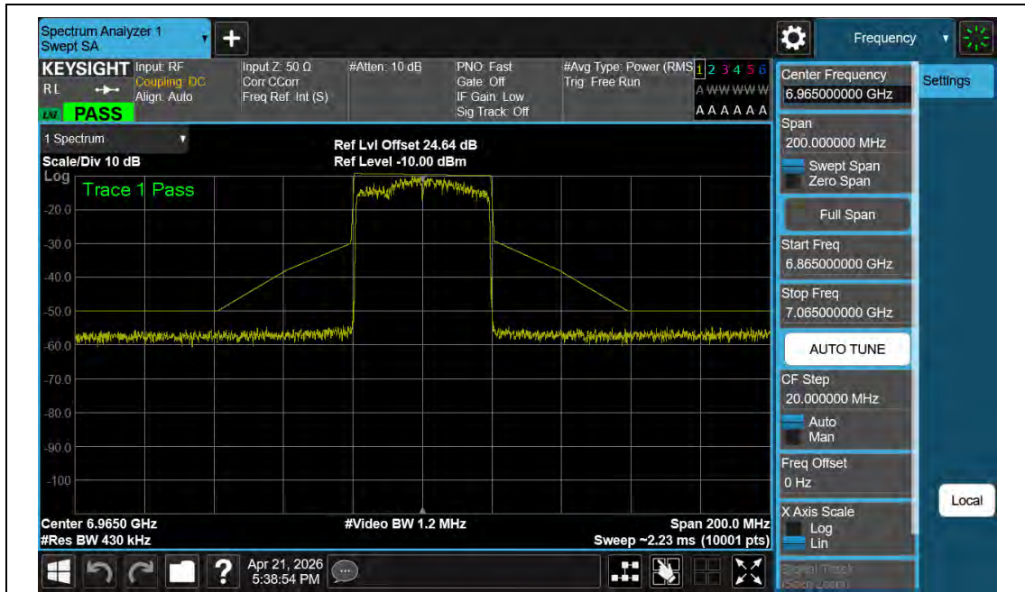
NTNV-11BE40MIMO-Ant2-6965-PASS
