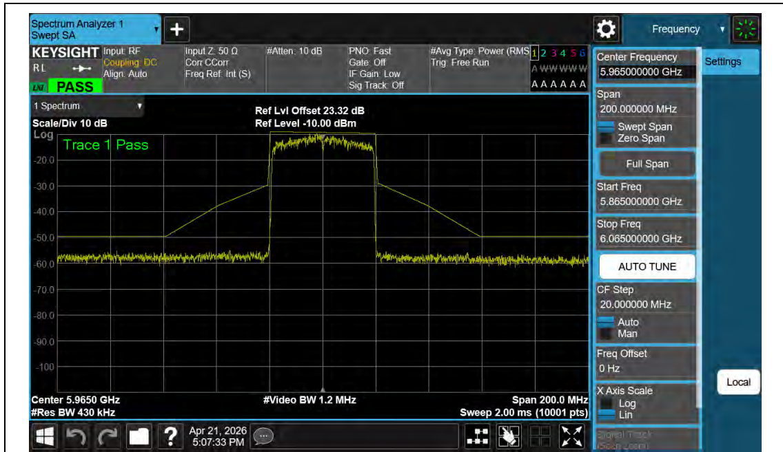
NTNV-11BE40MIMO-Ant2-5965-PASS
