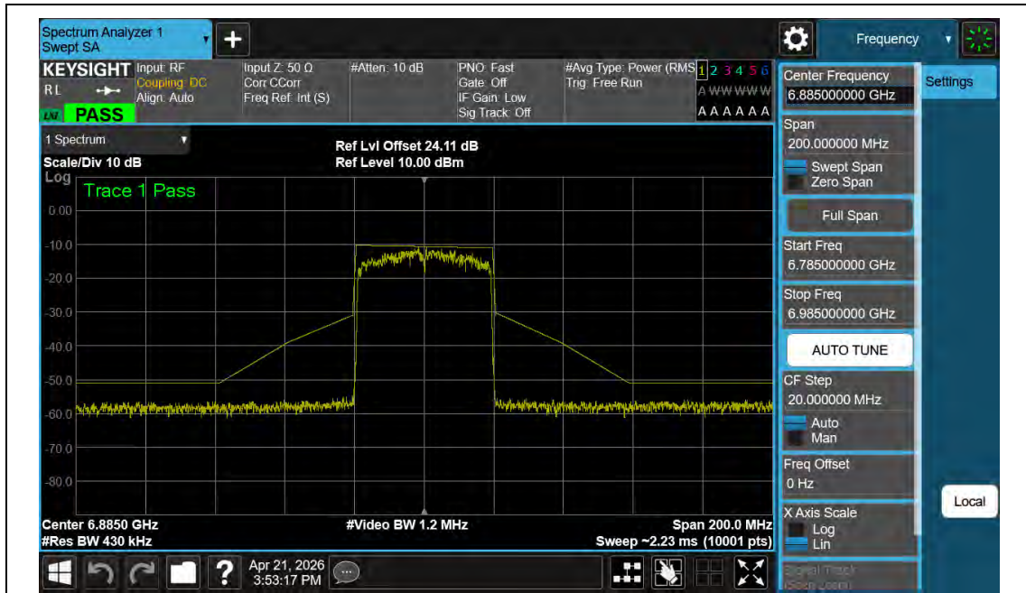
NTNV-11AX40MIMO-Ant2-6885-PASS
