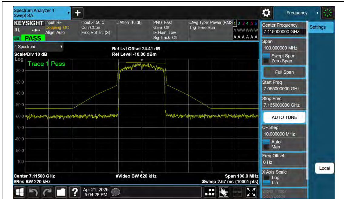
NTNV-11BE20MIMO-Ant2-7115-PASS
