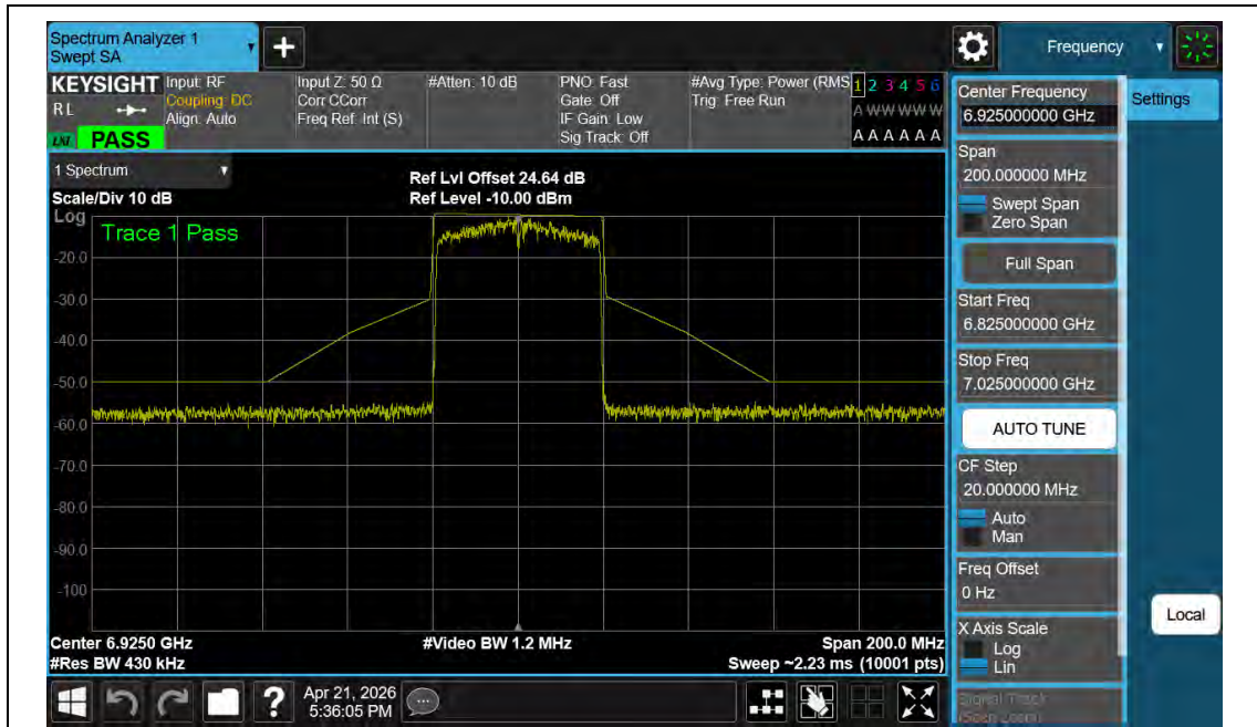
NTNV-11BE40MIMO-Ant2-6925-PASS
