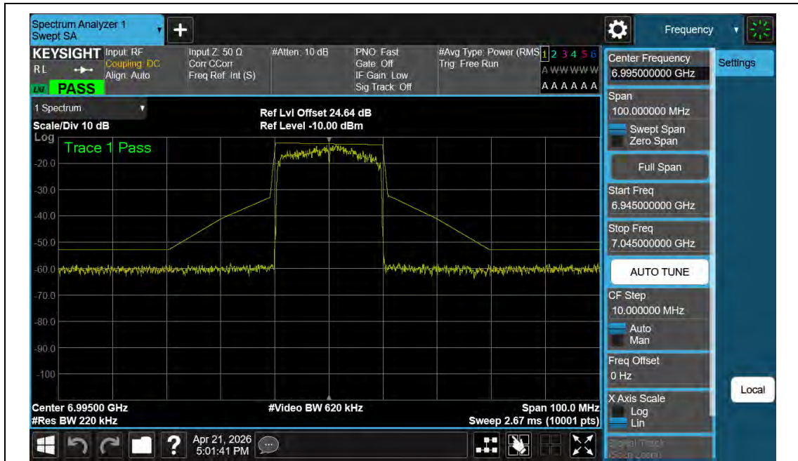
NTNV-11BE20MIMO-Ant2-6995-PASS
