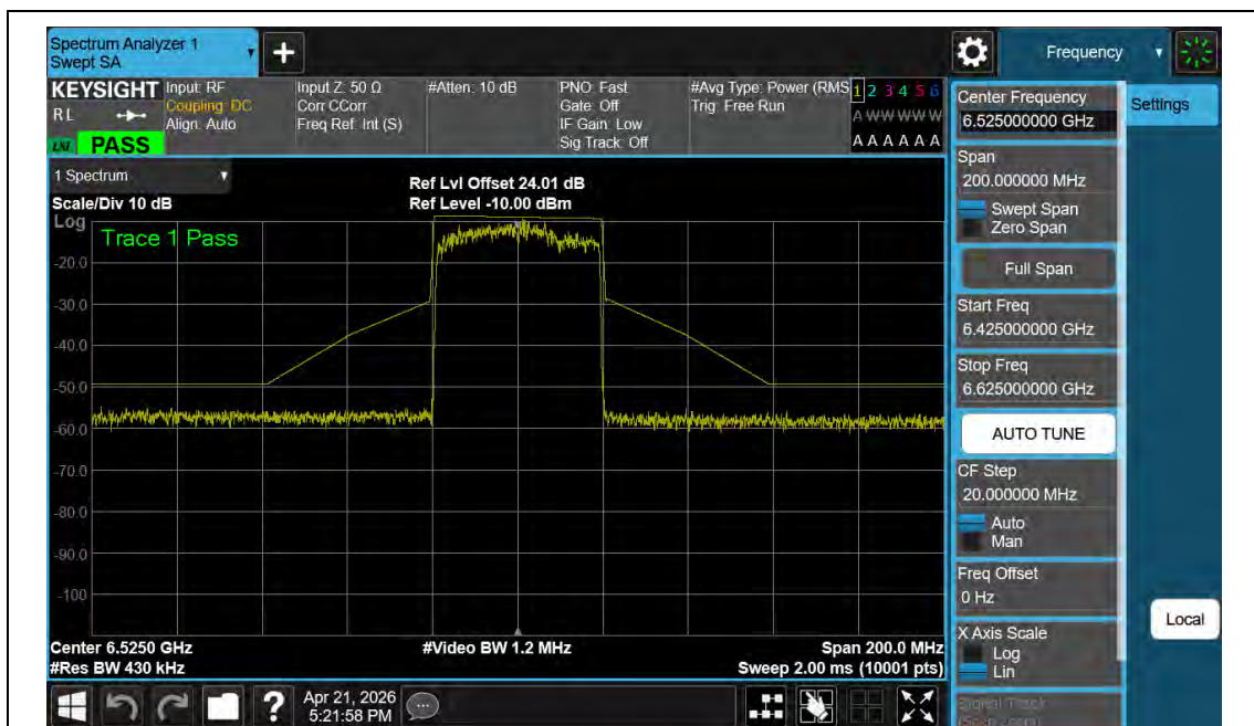
NTNV-11BE40MIMO-Ant2-6525-PASS
