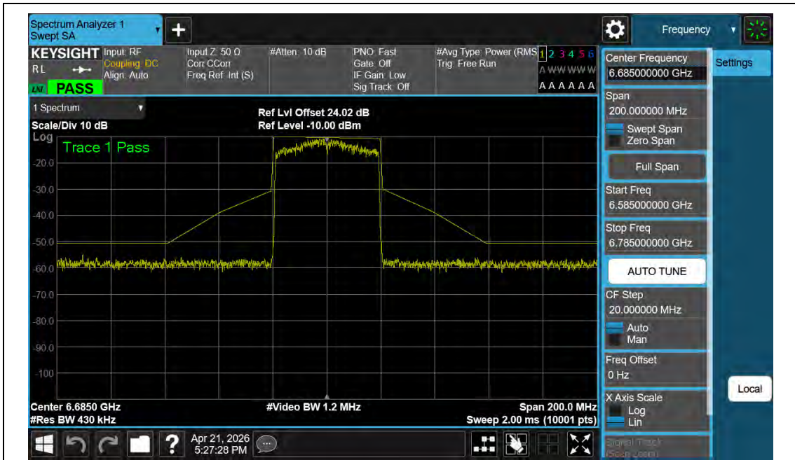
NTNV-11BE40MIMO-Ant2-6685-PASS
