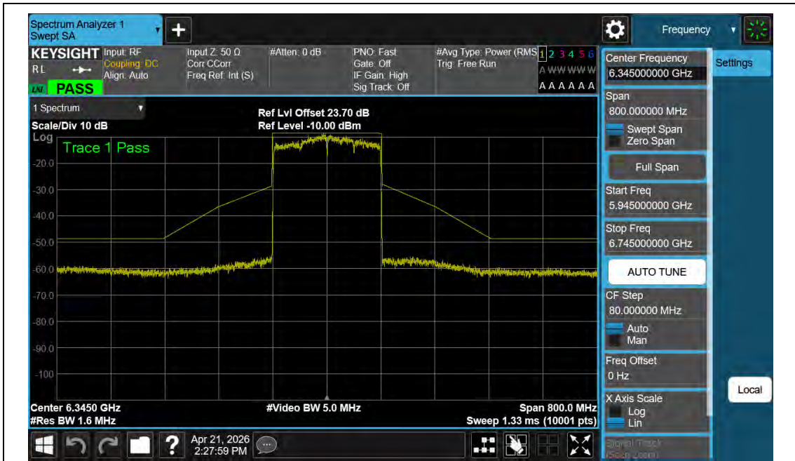
NTNV-11AX160MIMO-Ant2-6345-PASS
