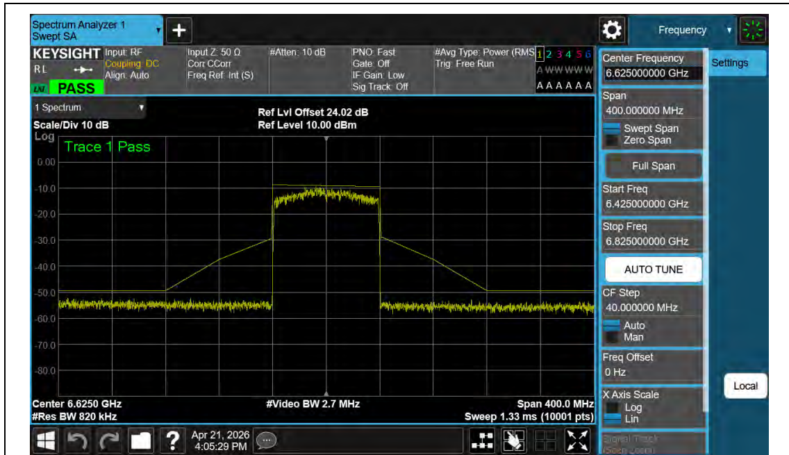
NTNV-11AX80MIMO-Ant2-6625-PASS
