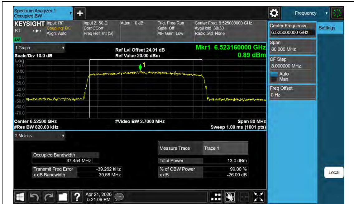
11BE40MIMO-Ant2-6525-PASS
