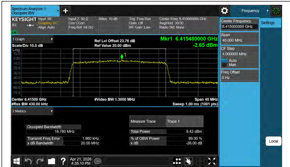
11BE20MIMO-Ant2-6415-PASS
