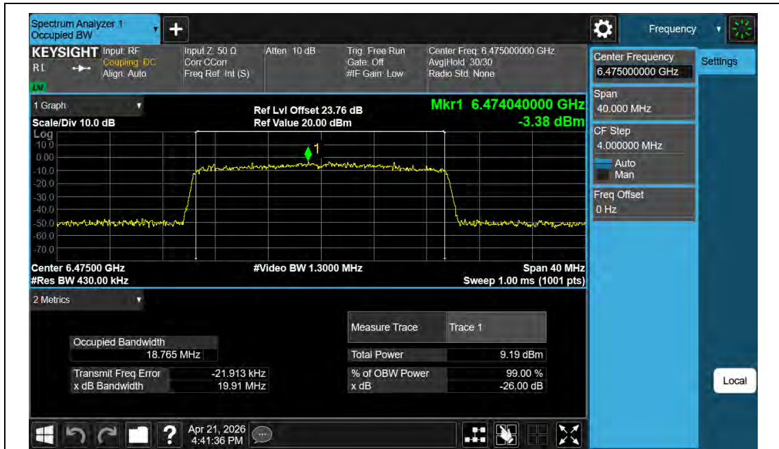
11BE20MIMO-Ant2-6475-PASS
