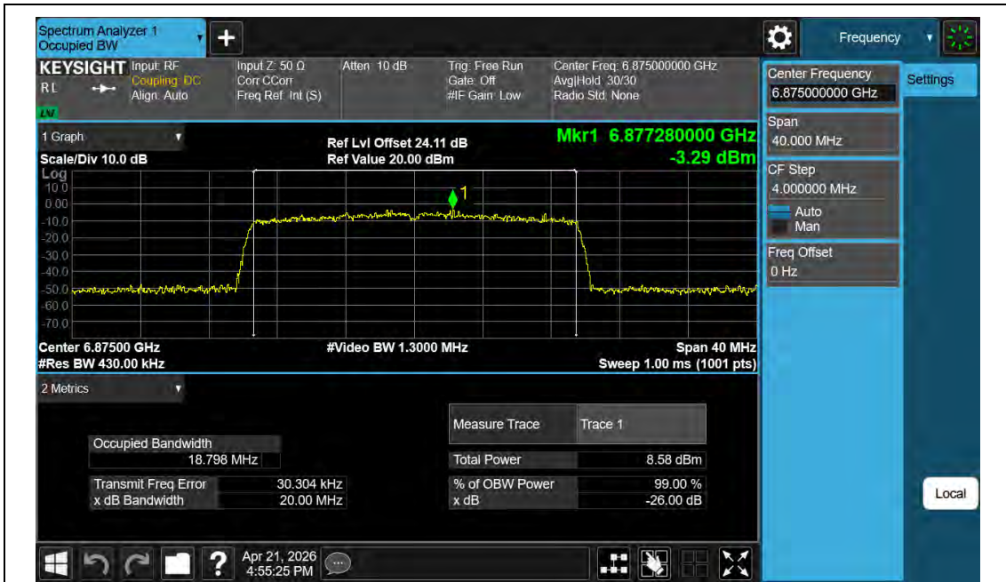
11BE20MIMO-Ant2-6875-PASS
