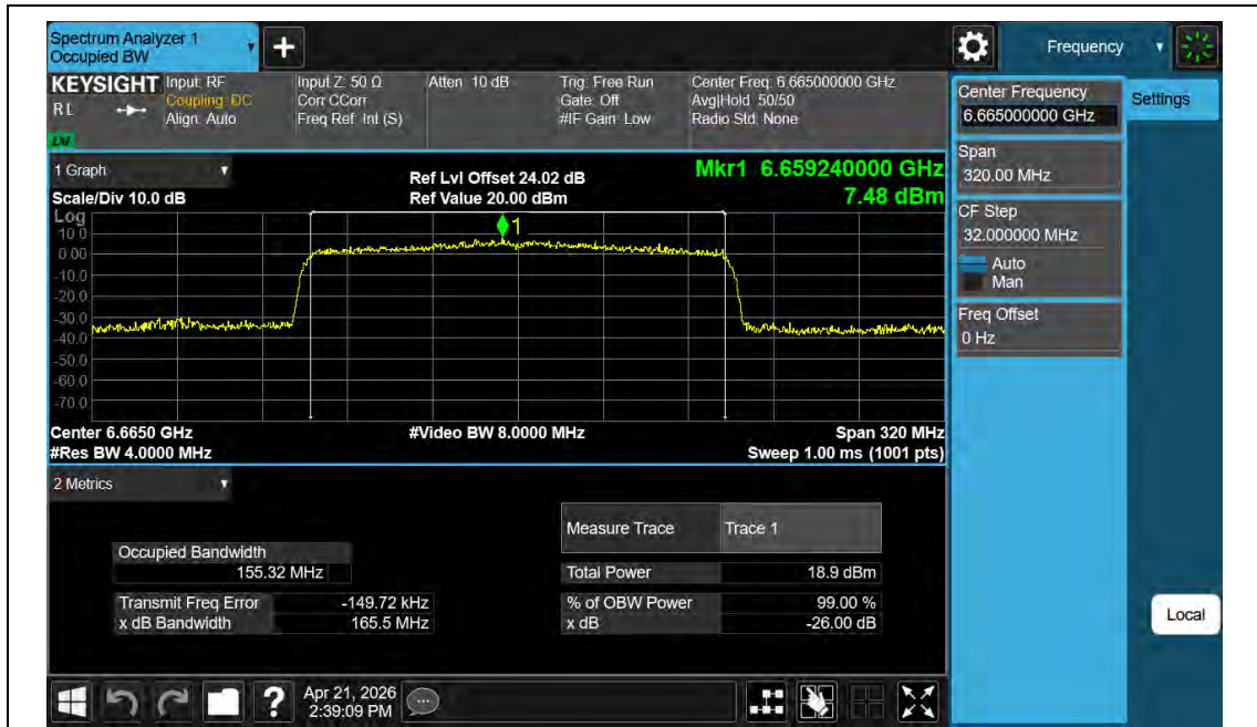
11AX160MIMO-Ant2-6665-PASS
