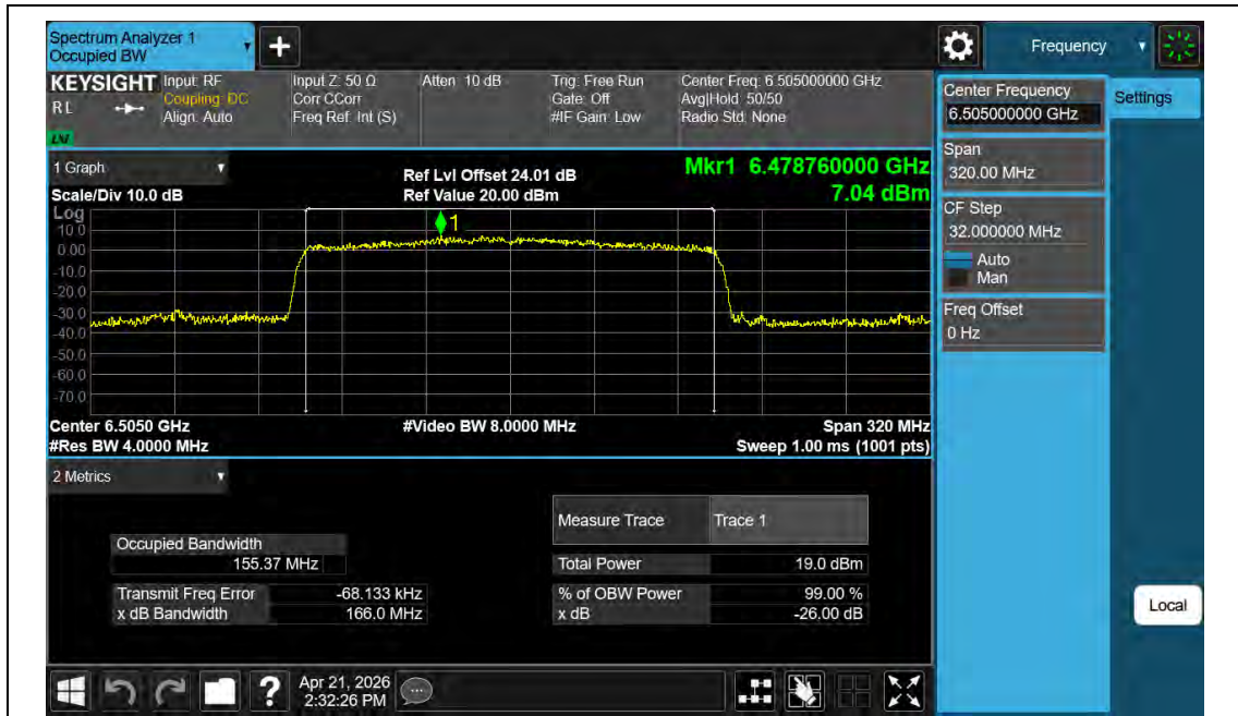
11AX160MIMO-Ant2-6505-PASS
