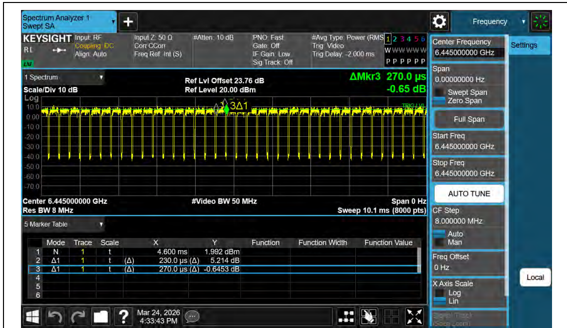
NTNV-11AX40MIMO-Ant2-6445
