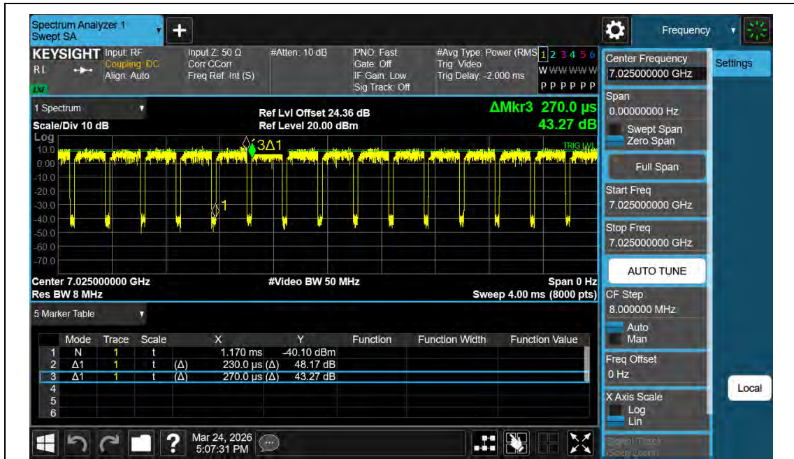
NTNV-11AX80MIMO-Ant2-7025
