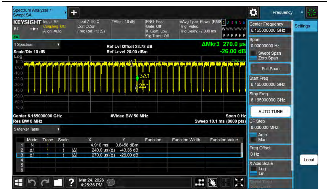
NTNV-11AX40MIMO-Ant2-6165
