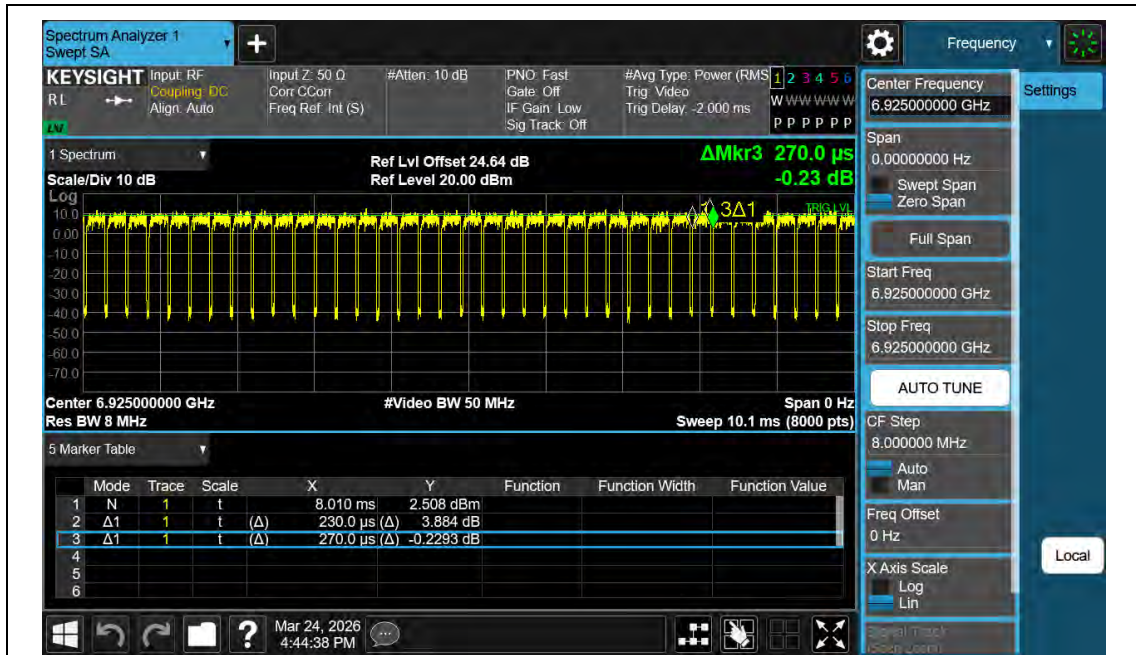
NTNV-11AX40MIMO-Ant2-6925
