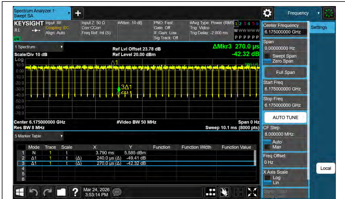
NTNV-11AX20MIMO-Ant2-6175
