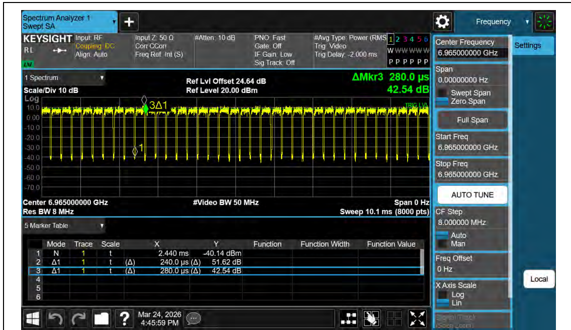
NTNV-11AX40MIMO-Ant2-6965
