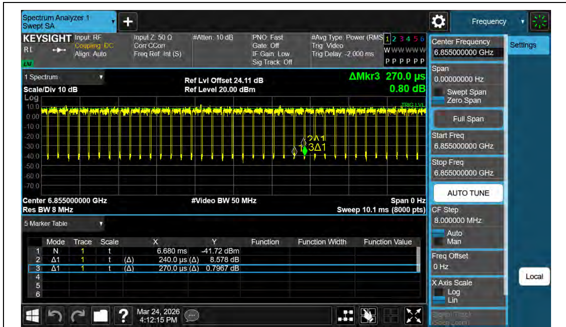
NTNV-11AX20MIMO-Ant2-6855
