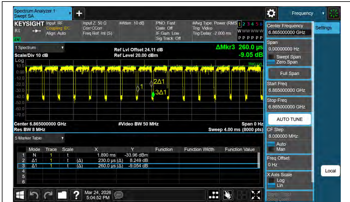
NTNV-11AX80MIMO-Ant2-6865
