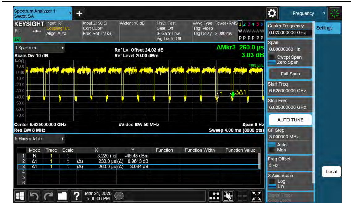
NTNV-11AX80MIMO-Ant2-6625
