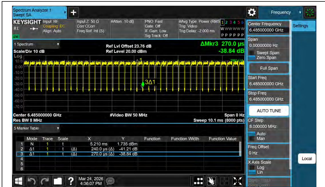
NTNV-11AX40MIMO-Ant2-6485
