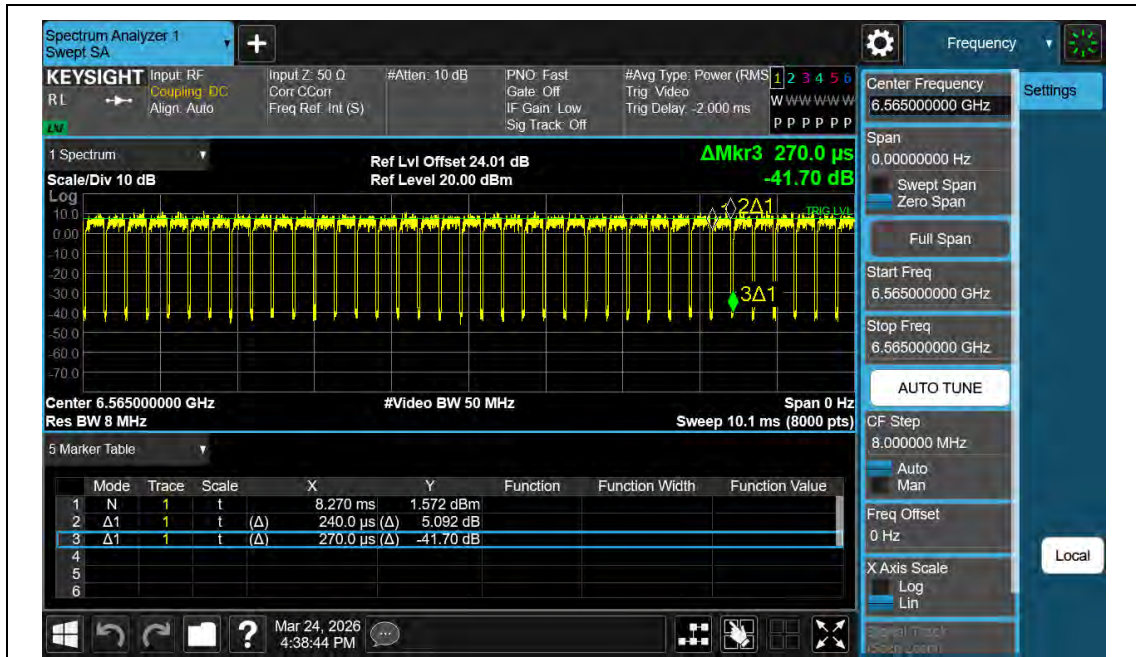
NTNV-11AX40MIMO-Ant2-6565
