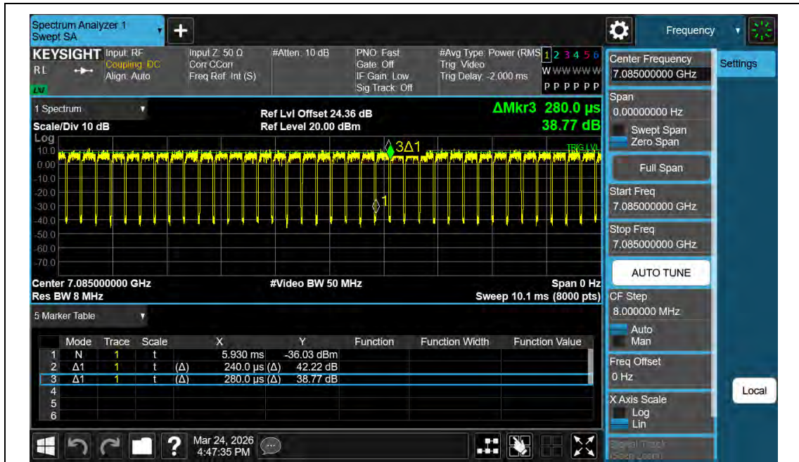
NTNV-11AX40MIMO-Ant2-7085
