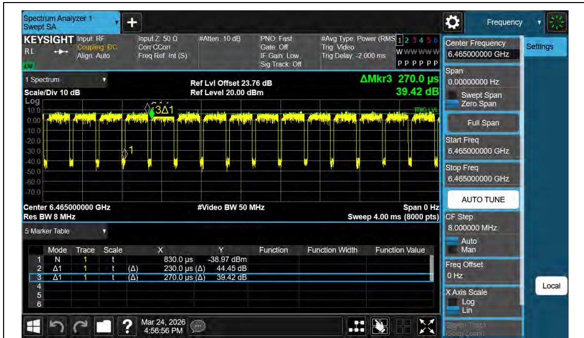
NTNV-11AX80MIMO-Ant2-6465
