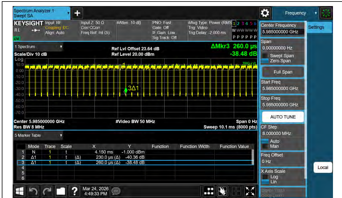
NTNV-11AX80MIMO-Ant2-5985
