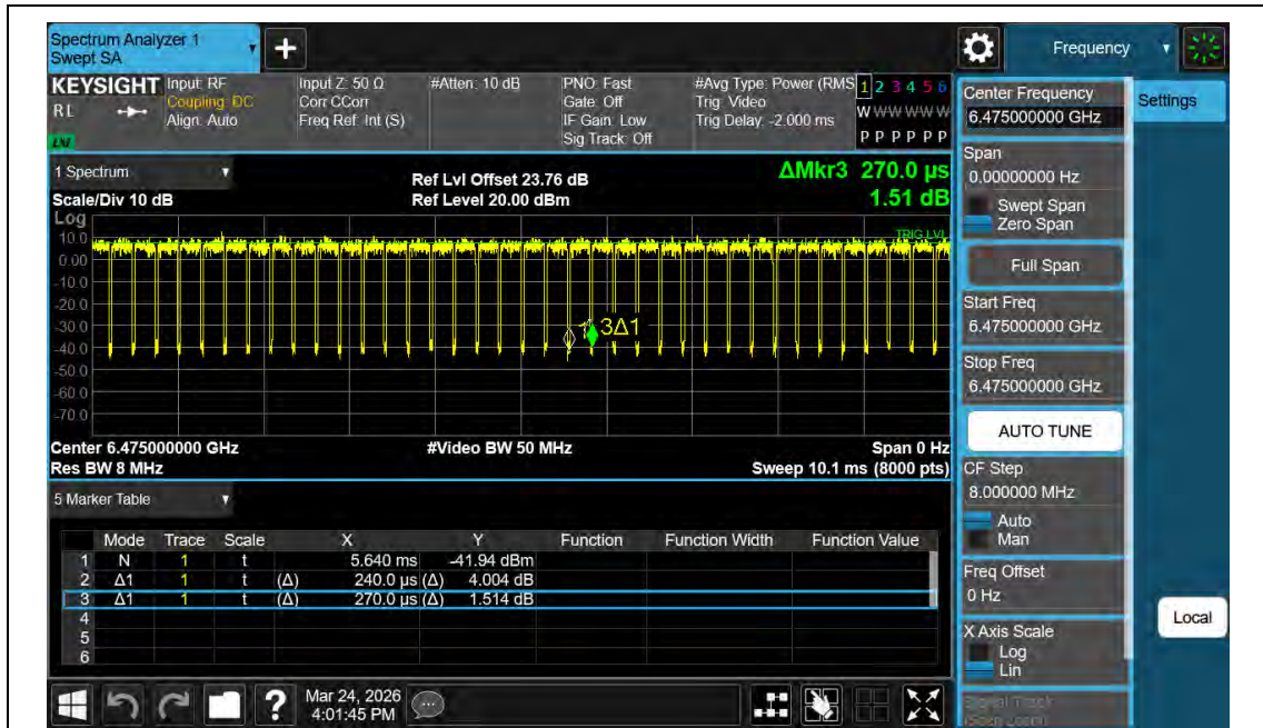
NTNV-11AX20MIMO-Ant2-6475
