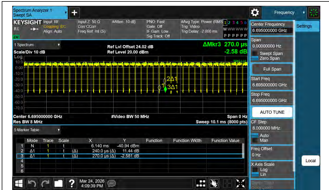
NTNV-11AX20MIMO-Ant2-6695
