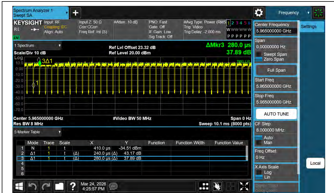
NTNV-11AX40MIMO-Ant2-5965
