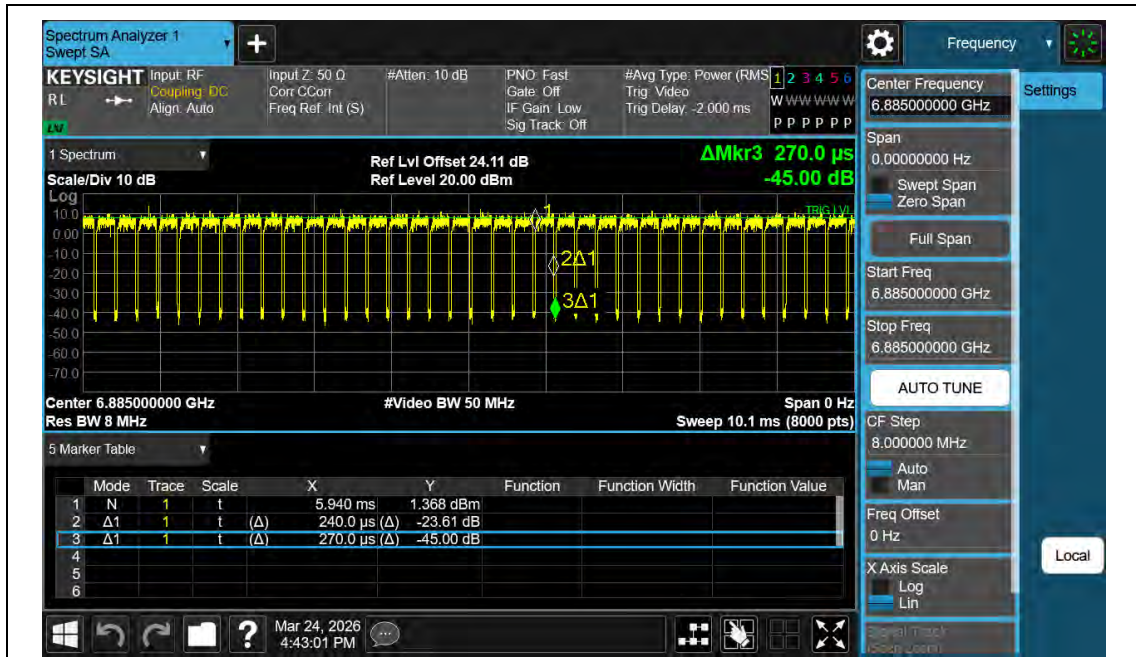
NTNV-11AX40MIMO-Ant2-6885
