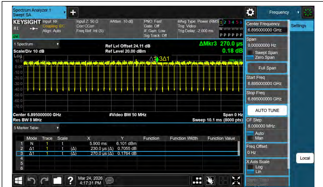
NTNV-11AX20MIMO-Ant2-6895
