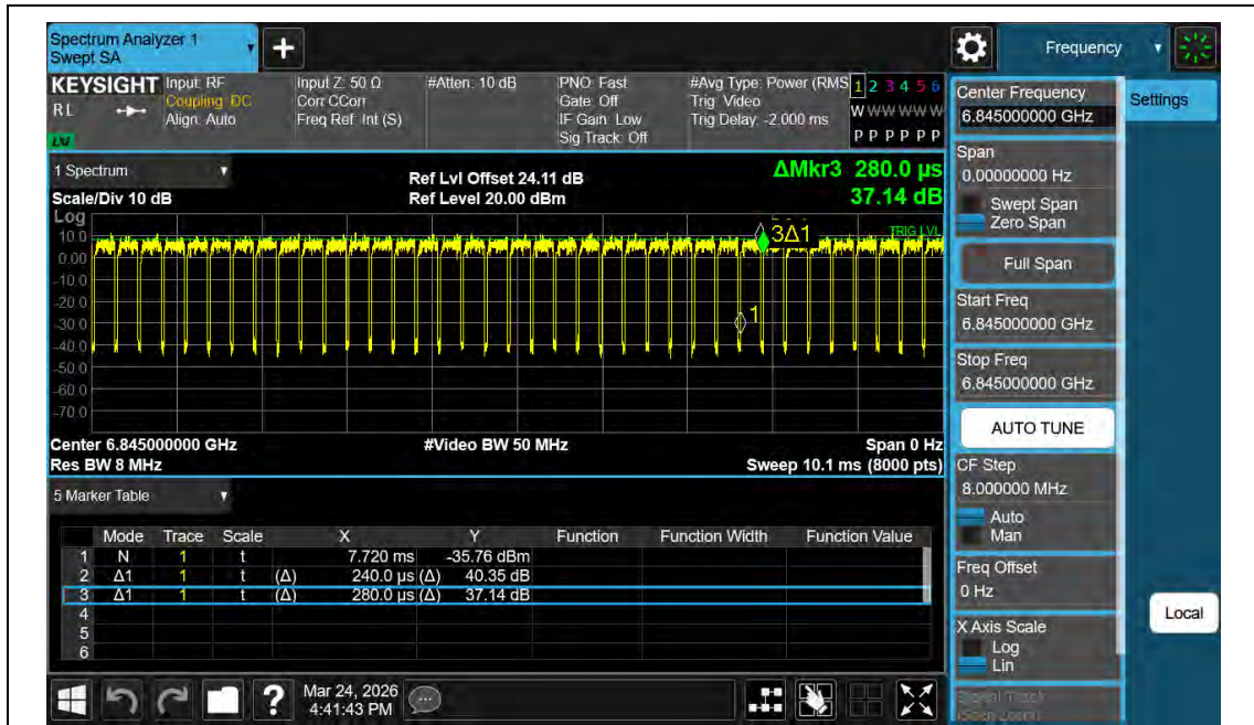
NTNV-11AX40MIMO-Ant2-6845
