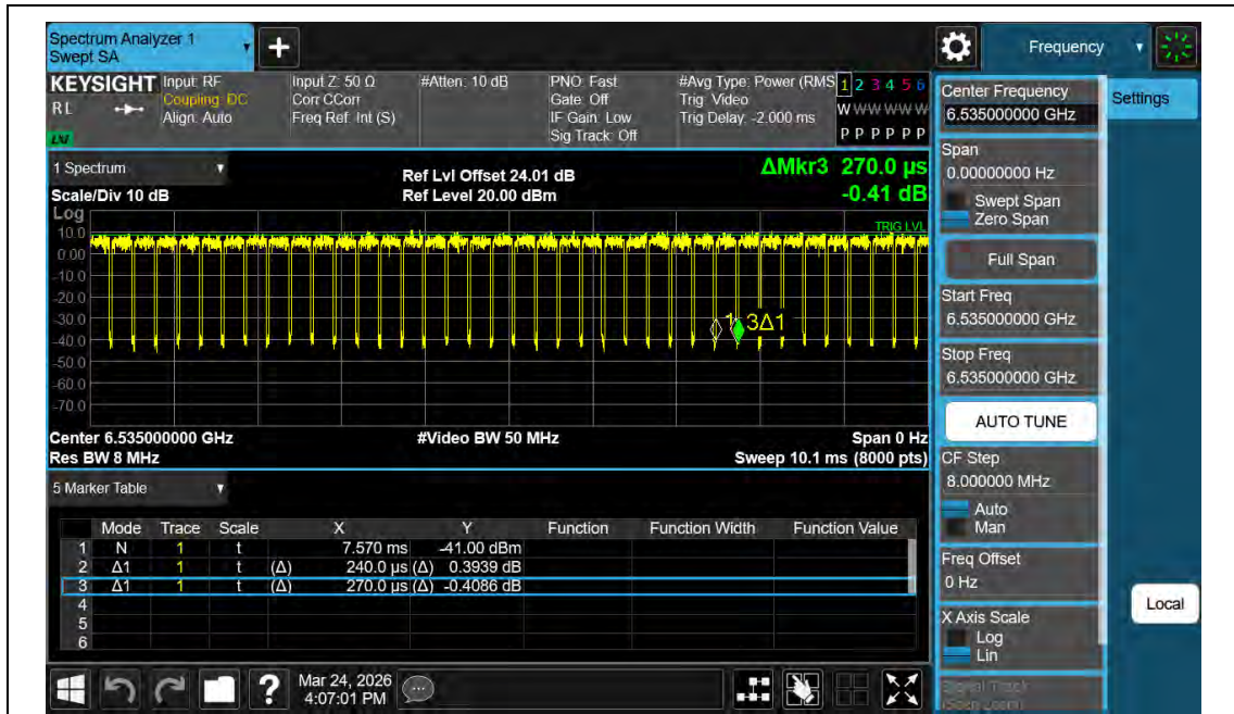
NTNV-11AX20MIMO-Ant2-6535
