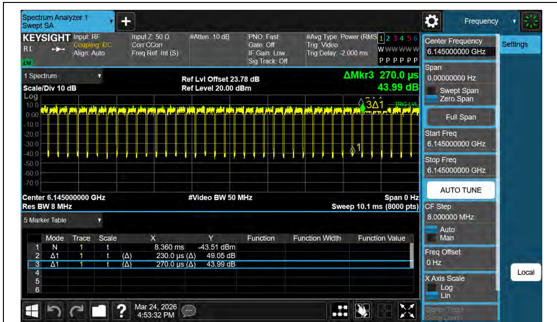
NTNV-11AX80MIMO-Ant2-6145
