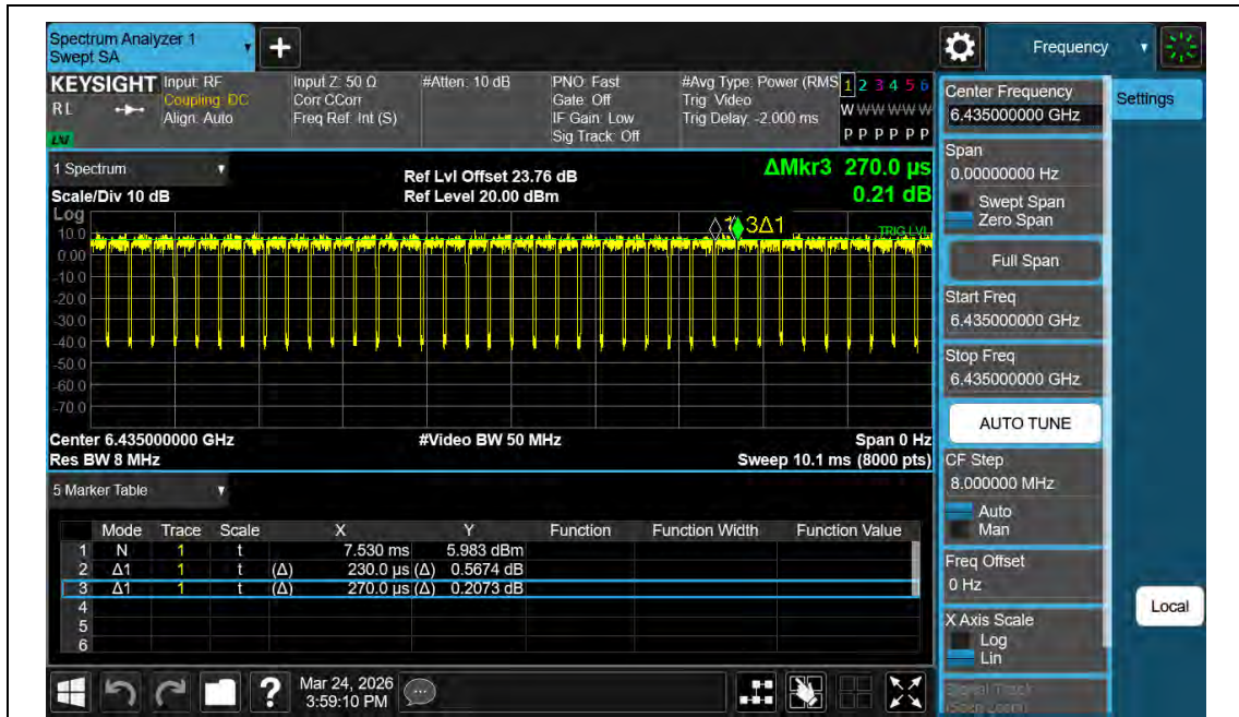
NTNV-11AX20MIMO-Ant2-6435
