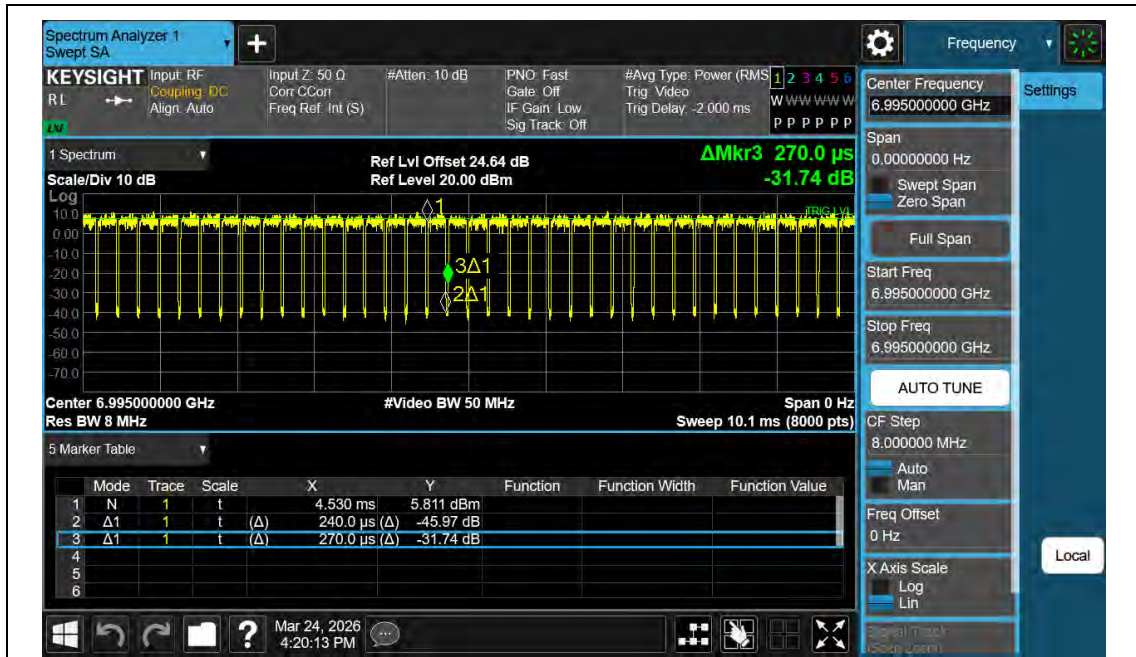
NTNV-11AX20MIMO-Ant2-6995
