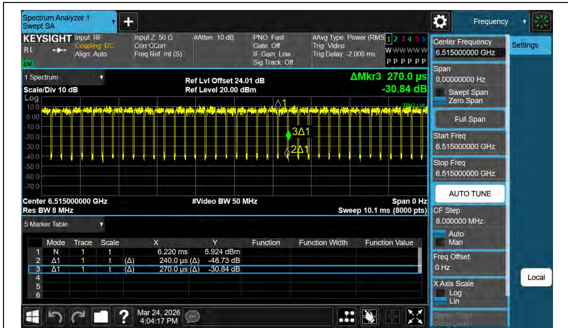
NTNV-11AX20MIMO-Ant2-6515
