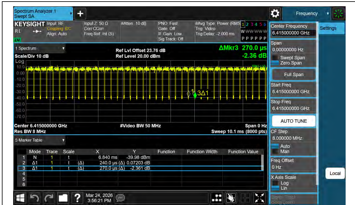
NTNV-11AX20MIMO-Ant2-6415
