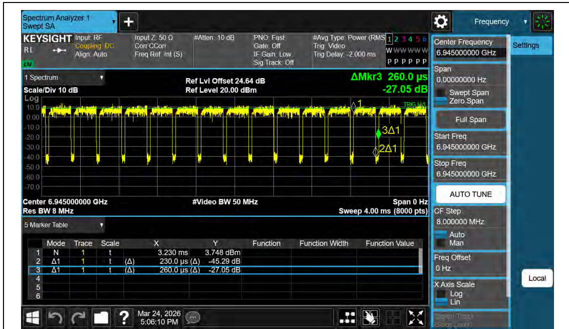
NTNV-11AX80MIMO-Ant2-6945
