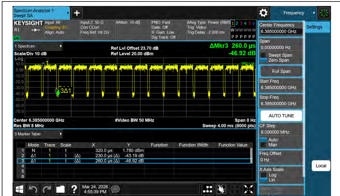
NTNV-11AX80MIMO-Ant2-6385
