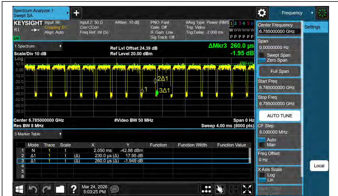
NTNV-11AX80MIMO-Ant2-6785
