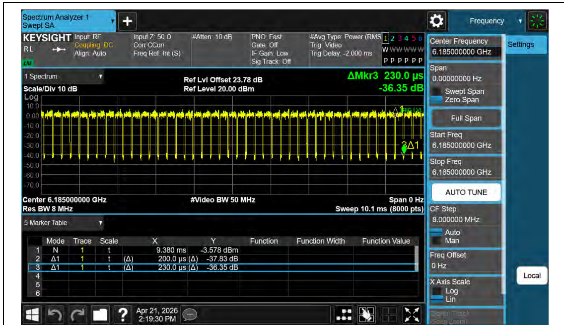
NTNV-11AX160MIMO-Ant2-6185
