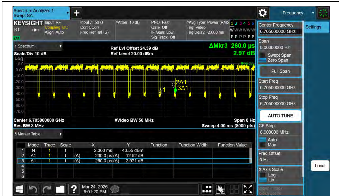
NTNV-11AX80MIMO-Ant2-6705
