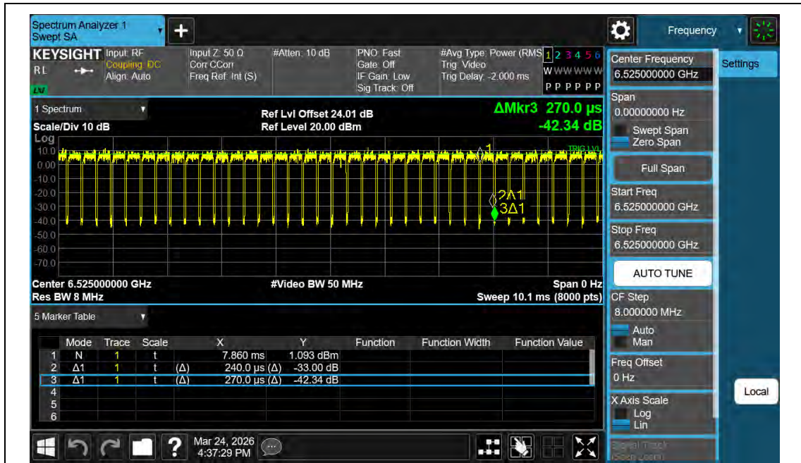
NTNV-11AX40MIMO-Ant2-6525
