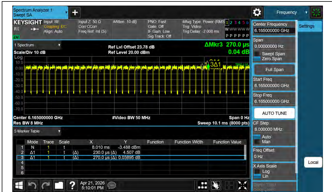
NTNV-11BE40MIMO-Ant2-6165
