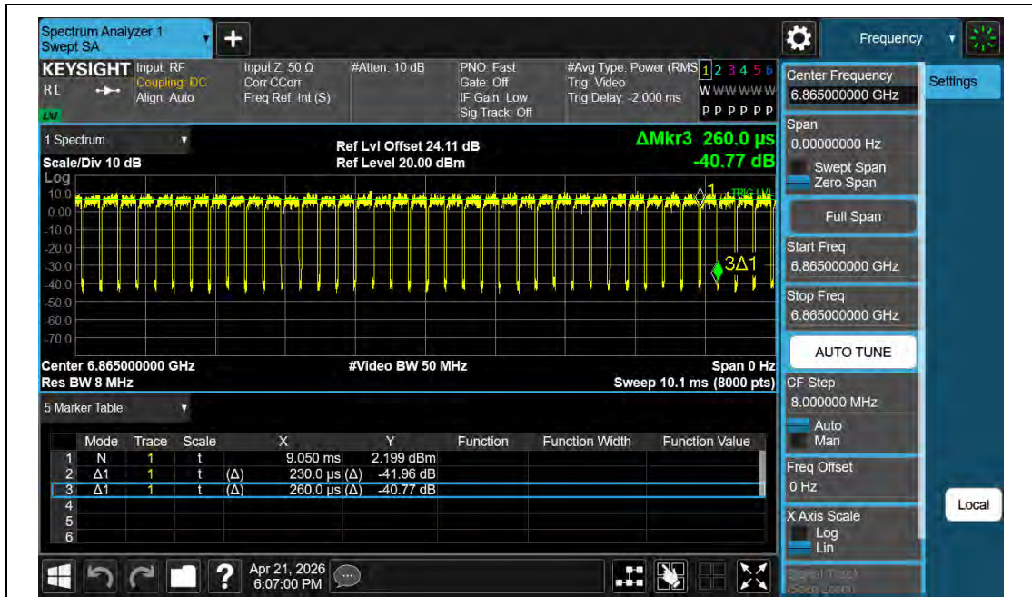
NTNV-11BE80MIMO-Ant2-6865
