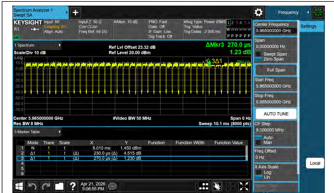
NTNV-11BE40MIMO-Ant2-5965
