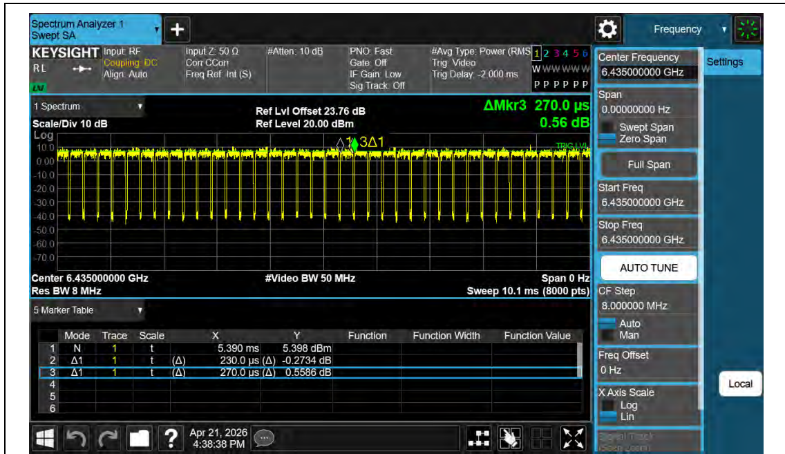
NTNV-11BE20MIMO-Ant2-6435
