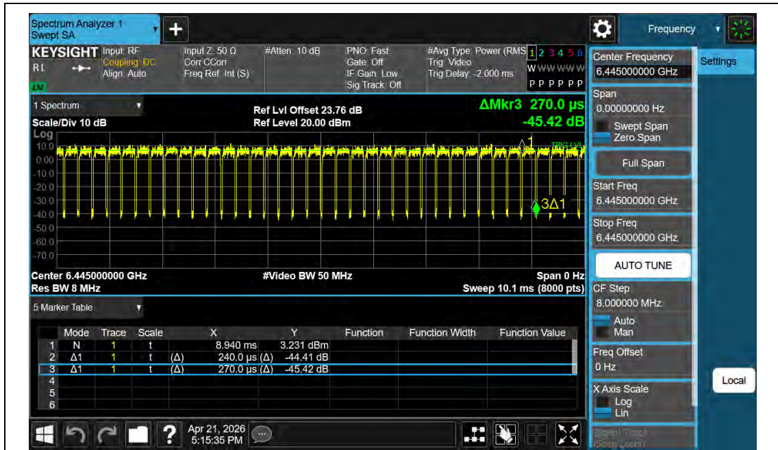
NTNV-11BE40MIMO-Ant2-6445
