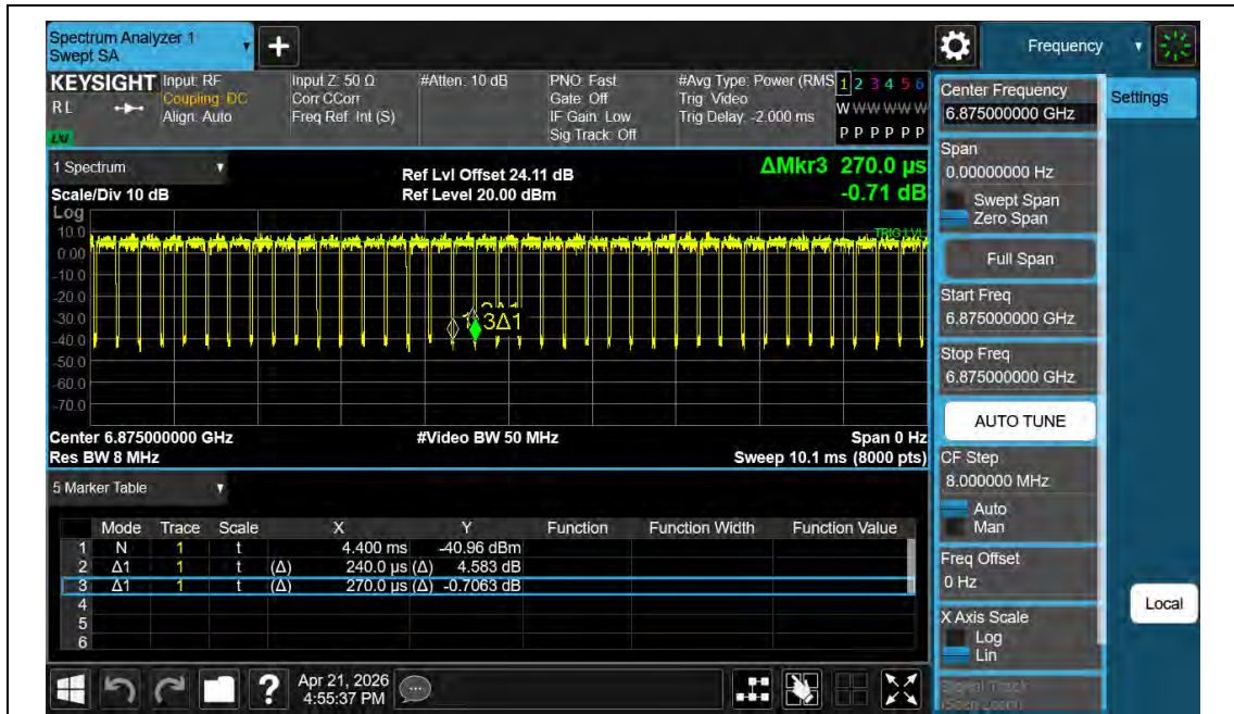
NTNV-11BE20MIMO-Ant2-6875
