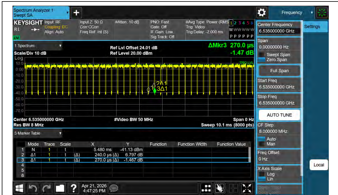
NTNV-11BE20MIMO-Ant2-6535
