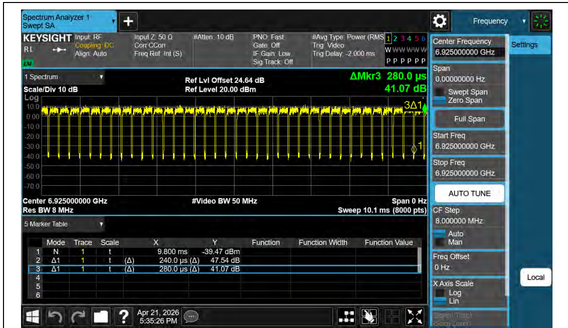
NTNV-11BE40MIMO-Ant2-6925
