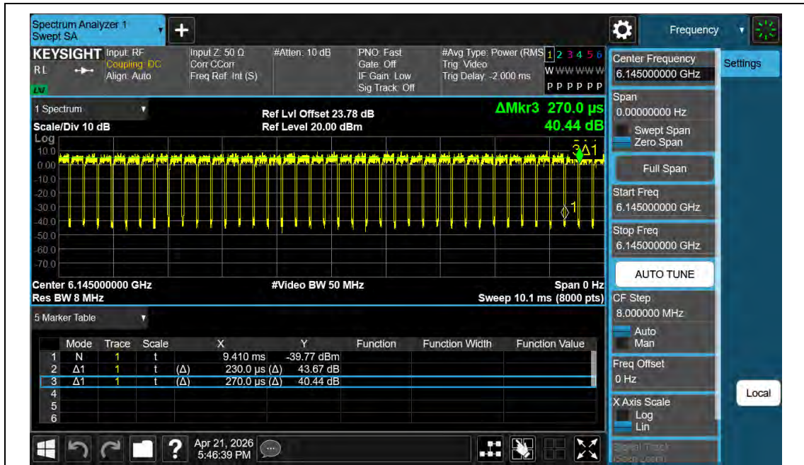
NTNV-11BE80MIMO-Ant2-6145
