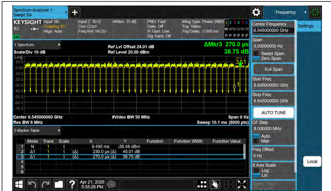
NTNV-11BE80MIMO-Ant2-6545
