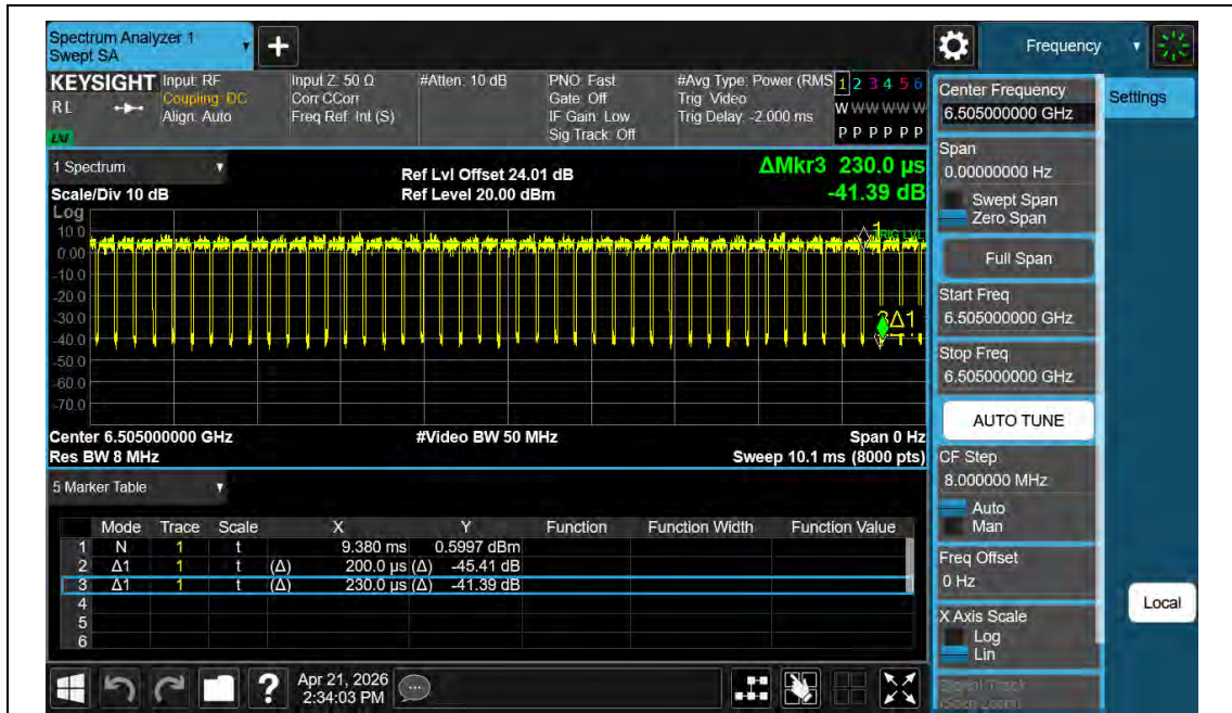
NTNV-11AX160MIMO-Ant2-6505
