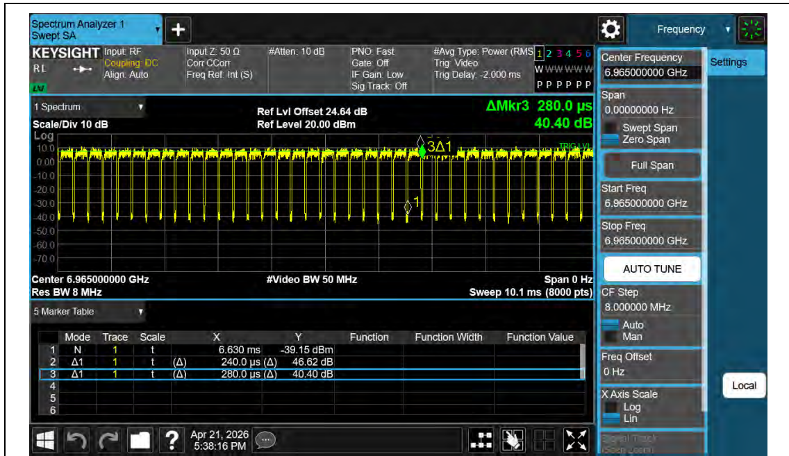
NTNV-11BE40MIMO-Ant2-6965
