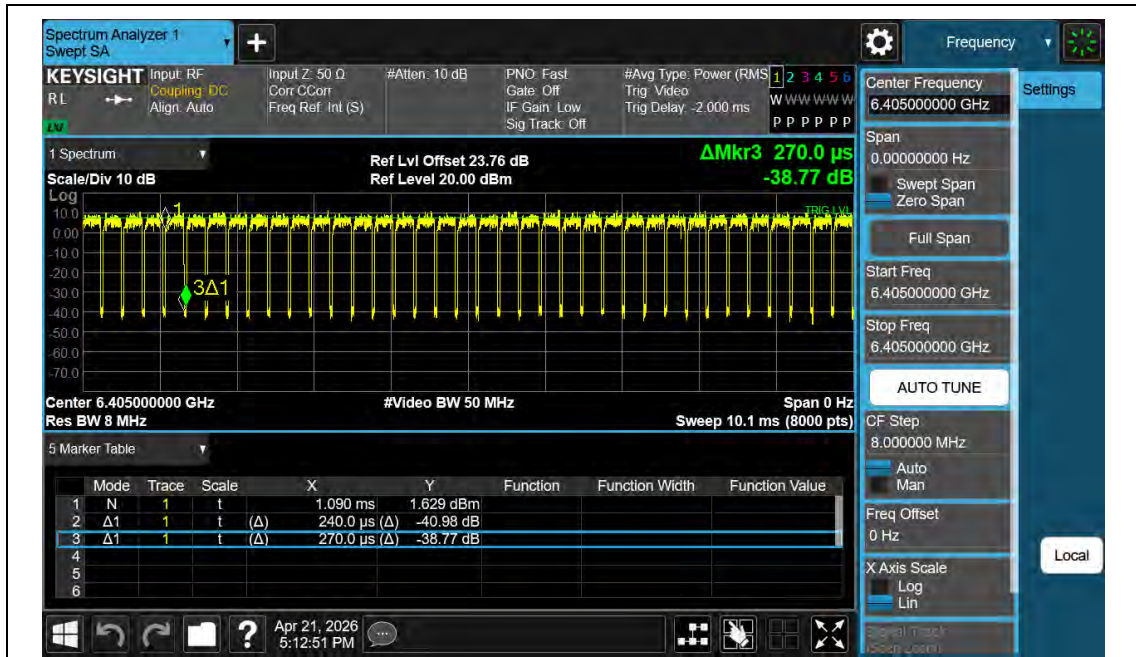
NTNV-11BE40MIMO-Ant2-6405
