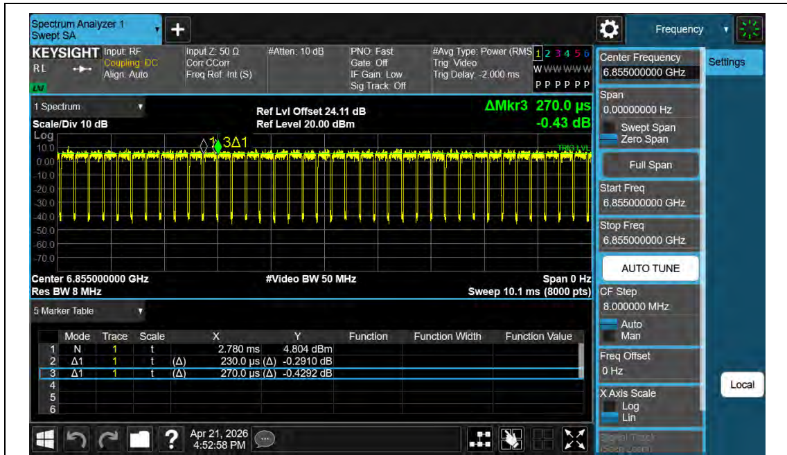
NTNV-11BE20MIMO-Ant2-6855
