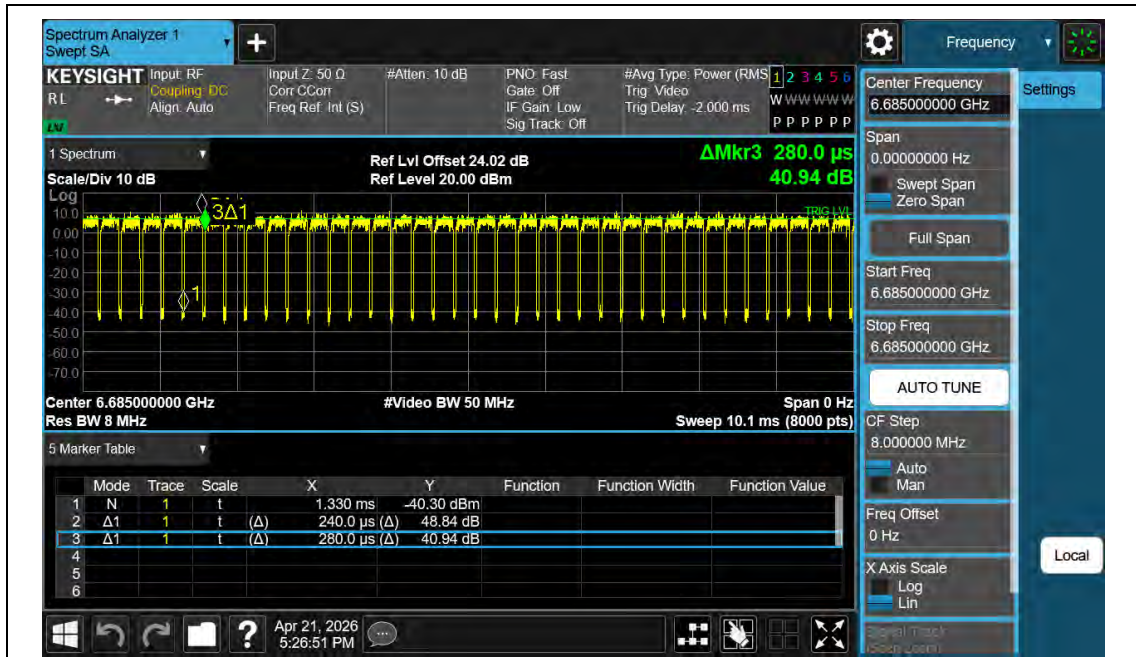
NTNV-11BE40MIMO-Ant2-6685
