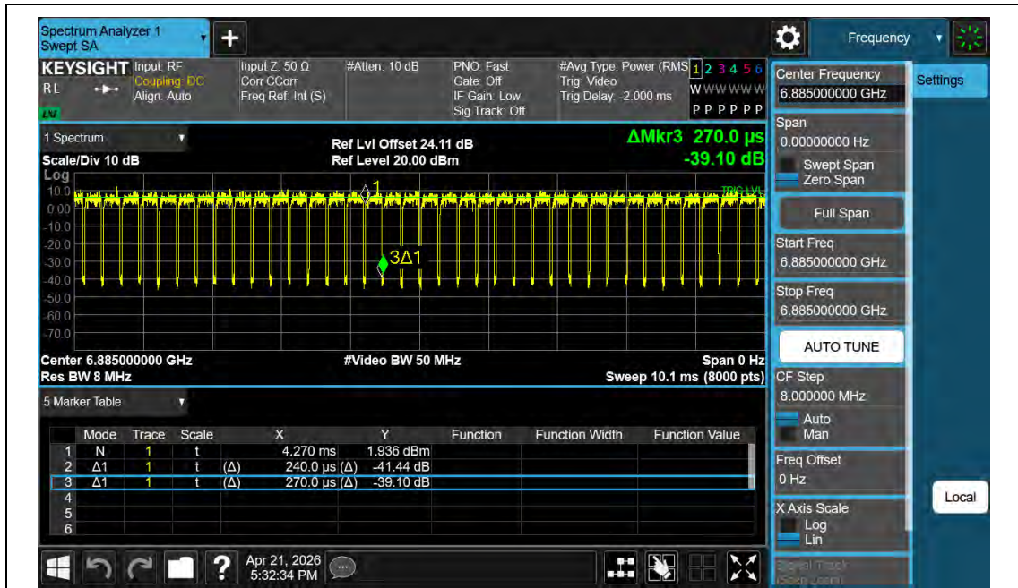
NTNV-11BE40MIMO-Ant2-6885
