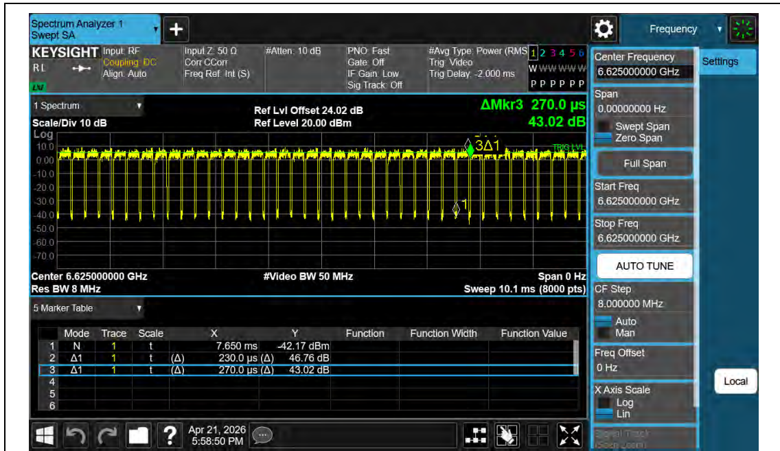
NTNV-11BE80MIMO-Ant2-6625
