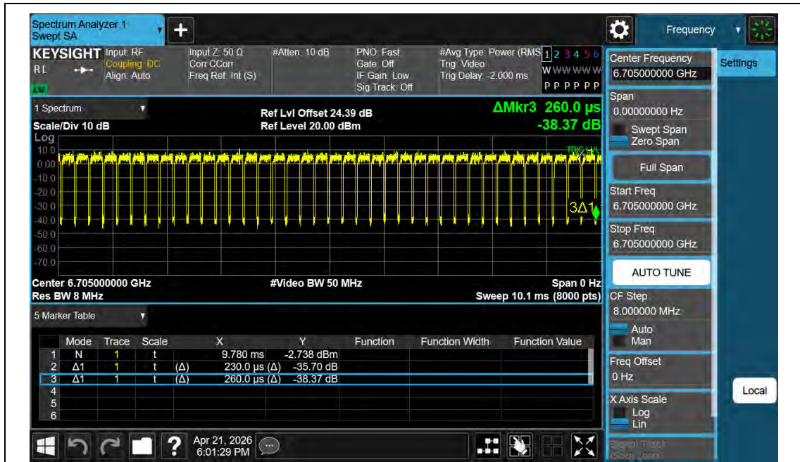
NTNV-11BE80MIMO-Ant2-6705
