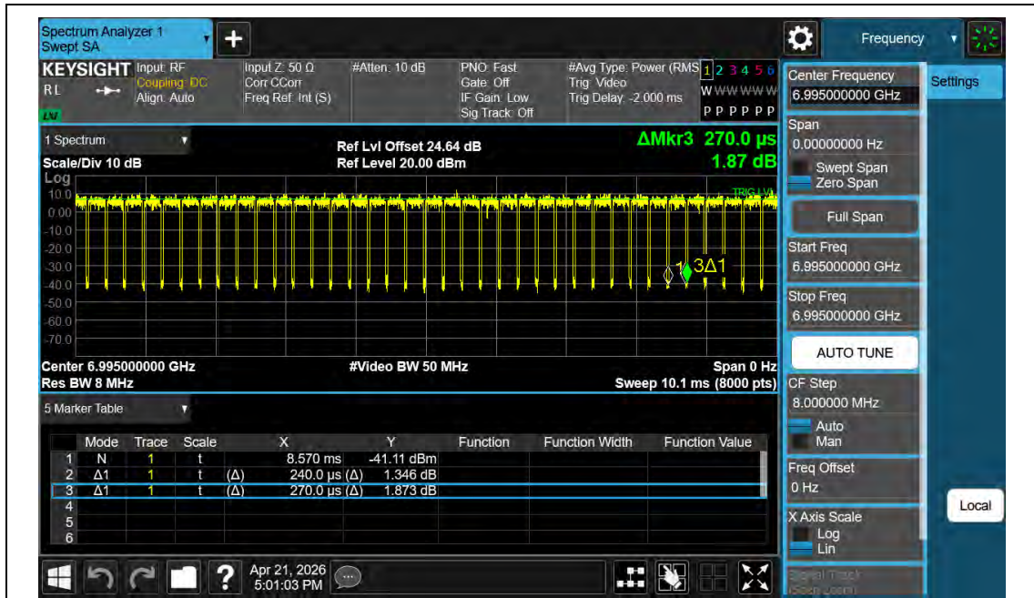
NTNV-11BE20MIMO-Ant2-6995
