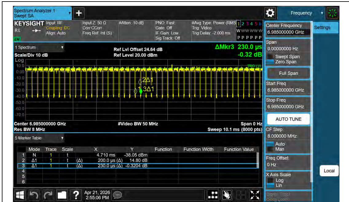
NTNV-11AX160MIMO-Ant2-6985
