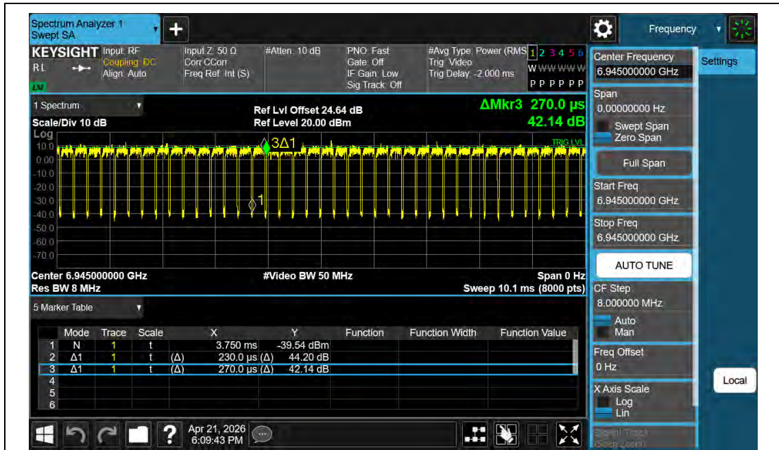
NTNV-11BE80MIMO-Ant2-6945
