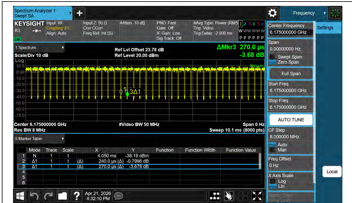
NTNV-11BE20MIMO-Ant2-6175
