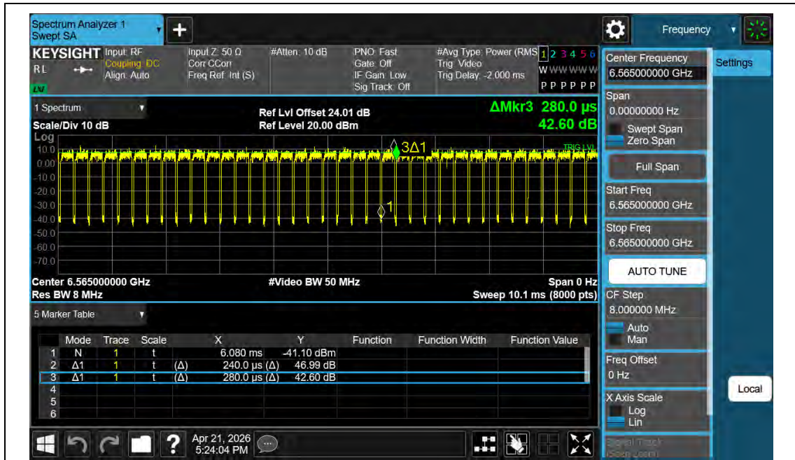
NTNV-11BE40MIMO-Ant2-6565
