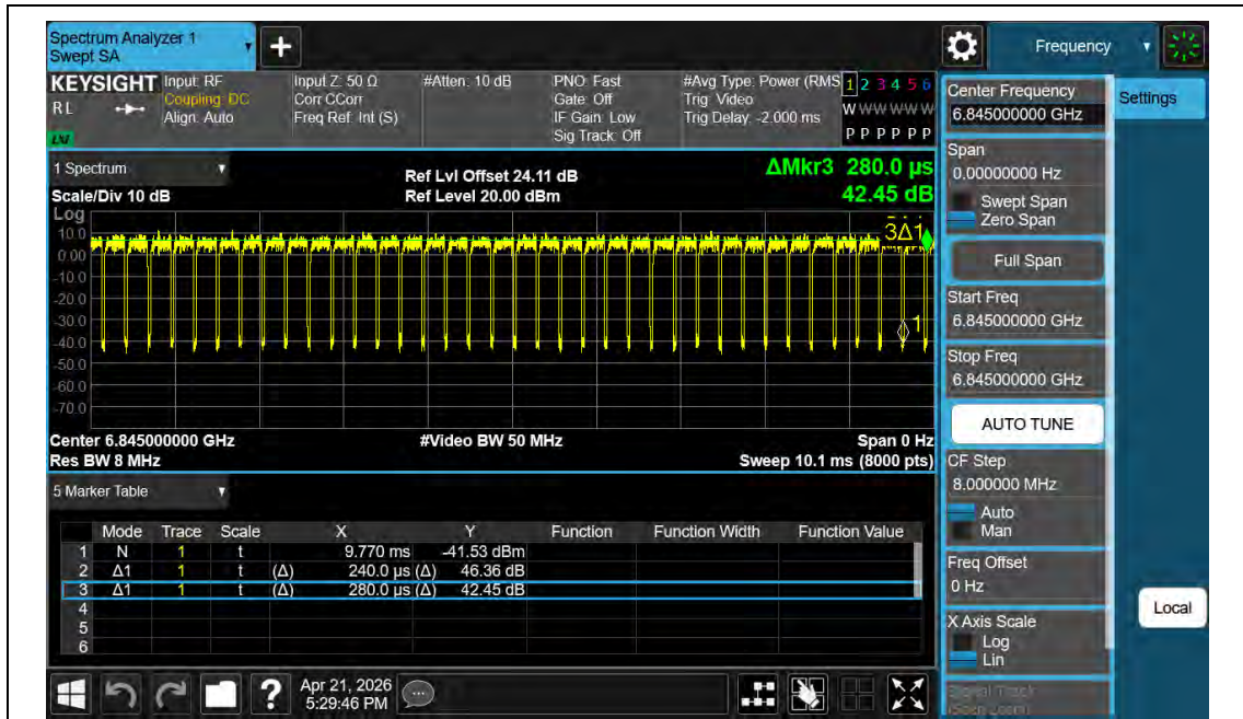
NTNV-11BE40MIMO-Ant2-6845
