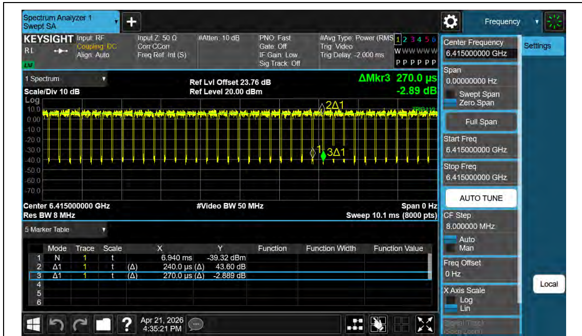
NTNV-11BE20MIMO-Ant2-6415
