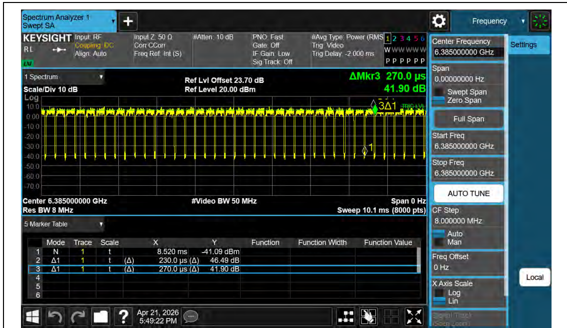
NTNV-11BE80MIMO-Ant2-6385
