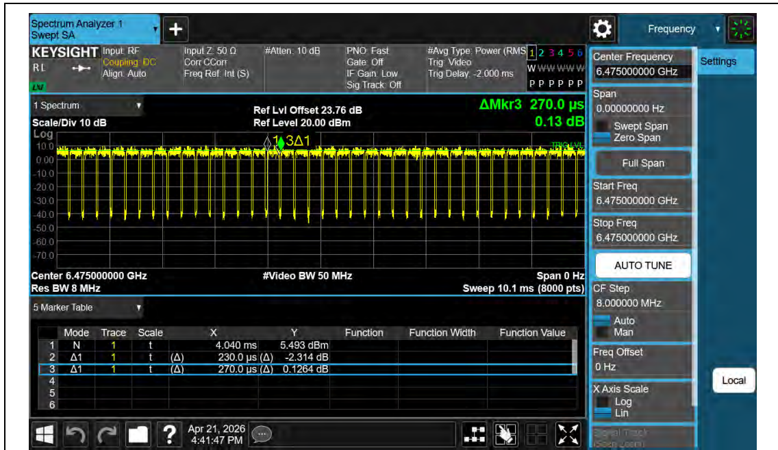
NTNV-11BE20MIMO-Ant2-6475
