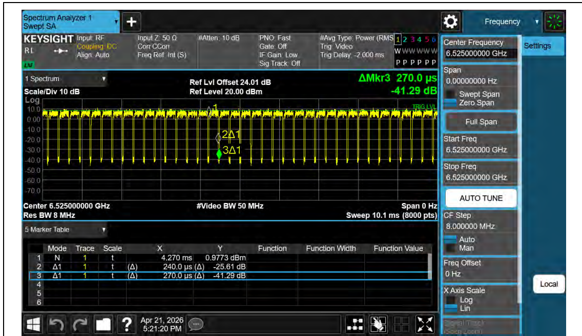
NTNV-11BE40MIMO-Ant2-6525
