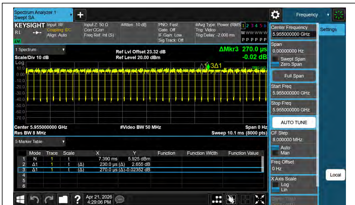
NTNV-11BE20MIMO-Ant2-5955
