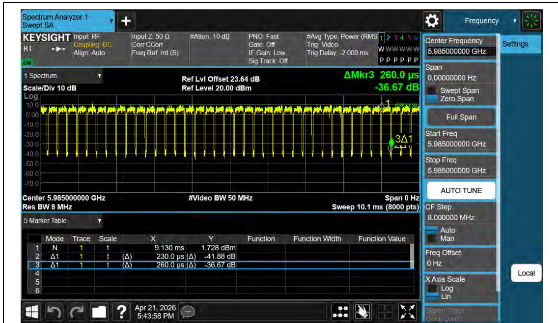
NTNV-11BE80MIMO-Ant2-5985
