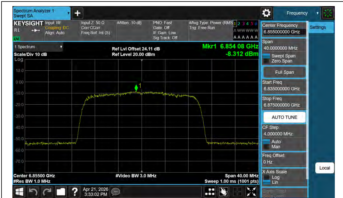
11AX20MIMO-Ant2-6855-PASS
