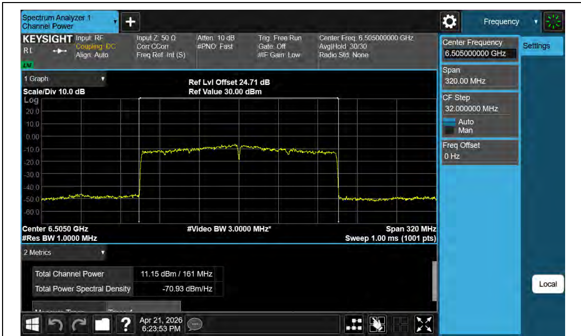
11BE160MIMO-Ant2-6505-PASS
