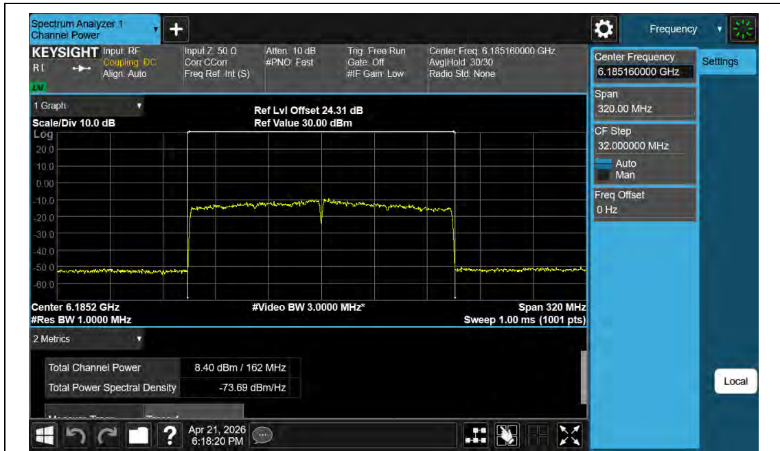
11BE160MIMO-Ant2-6185-PASS
