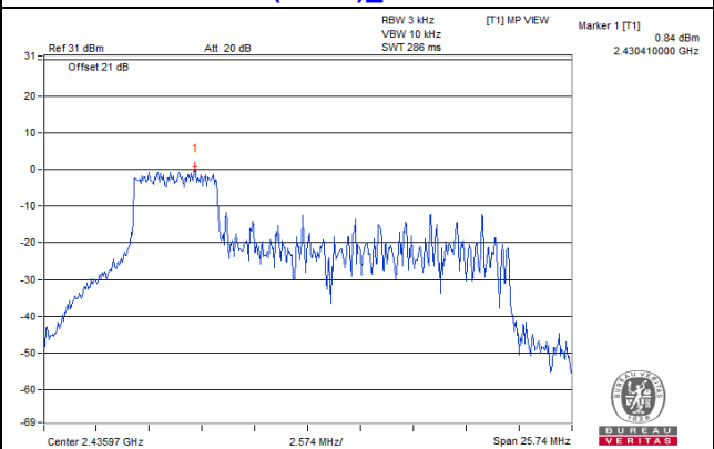
802.11ax (RU52)_Chain 0 / CH6
