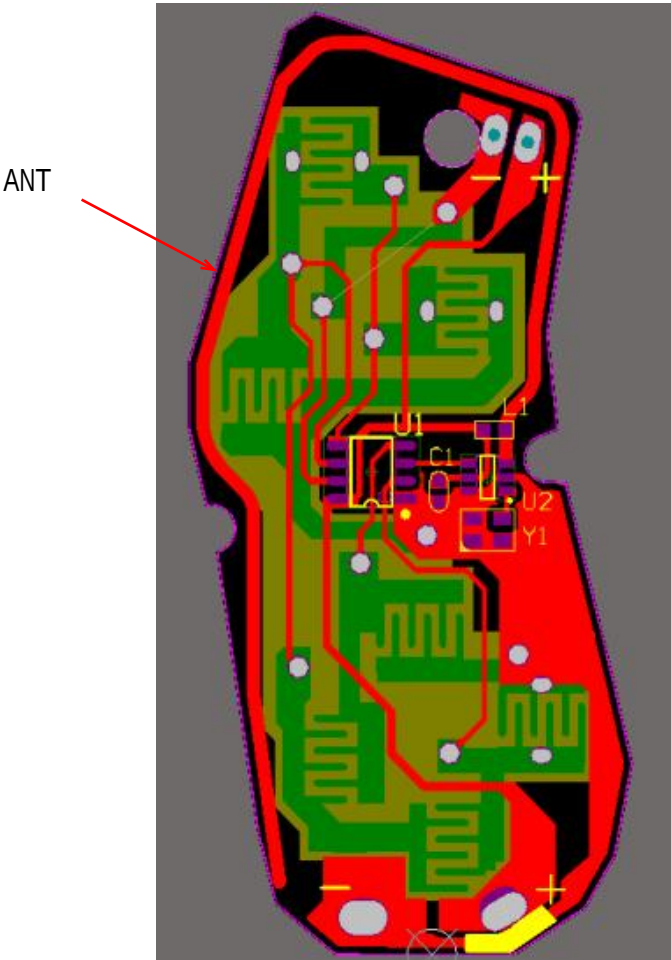
Picture of antenna
