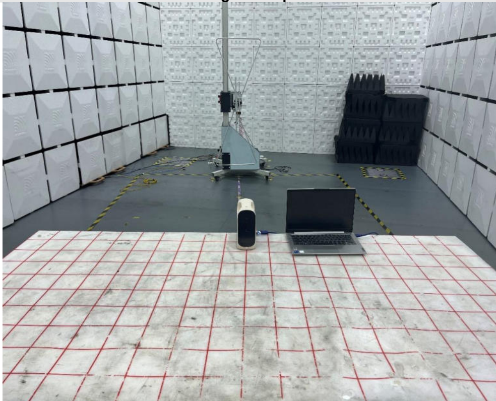
Radiated Band edge and Spurious Emission
