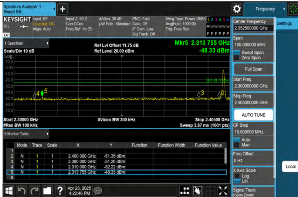
DH5-Ant1-2402-PASS
