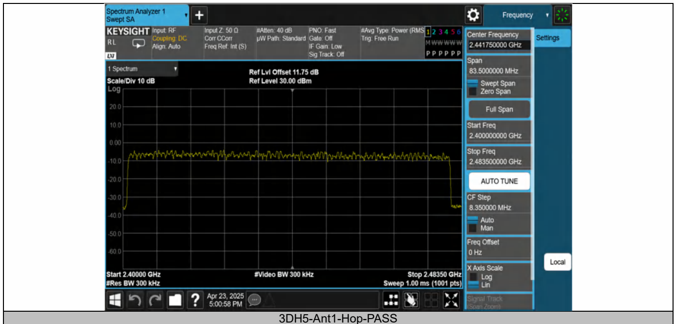
3DH5-Ant1-Hop-PASS
