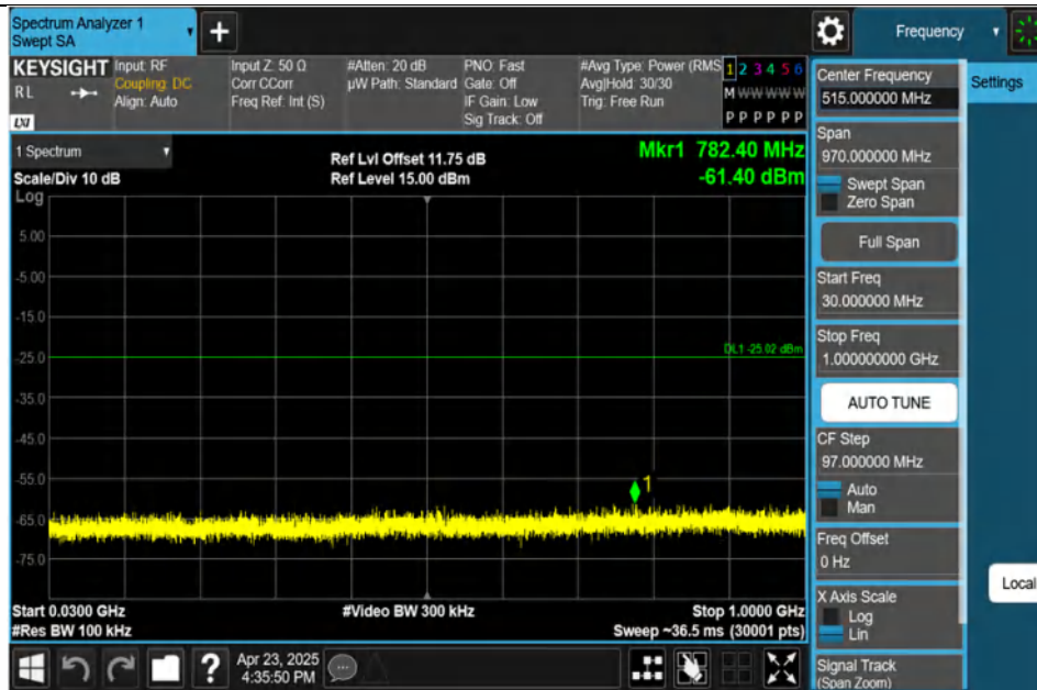
2DH5-Ant1-2402-30~1000-PASS
