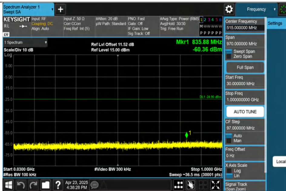
2DH5-Ant1-2441-30~1000-PASS
