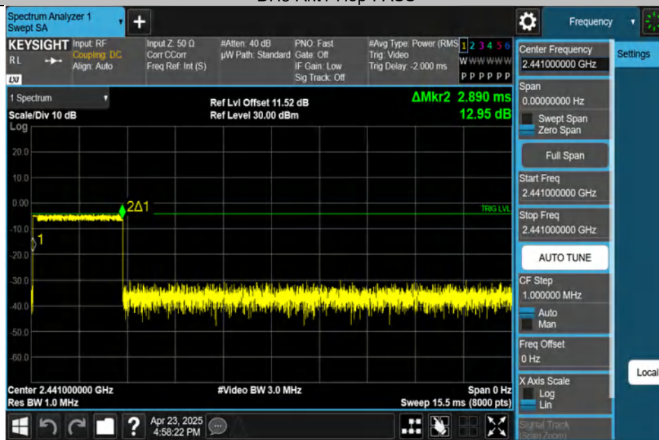
2DH5-Ant1-Hop-PASS
