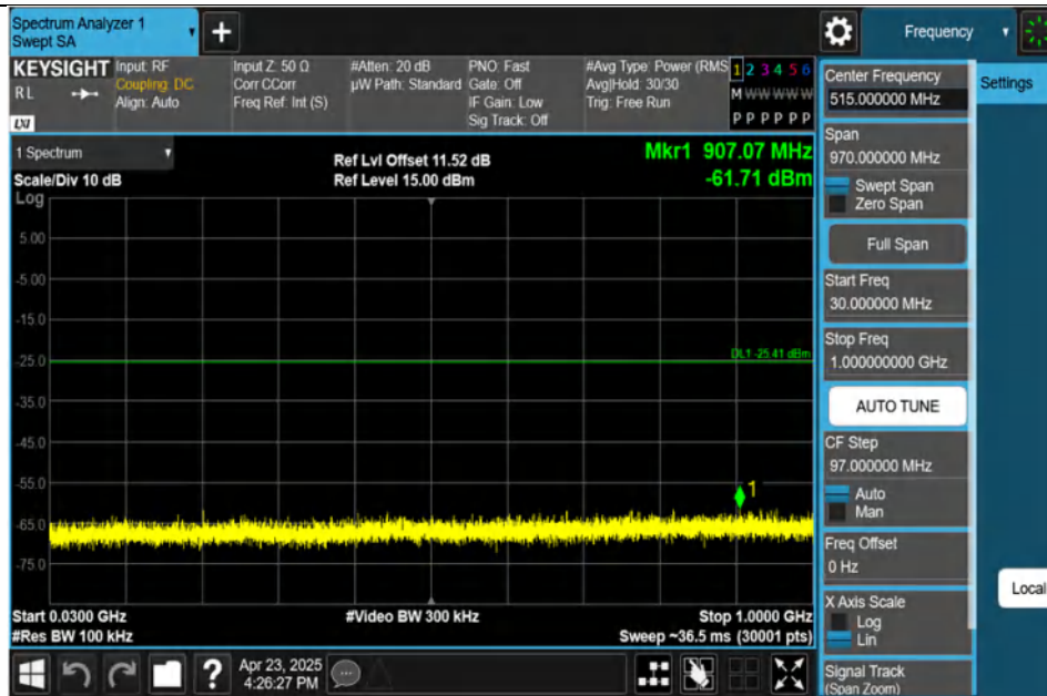
DH5-Ant1-2441-30~1000-PASS
