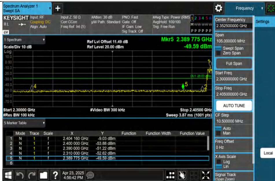
2DH5-Ant1-Hop_2402-PASS
