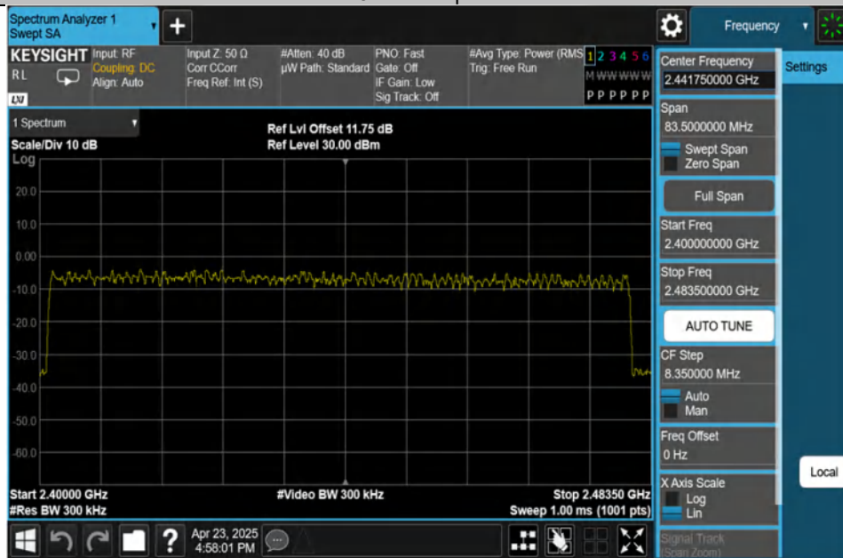
2DH5-Ant1-Hop-PASS
