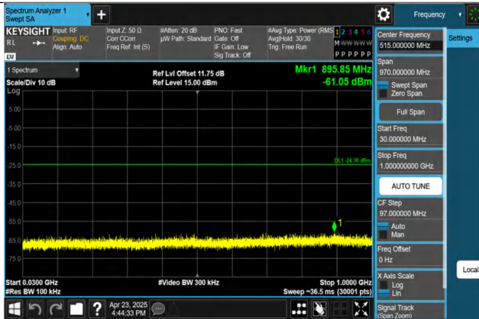
3DH5-Ant1-2402-30~1000-PASS
