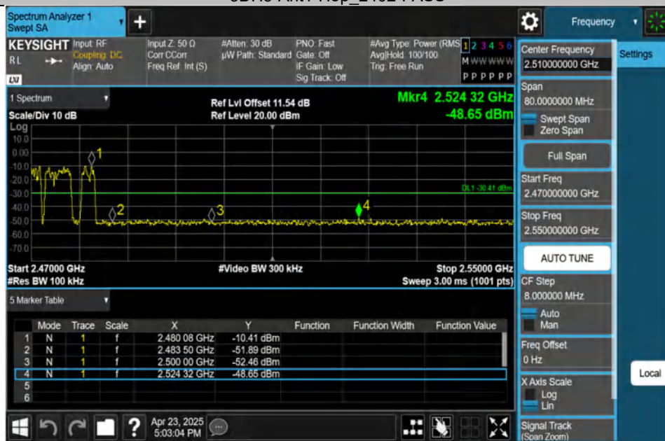
3DH5-Ant1-Hop_2480-PASS
