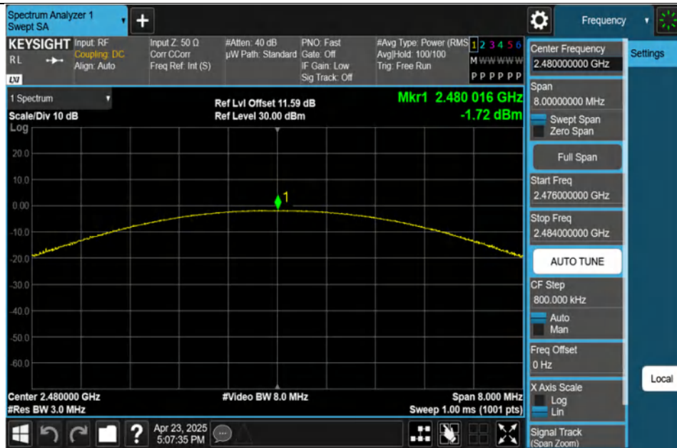
DH5-Ant1-2480-PASS
