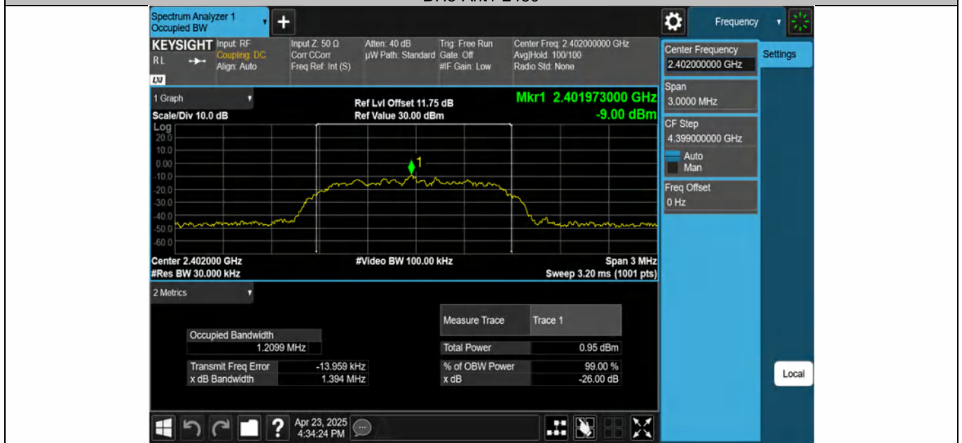
2DH5-Ant1-2402
