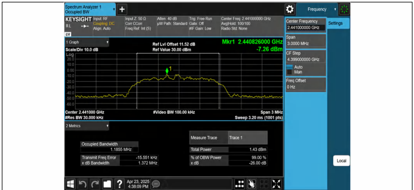
2DH5-Ant1-2441
