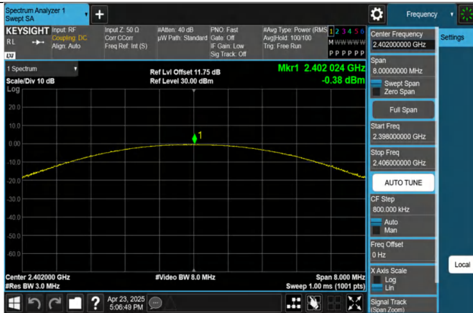
DH5-Ant1-2402-PASS
