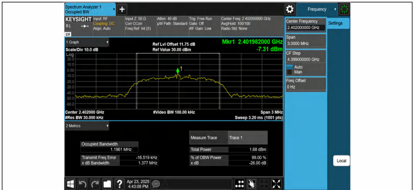
3DH5-Ant1-2402
