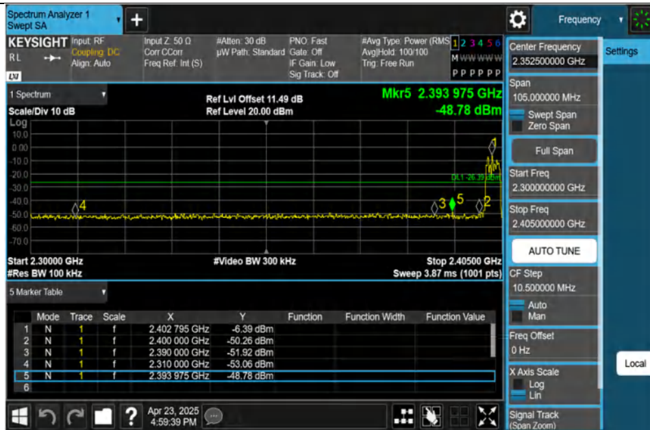
3DH5-Ant1-Hop_2402-PASS
