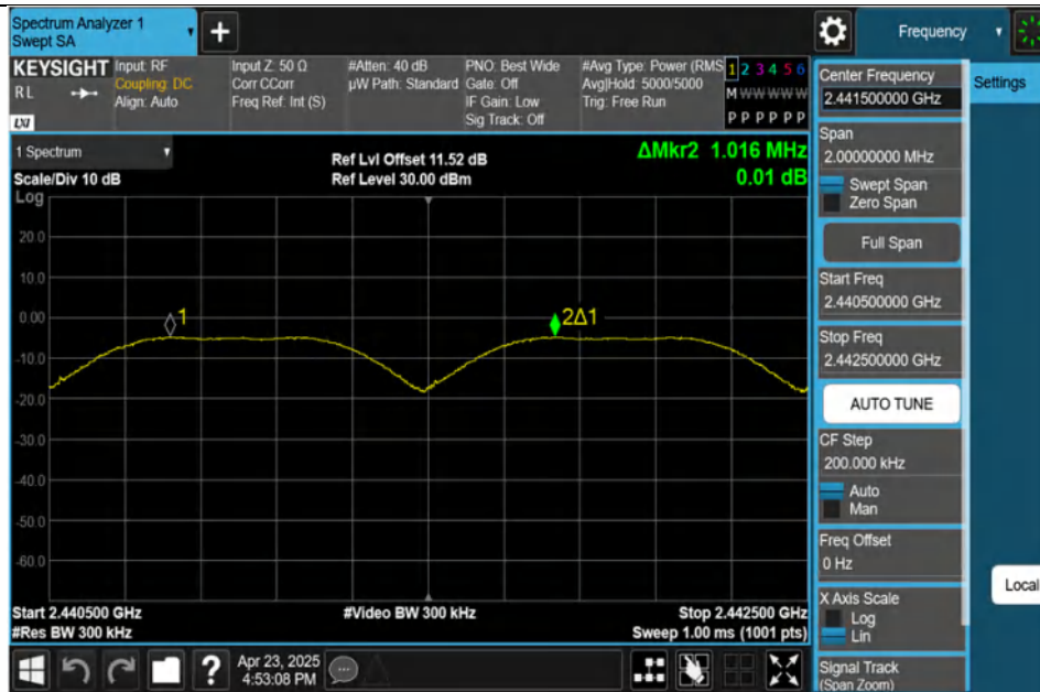
DH5-Ant1-Hop-PASS
