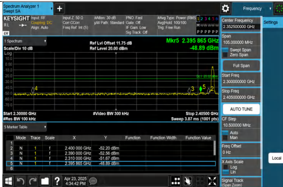
2DH5-Ant1-2402-PASS
