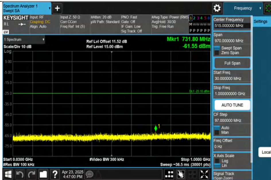
3DH5-Ant1-2441-30~1000-PASS
