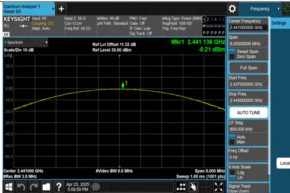
2DH5-Ant1-2441-PASS
