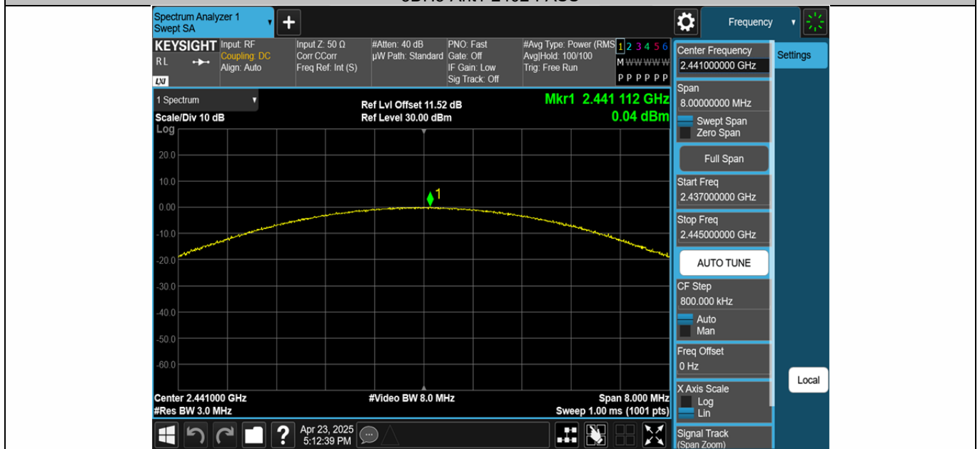
3DH5-Ant1-2441-PASS
