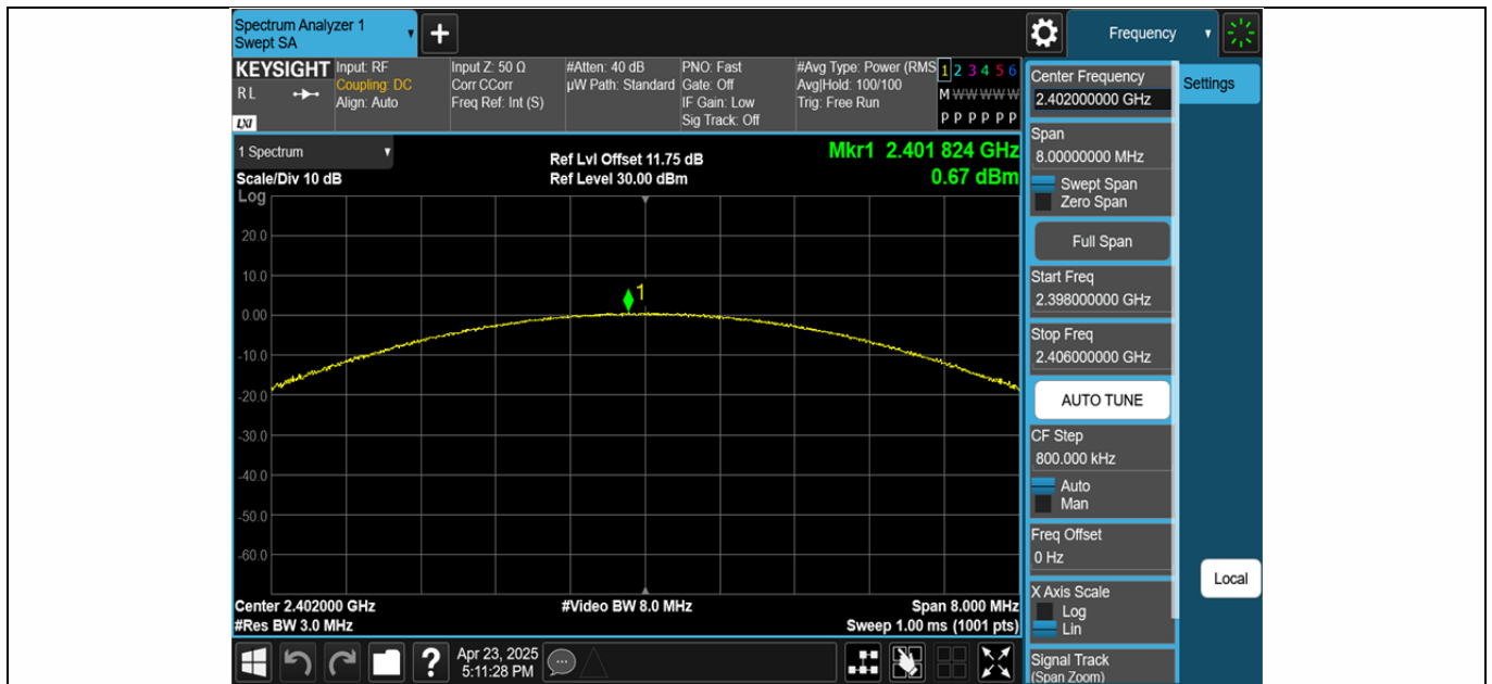
3DH5-Ant1-2402-PASS
