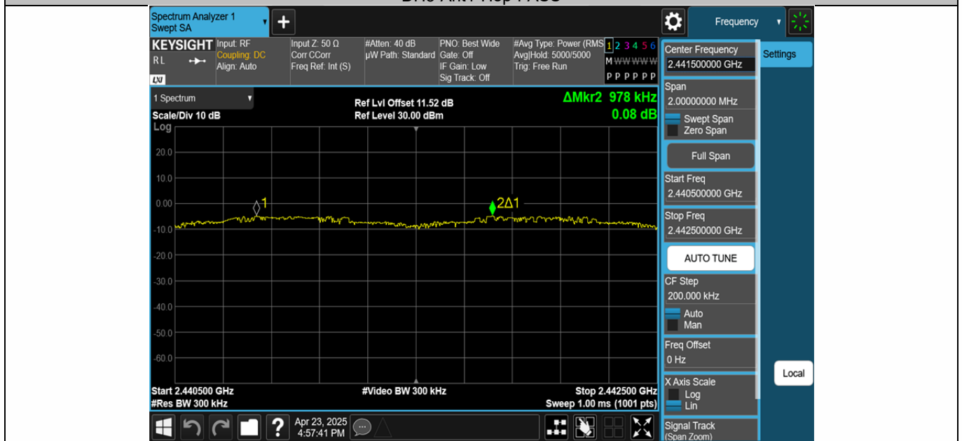
2DH5-Ant1-Hop-PASS
