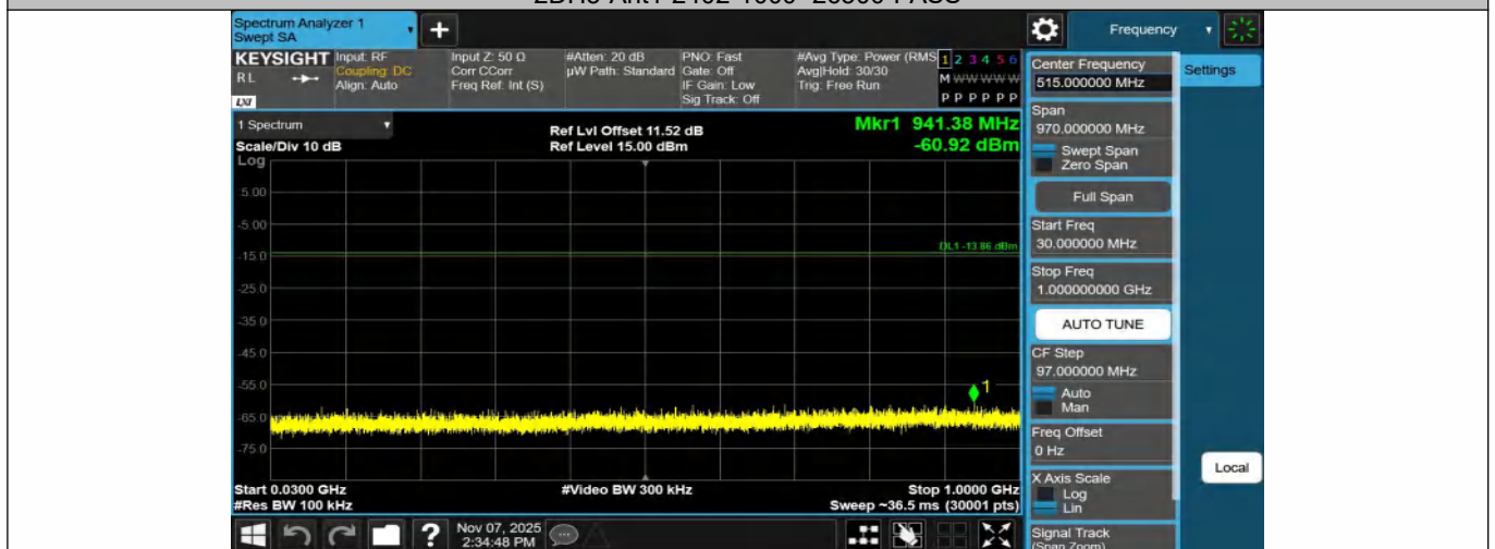
2DH5-Ant1-2441-30~1000-PASS
