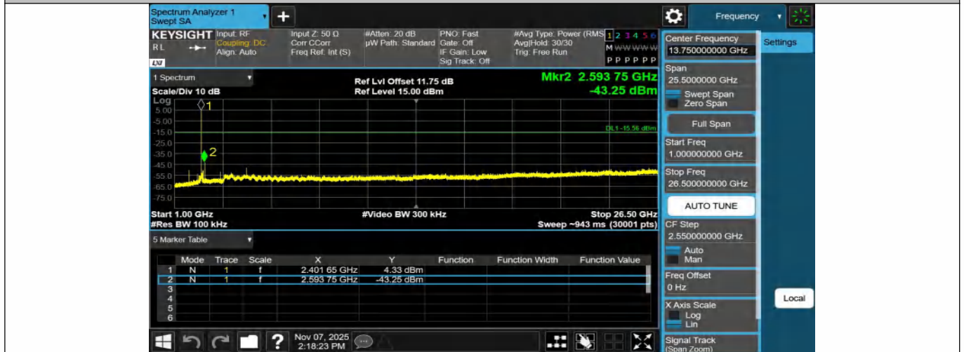
DH5-Ant1-2402-1000~26500-PASS
