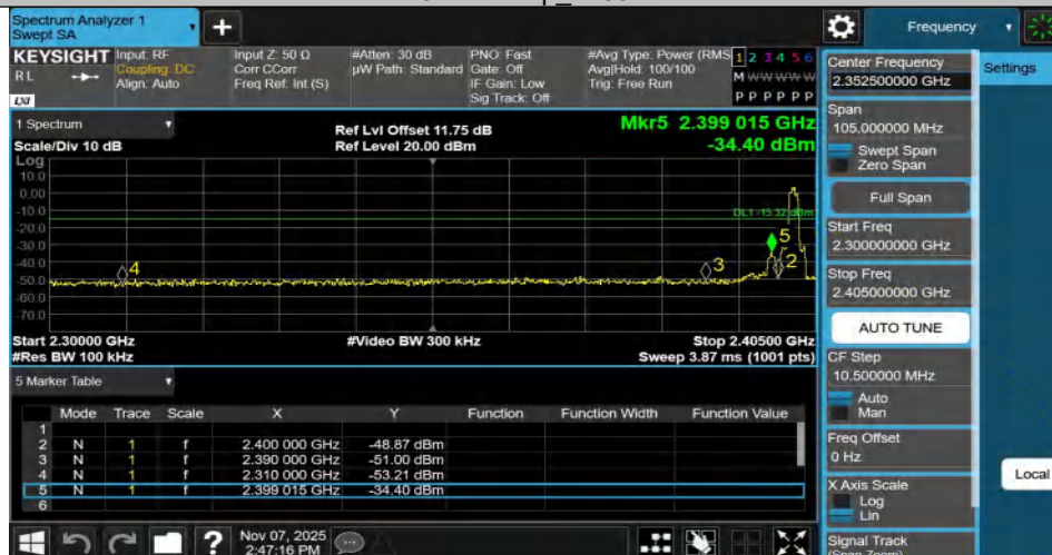
3DH5-Ant1-2402-PASS
