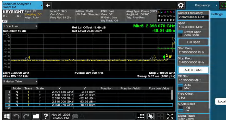
2DH5-Ant1-Hop_2402-PASS
