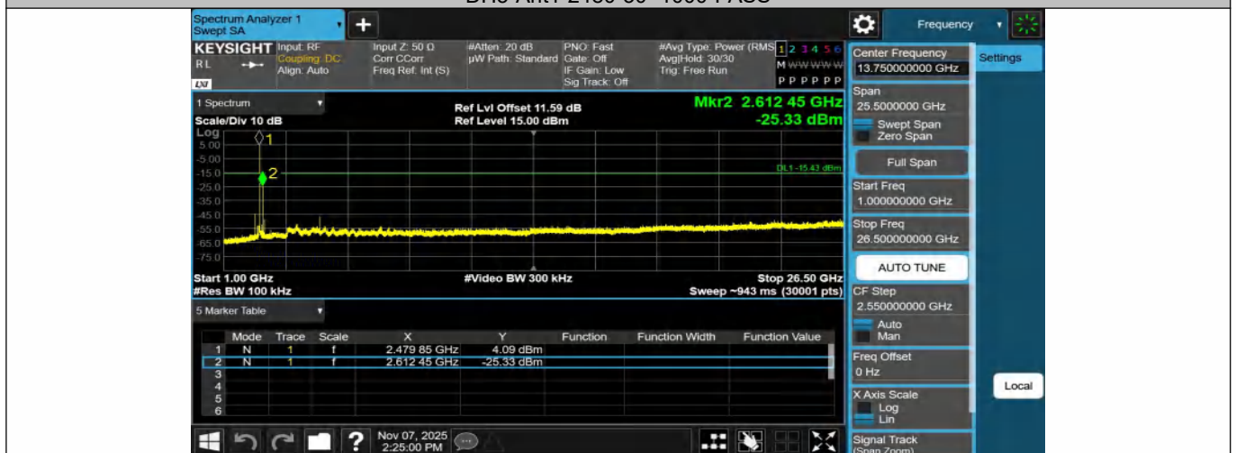
DH5-Ant1-2480-1000~26500-PASS
