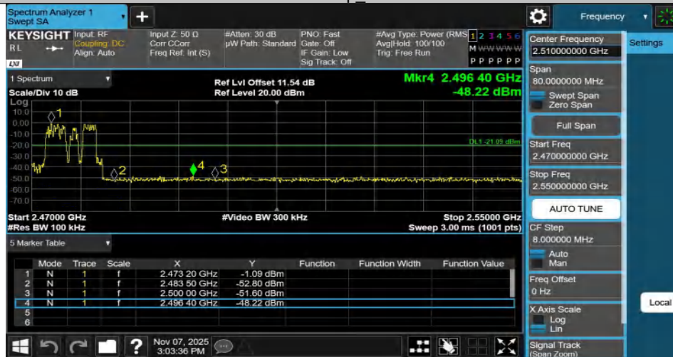
2DH5-Ant1-Hop_2480-PASS
