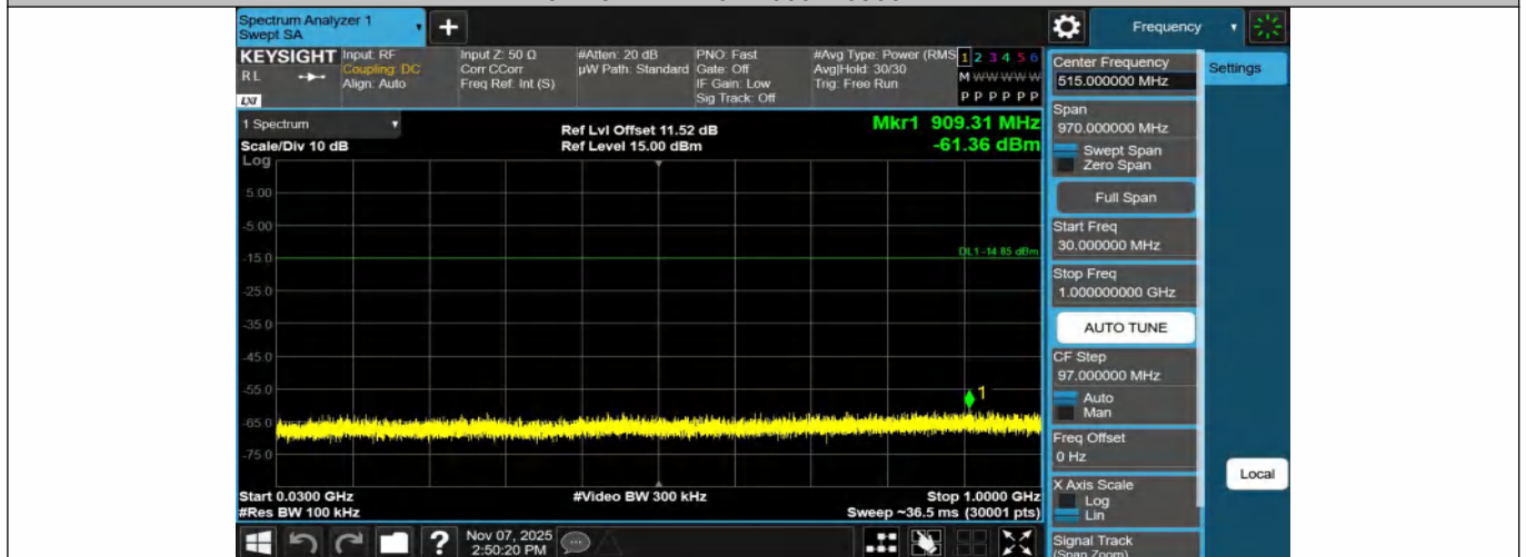
3DH5-Ant1-2441-30~1000-PASS
