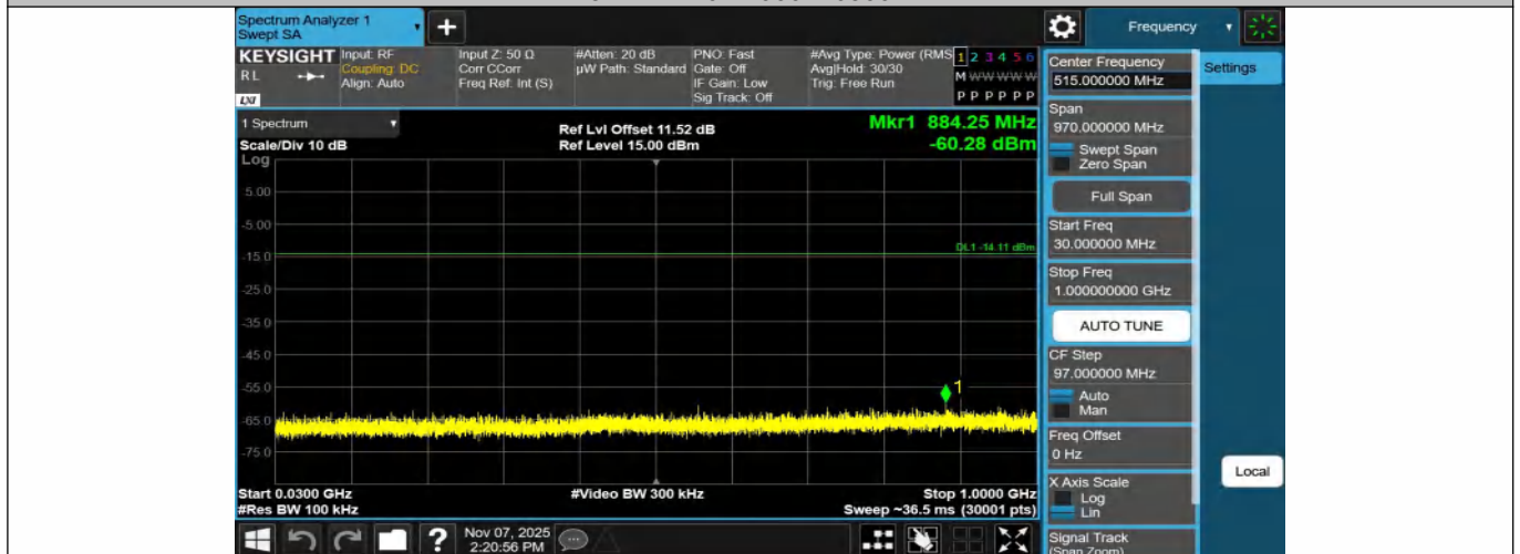
DH5-Ant1-2441-30~1000-PASS
