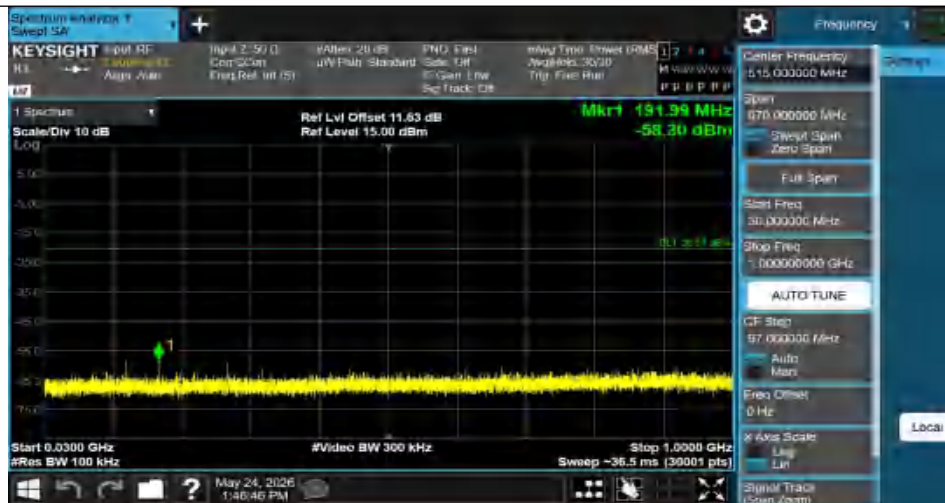
3DH5-Ant1-2402-30~1000-PASS
