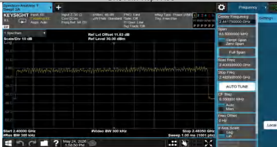
2DH5-Ant1-Hop-PASS
