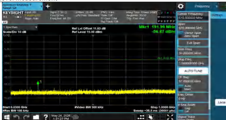
DH5-Ant1-2402-30~1000-PASS
