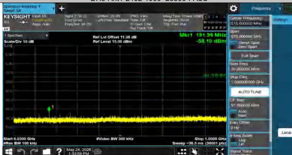
DH5-Ant1-2441-30~1000-PASS
