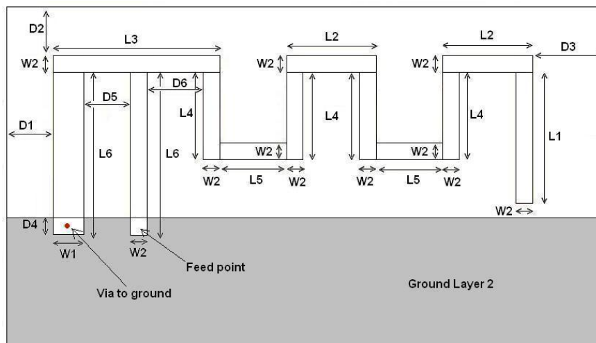
Figure 3: Antenna Dimensions
