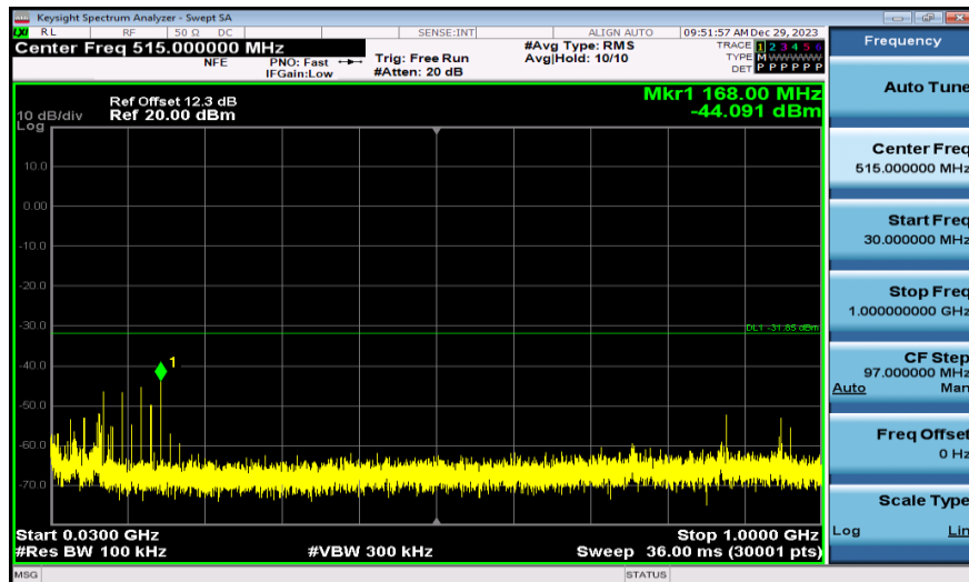
11N40SISO-Ant1-2452-30~1000-PASS
