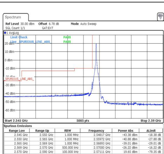
Band38_20MHz_16QAM_37850_1RB#0
