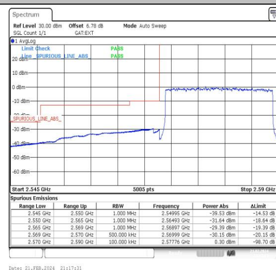
Band38_20MHz_16QAM_37850_100RB#0
