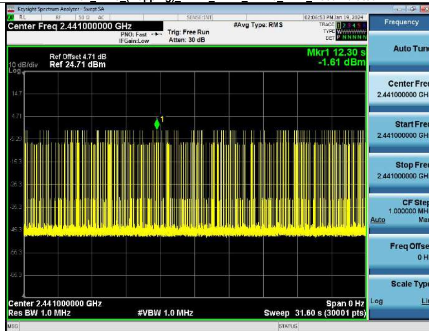
Dwell_Time_(Hopping)_NVNT_ANT1_2-DH5_2441_Accumulated
