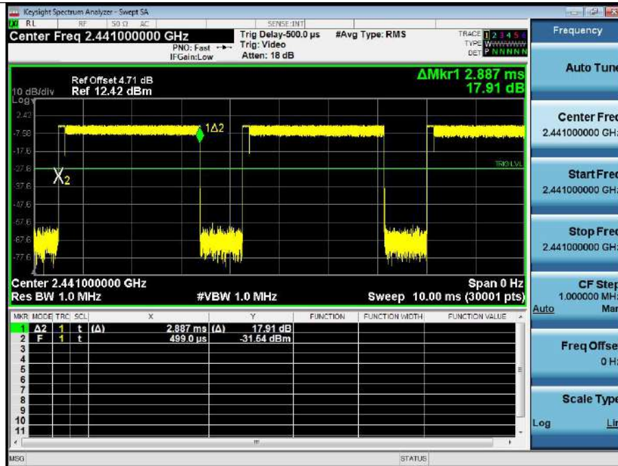
Dwell_Time_(Hopping)_NVNT_ANT1_2-DH5_2441_Accumulated
