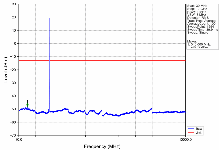
Band2_RMC_MCH_1880MHz_12.2kbps RMC_NTNV
