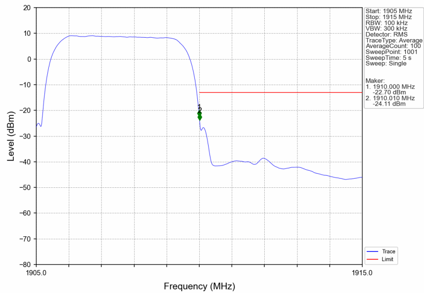
Band2_RMC_HCH_1907.6MHz_12.2kbps RMC_NTNV
