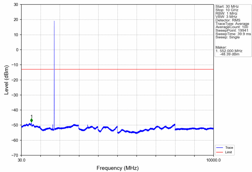
Band4_RMC_MCH_1732.6MHz_12.2kbps RMC_NTNV
