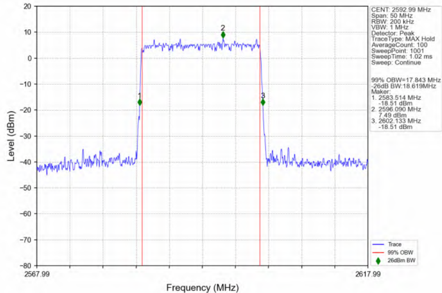
n41_30kHz_SISO_NTNV_20MHz_CP-OFDM QPSK_2592.99MHz_Outer_Full_Ant1
