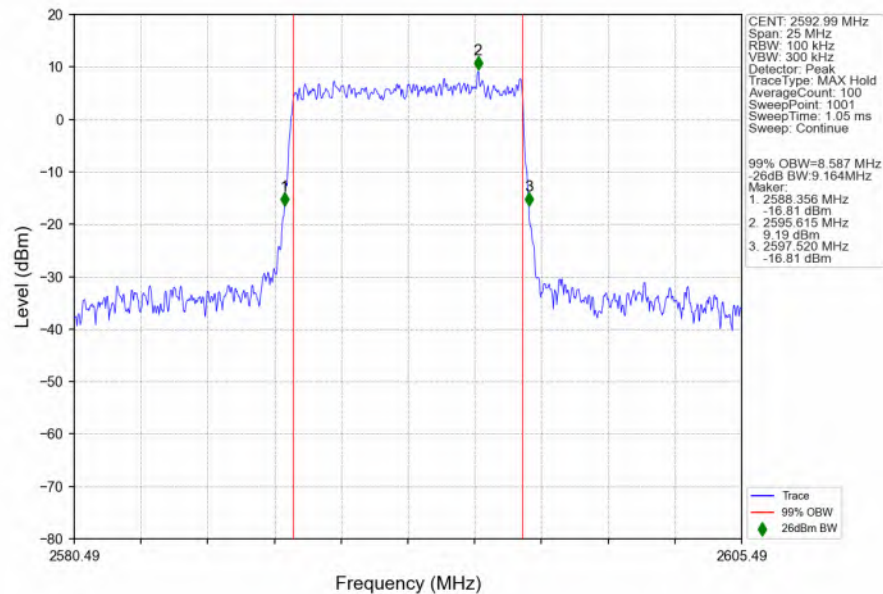
n41_30kHz_SISO_NTNV_10MHz_CP-OFDM 64 QAM_2592.99MHz_Outer_Full_Ant1
