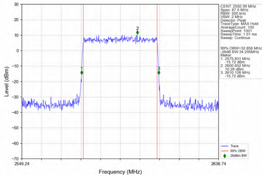
n41_30kHz_SISO_NTNV_35MHz_CP-OFDM_64_QAM_2592.99MHz_Outer_Full_Ant1
