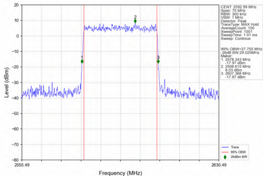
n41_30kHz_SISO_NTNV_30MHz_CP-OFDM 64 QAM_2592.99MHz_Outer_Full_Ant1
