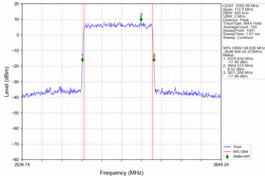
n41_30kHz_SISO_NTNV_45MHz_CP-OFDM QPSK_2592.99MHz_Outer_Full_Ant1
