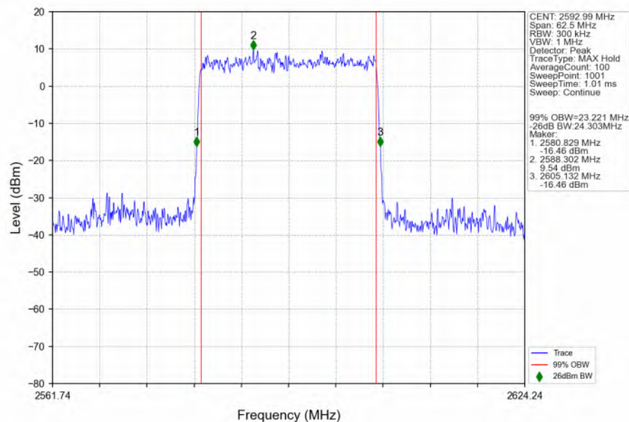
n41_30kHz_SISO_NTNV_25MHz_CP-OFDM QPSK_2592.99MHz_Outer_Full_Ant1
