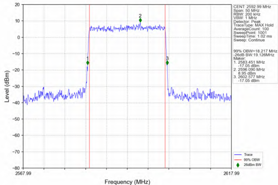
n41_30kHz_SISO_NTNV_20MHz_CP-OFDM QPSK_2592.99MHz_Outer_Full_Ant1
