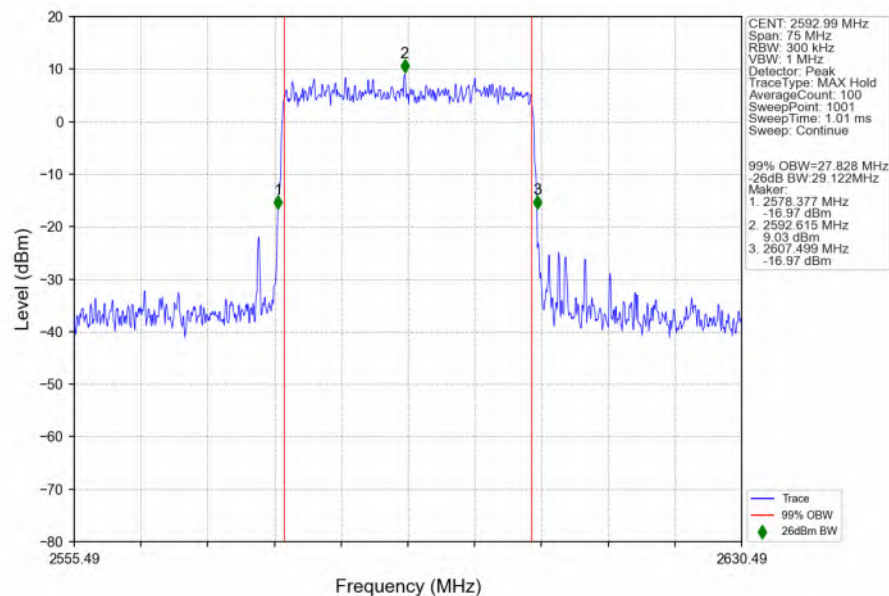
n41_30kHz_SISO_NTNV_30MHz_CP-OFDM QPSK 2592.99MHz_Outer_Full_Ant1
