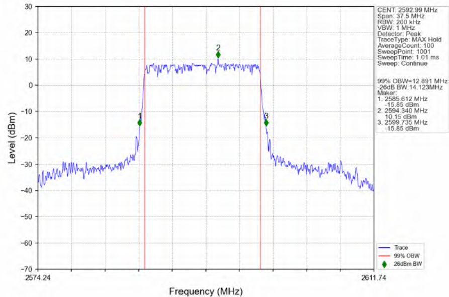
n41_30kHz_SISO_NTNV_15MHz_DFT-s-OFDM_64_QAM_2592.99MHz_Outer_Full_Ant1
