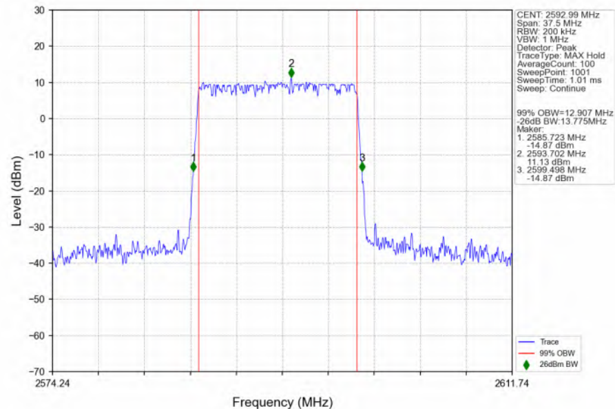
n41_30kHz_SISO_NTNV_15MHz_DFT-s-OFDM_64_QAM_2592.99MHz_Outer_Full_Ant1
