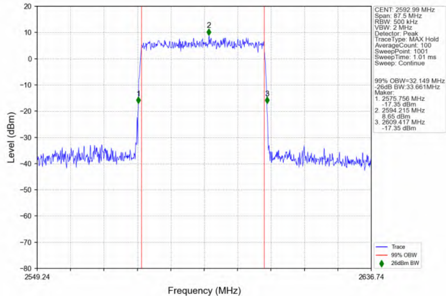
n41_30kHz_SISO_NTNV_35MHz_CP-OFDM QPSK 2592.99MHz_Outer_Full_Ant1
