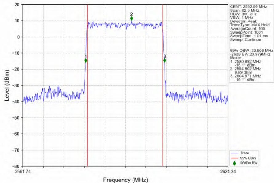
n41_30kHz_SISO_NTNV_25MHz_DFT-s-OFDM_64_QAM_2592.99MHz_Outer_Full_Ant1
