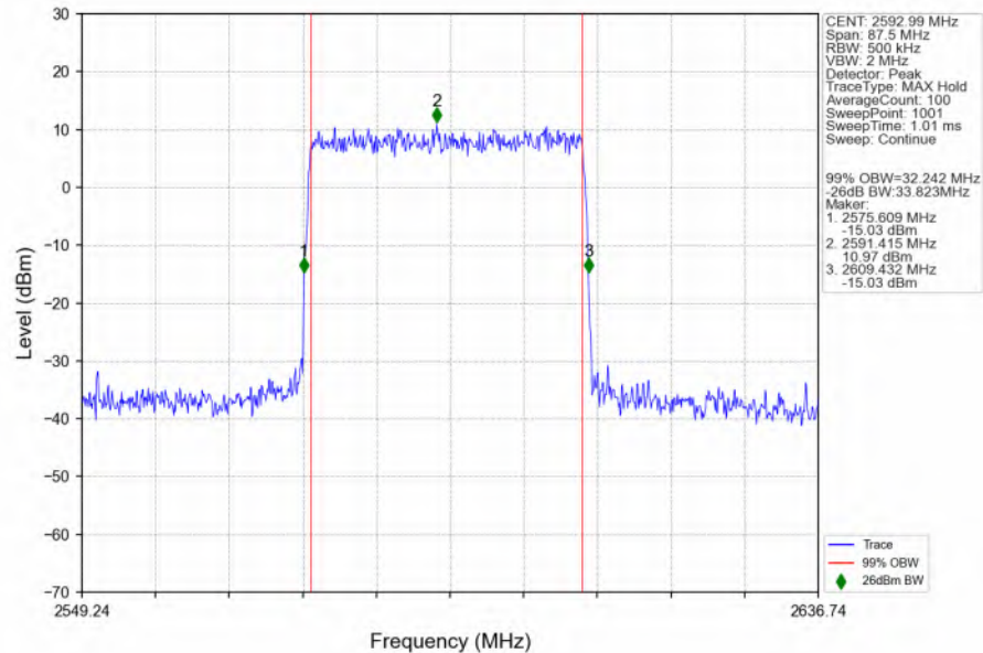
n41_30kHz_SISO_NTNV_35MHz_DFT-s-OFDM_64_QAM_2592.99MHz_Outer_Full_Ant1
