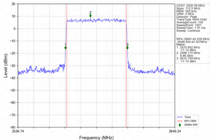
n41_30kHz_SISO_NTNV_45MHz_CP-OFDM_64_QAM_2592.99MHz_Outer_Full_Ant1
