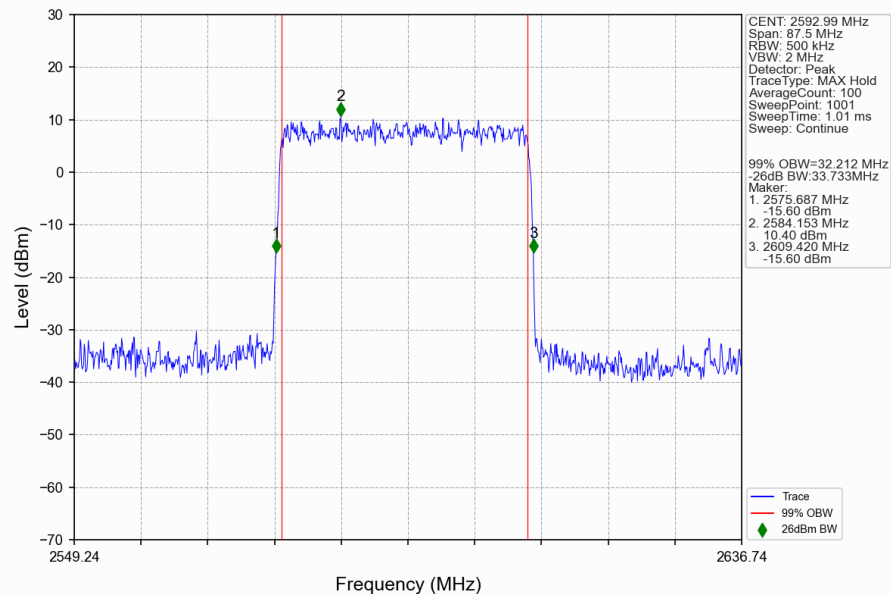
n41_30kHz_SISO_NTNV_35MHz_DFT-s-OFDM_64_QAM_2592.99MHz_Outer_Full_Ant1
