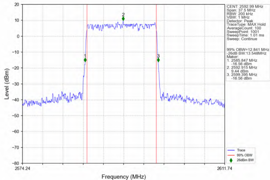
n41_30kHz_SISO_NTNV_15MHz_CP-OFDM QPSK 2592.99MHz_Outer_Full_Ant1
