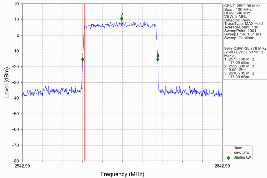
n41_30kHz_SISO_NTNV_40MHz_CP-OFDM QPSK 2592.99MHz_Outer_Full_Ant1
