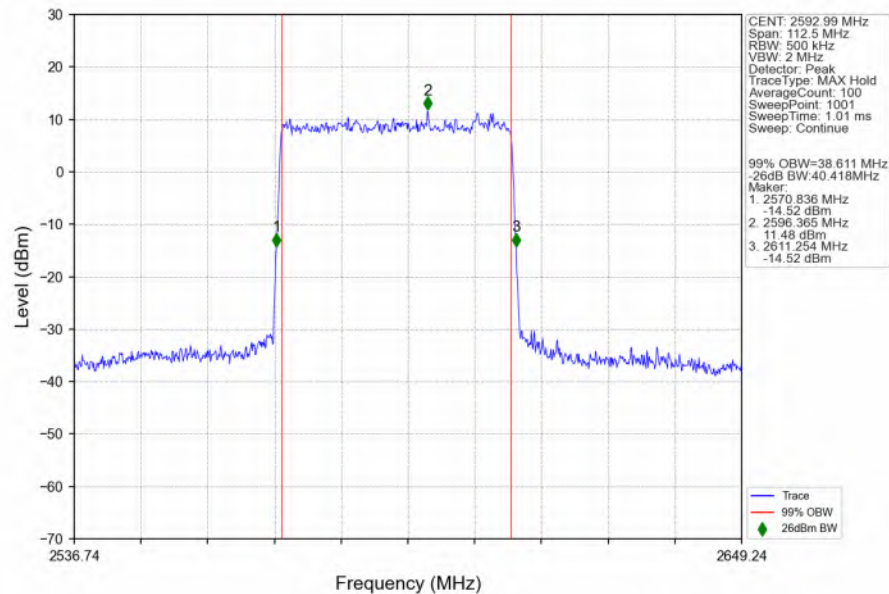
n41_30kHz_SISO_NTNV_45MHz_DFT-s-OFDM 64 QAM_2592.99MHz_Outer_Full_Ant1
