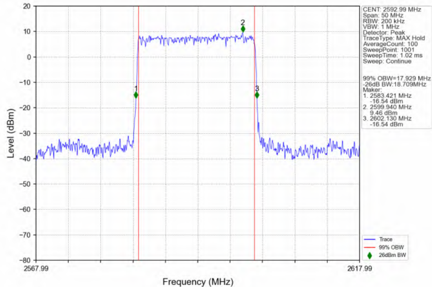
n41_30kHz_SISO_NTNV_20MHz_DFT-s-OFDM_64_QAM_2592.99MHz_Outer_Full_Ant1
