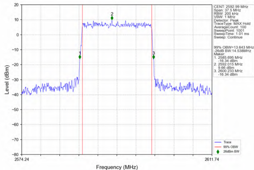
n41_30kHz_SISO_NTNV_15MHz_CP-OFDM 64 QAM_2592.99MHz_Outer_Full_Ant1
