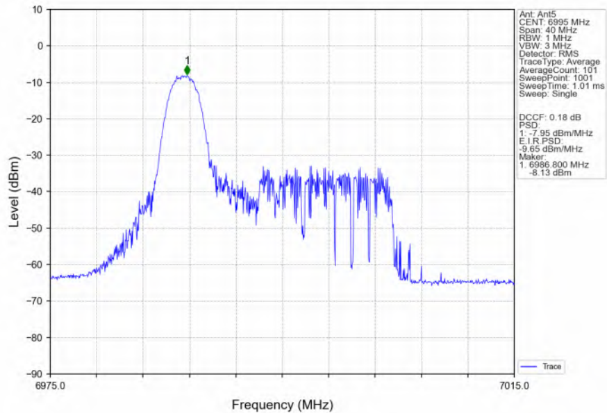
802.11ax(HEW20)_MCH_6995MHz_RU26_Left_MIMO_NTNV
