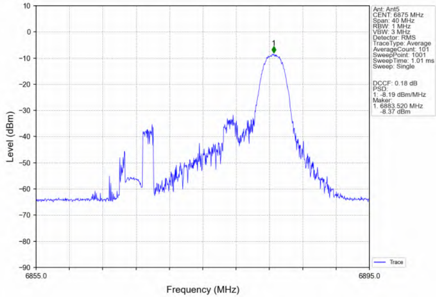
802.11ax(HEW20)_HCH_6875MHz_RU26_Left_MIMO_NTNV
