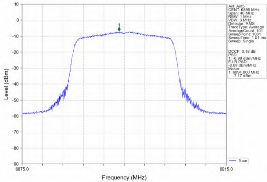
802.11ax(HEW20)_LCH_6895MHz_SU / Ant5_NTNV
