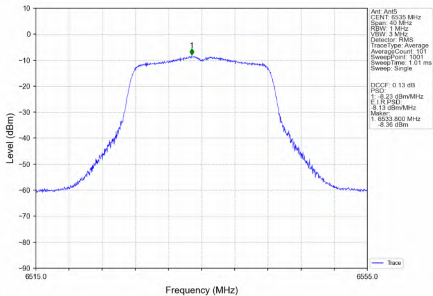
802.11a_LCH_6535MHz_Ant5_NTNV
