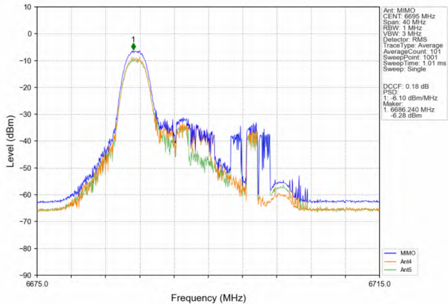
802.11ax(HEW20)_MCH_6695MHz_RU26_Left_MIMO_NTNV
