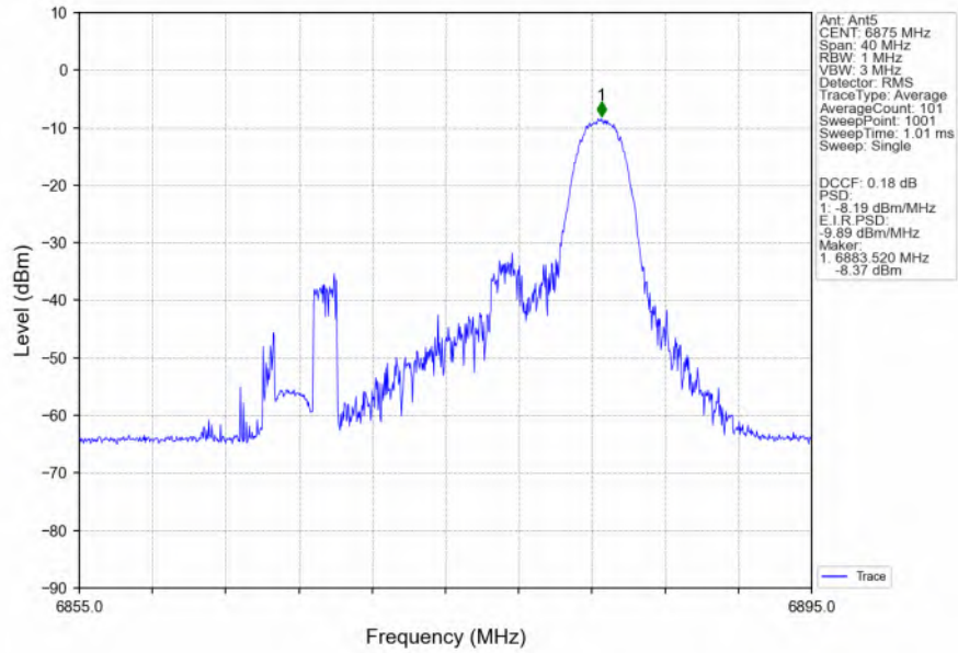
802.11ax(HEW20) HCH 6875MHz RU26 Left MIMO_NTNV
