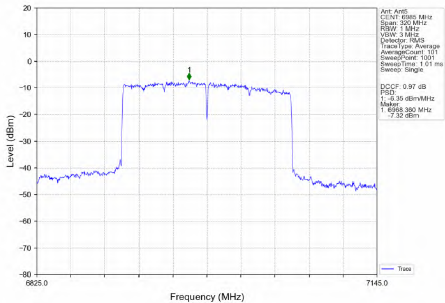
802.11ax(HEW160)_MCH_6985MHz_SU / _Ant5_NTNV
