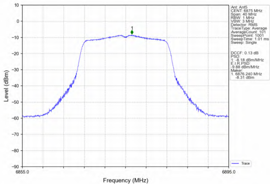
802.11a_HCH_6875MHz_Ant5_NTNV
