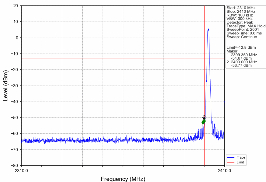
1M_LCH_2402MHz_Ant4_NTNV
