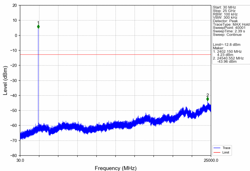
1M_LCH_2402MHz_Ant4_NTNV
