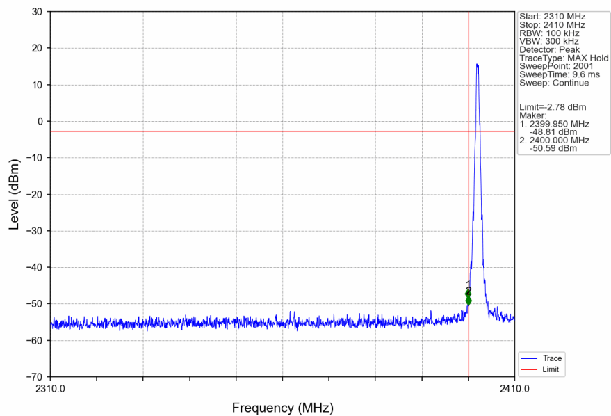
GFSK DH5 LCH 2402MHz Ant4 NTN
