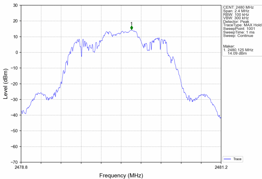
Pi/4DQPSK_2DH5_HCH_2480MHz_Ant4_NTNV
