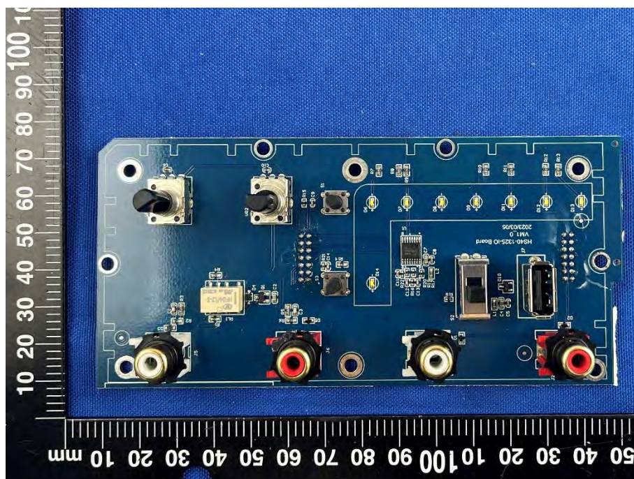
SECONDARY BOARD 8 TOP VIEW
