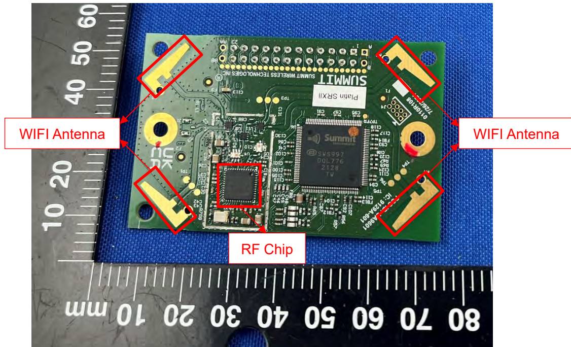
SECONDARY BOARD 7 TOP VIEW (WITHOUT SHIELDING)
