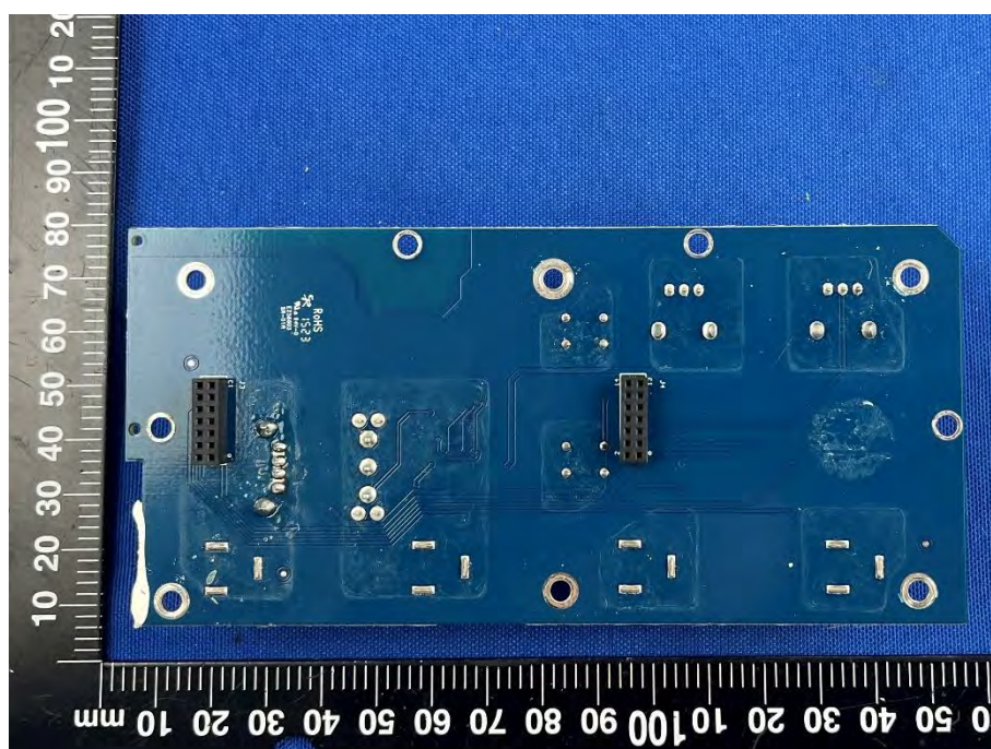
SECONDARY BOARD 8 REAR VIEW
