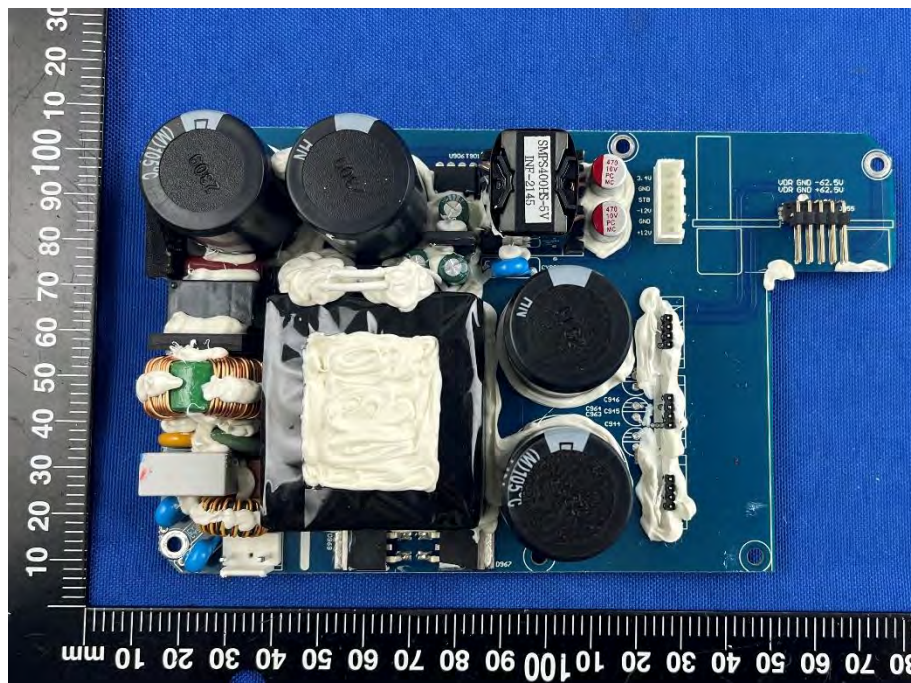
SECONDARY BOARD 9 TOP VIEW
