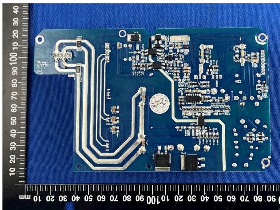
SECONDARY BOARD 9 REAR VIEW
