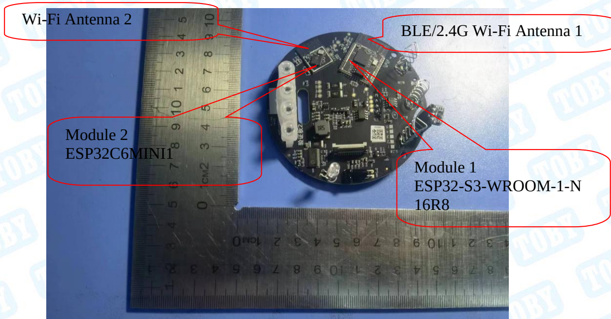
Photo 13 Appearance of PCB
