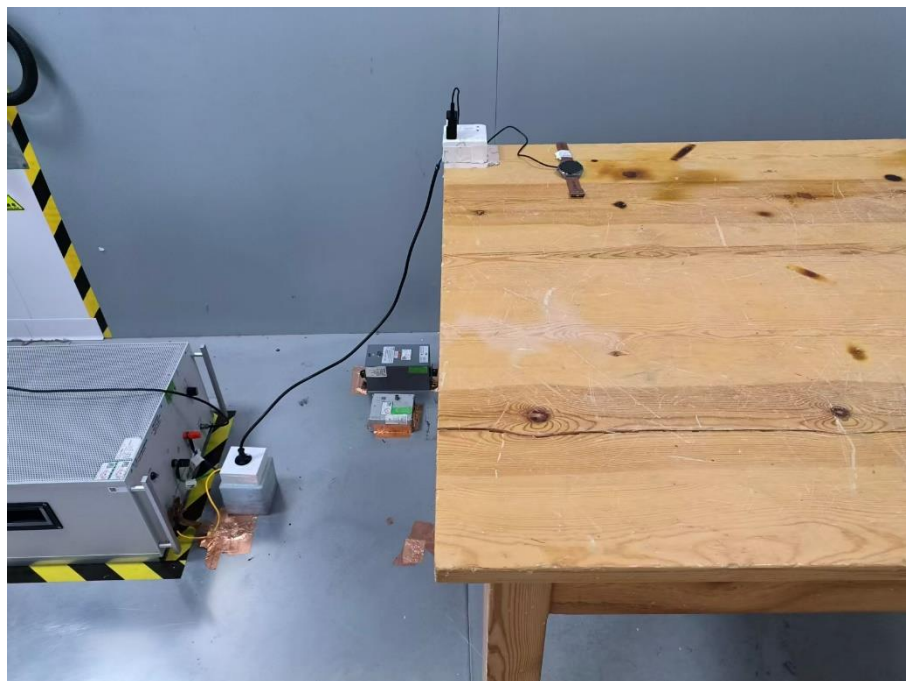
Set-up for Conducted Emission
