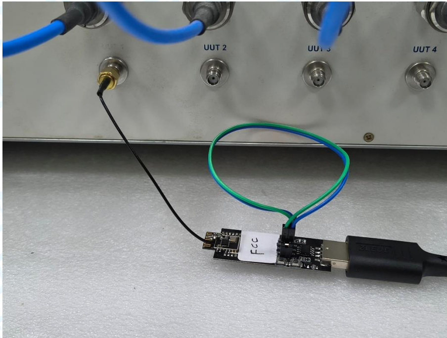
Photo of Setup for Conducted Measurement
