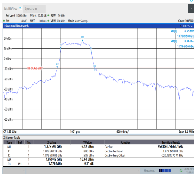
Band2-3MHz-16QAM-18900-PASS
