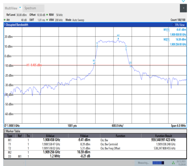
Band2-3MHz-16QAM-19185-PASS
