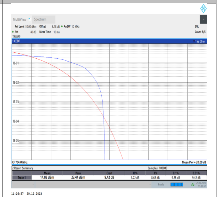
Band12-10MHz-16QAM-23060-PASS
