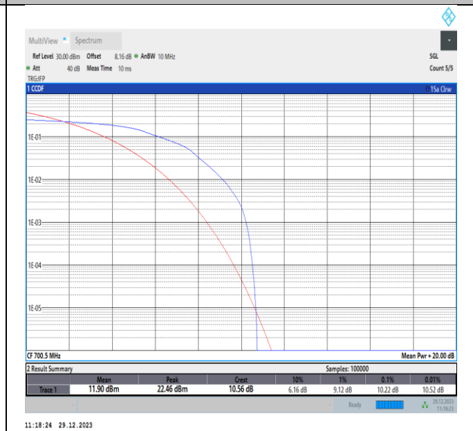
Band12-3MHz-16QAM-23025-PASS
