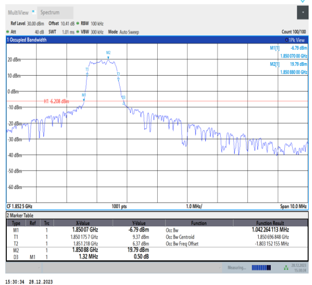
Band2-5MHz-16QAM-18625-PASS
