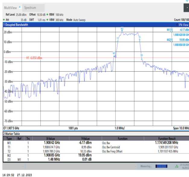
Band2-5MHz-QPSK-19175-PASS
