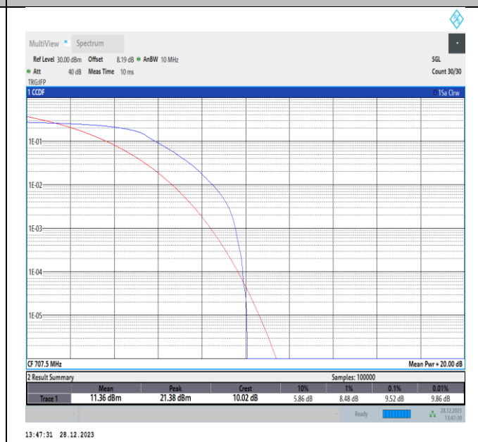
Band12-1.4MHz-QPSK-23095-PASS
