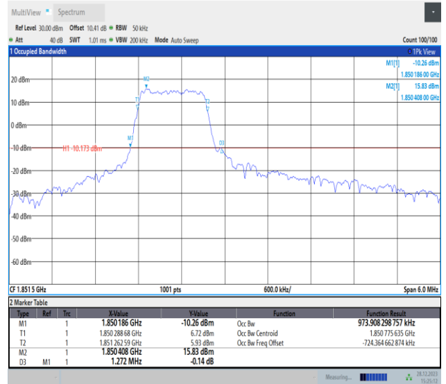
Band2-3MHz-16QAM-18615-PASS
