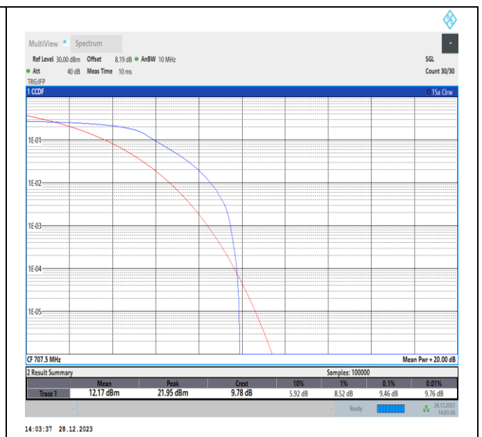
Band12-10MHz-QPSK-23095-PASS
