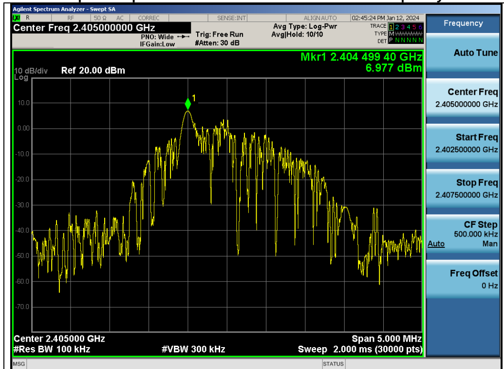
Test_Graph_ANT1_2405_Reference Level
