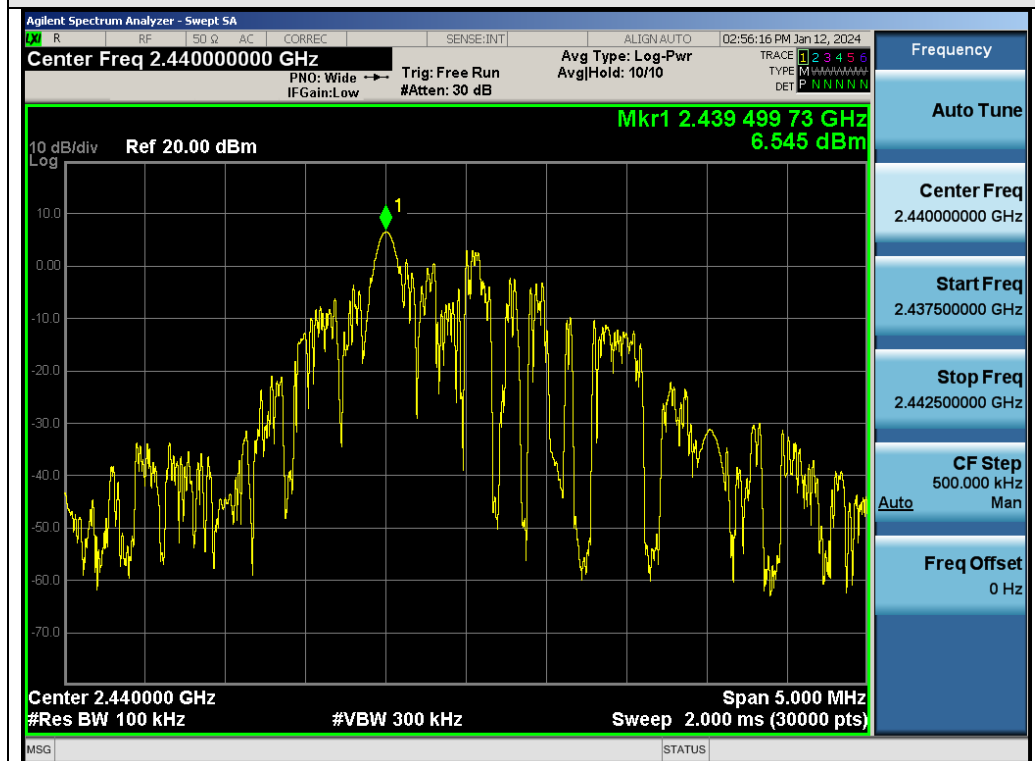
Test_Graph_ANT1_2440_Reference Level
