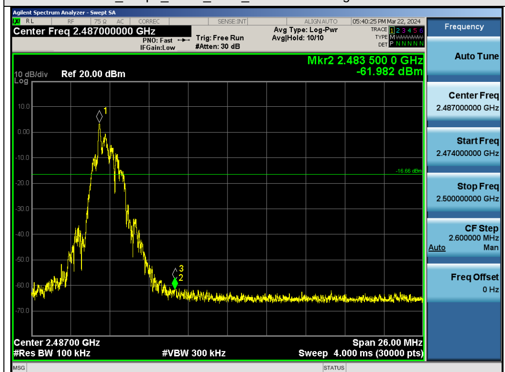
Test_Graph_ANT1_2479_Higher Band Edge Emissions
