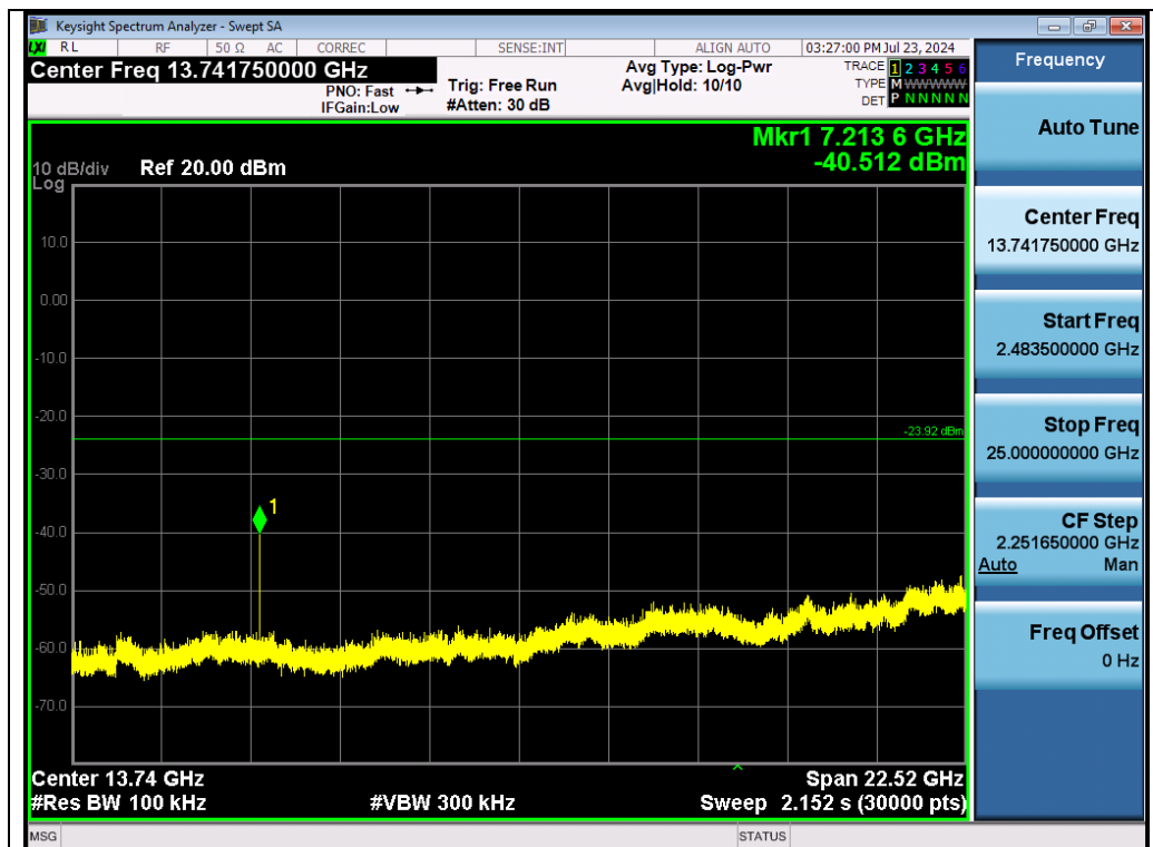
Test_Graph_2.4G_ANT1_2405_GFSK_Higher Band Emissions
