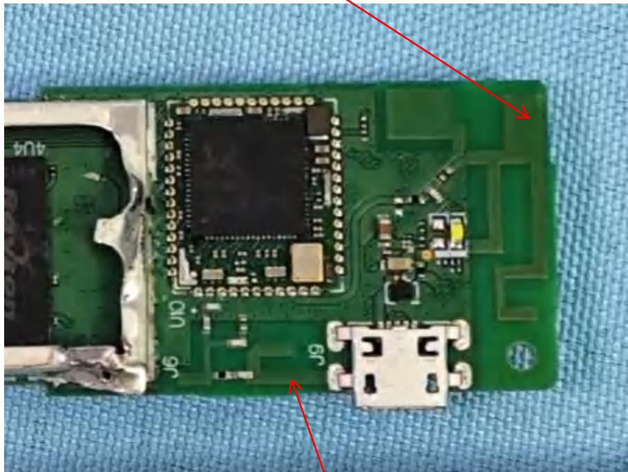
(TV stick) BT&WiFi-ANT2
