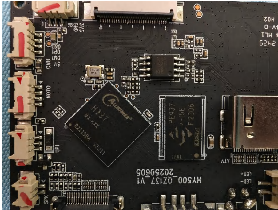
(Mainboard) BT-ANT
