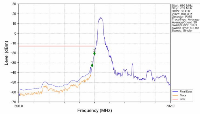
Band12_3MHz_QPSK_LCH_700.5MHz_RB_1_0_NTNV
