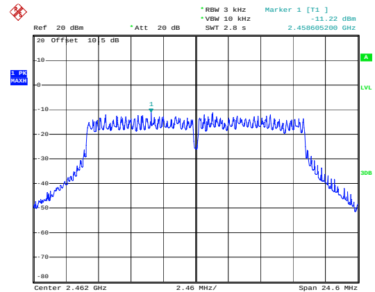
g_2462MHz_Chain 0
