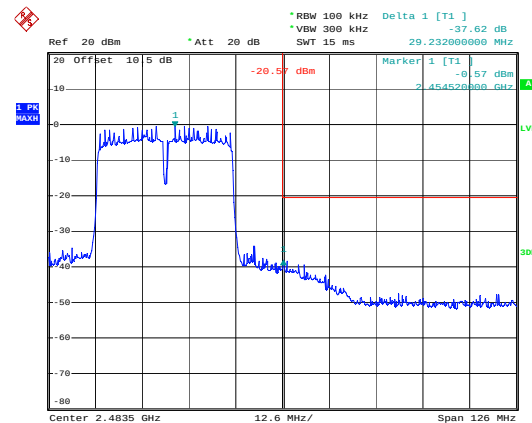
n40_2452MHz_Chain 0
