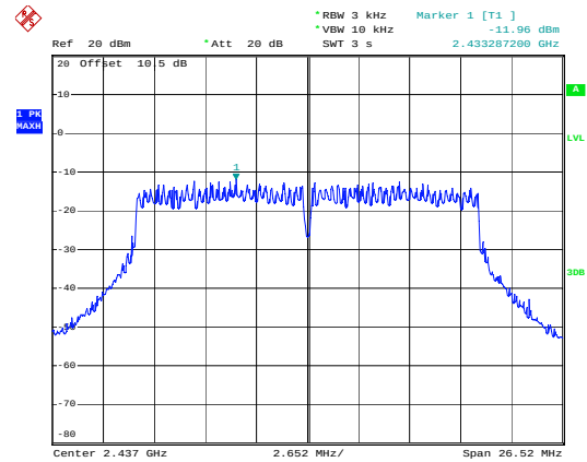
n20_2437MHz_Chain 0
