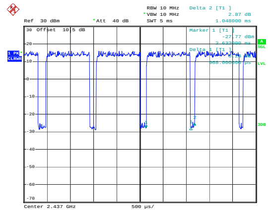
n40_2437MHz_Chain 0
