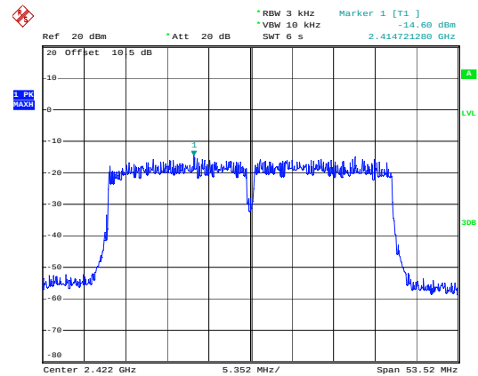
n40_2422MHz_Chain 0
