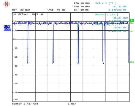
g_2437MHz_Chain 0
