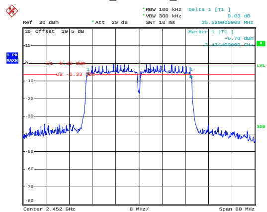
n40_2452MHz_Chain 0
