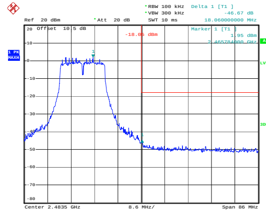
g_2462MHz_Chain 0
