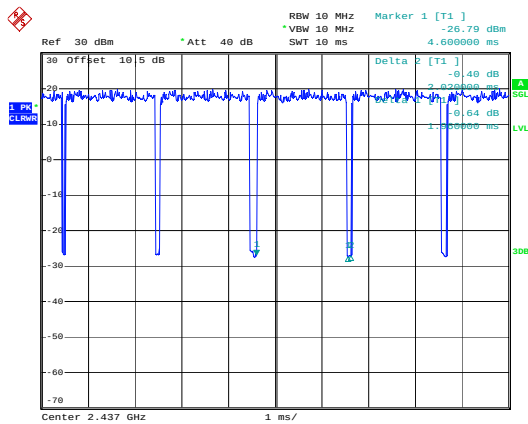
n20_2437MHz_Chain 0
