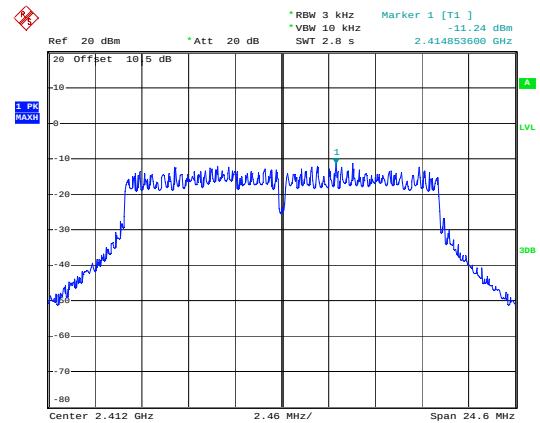
g_2412MHz_Chain 0
