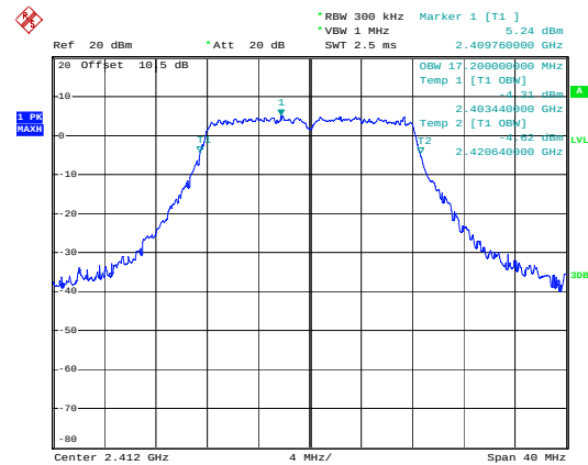
g_2412MHz_Chain 0
