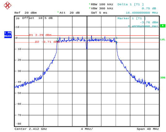
g_2412MHz_Chain 0
