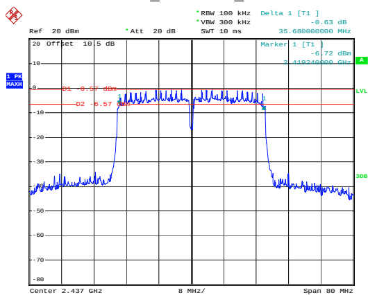
n40_2437MHz_Chain 0
