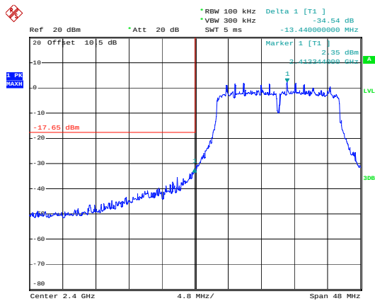
n20_2412MHz_Chain 0
