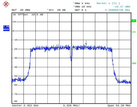
n40_2452MHz_Chain 0
