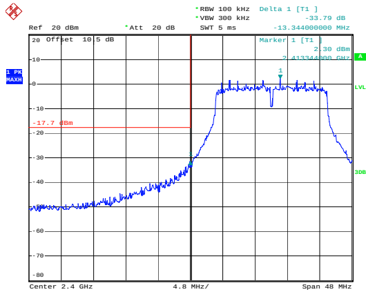
g_2412MHz_Chain 0
