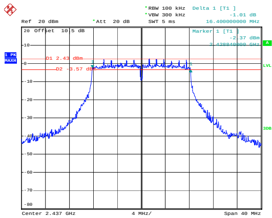
g_2437MHz_Chain 0
