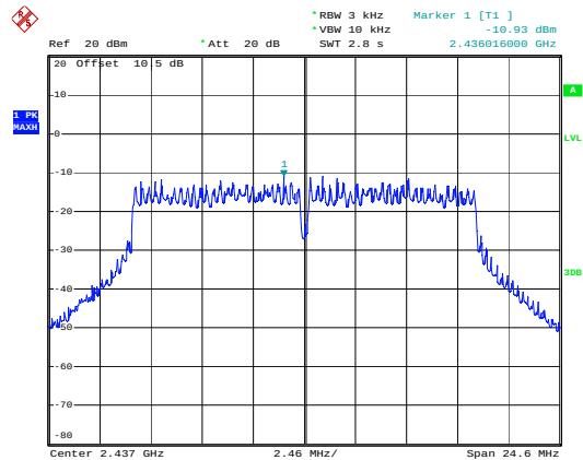
g_2437MHz_Chain 0
