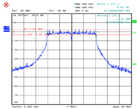
g_2462MHz_Chain 0
