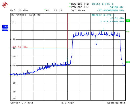
n40_2422MHz_Chain 0
