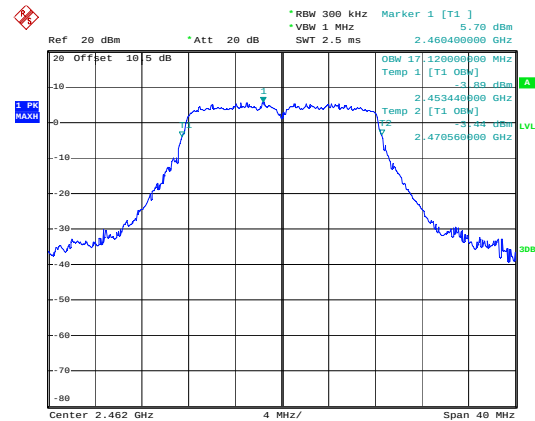
g_2462MHz_Chain 0
