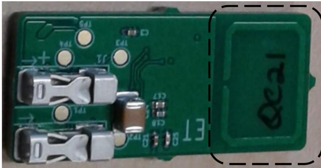
915 MHz tuned loop antenna
