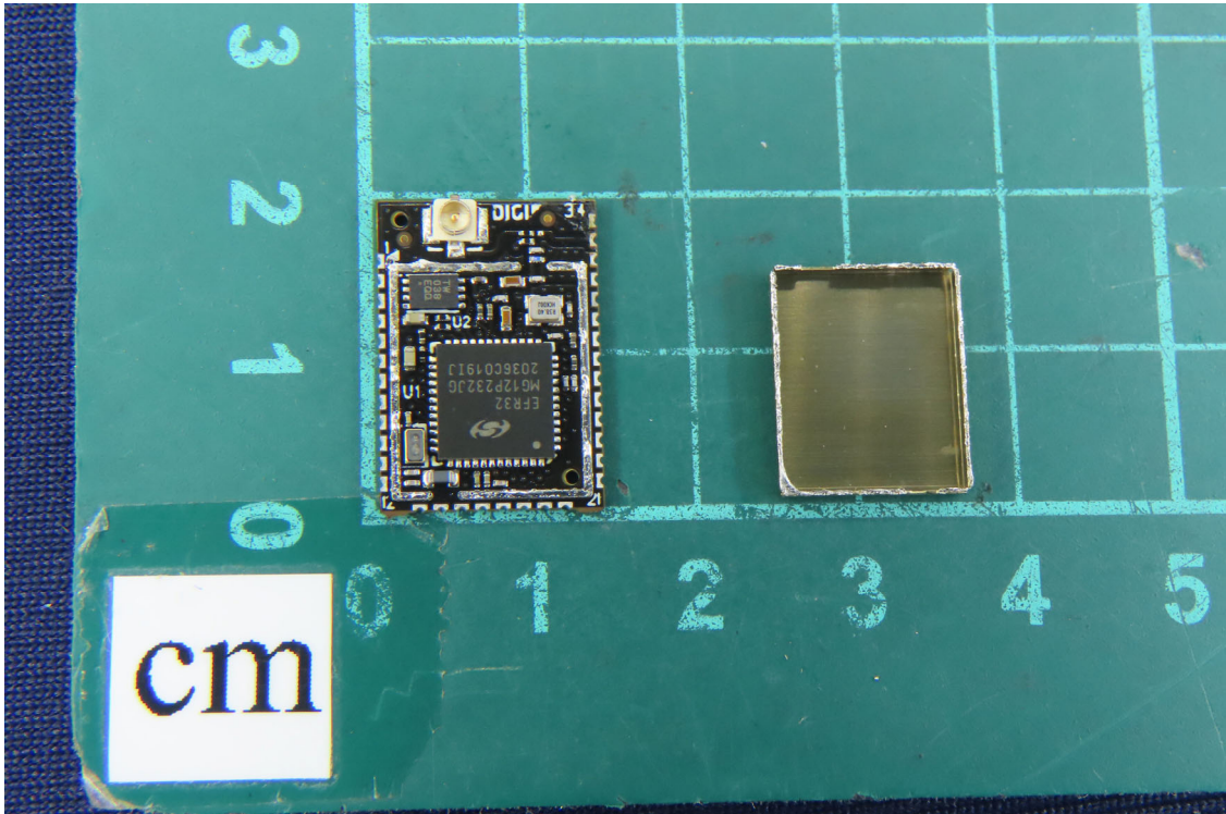
(20)EUT Photo
