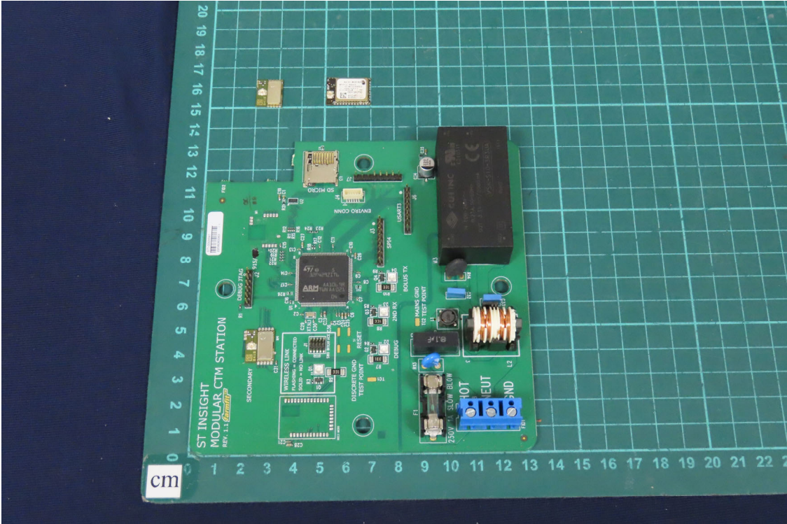
(14)EUT Photo
