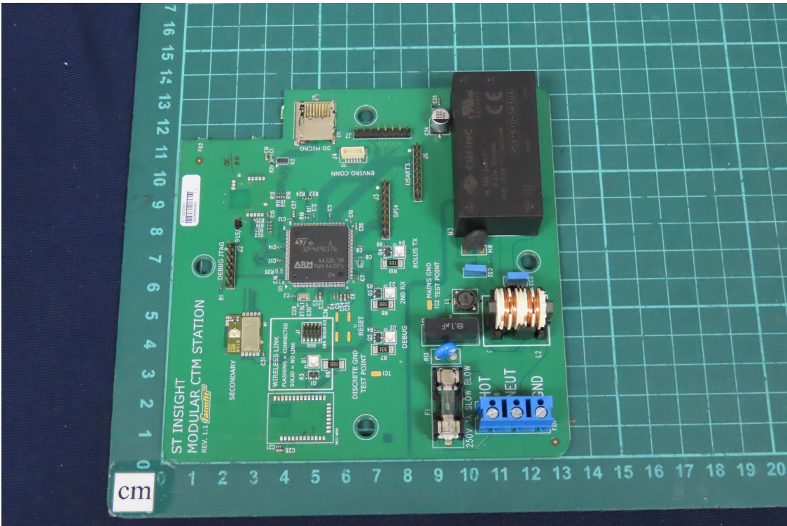
(23)EUT Photo
