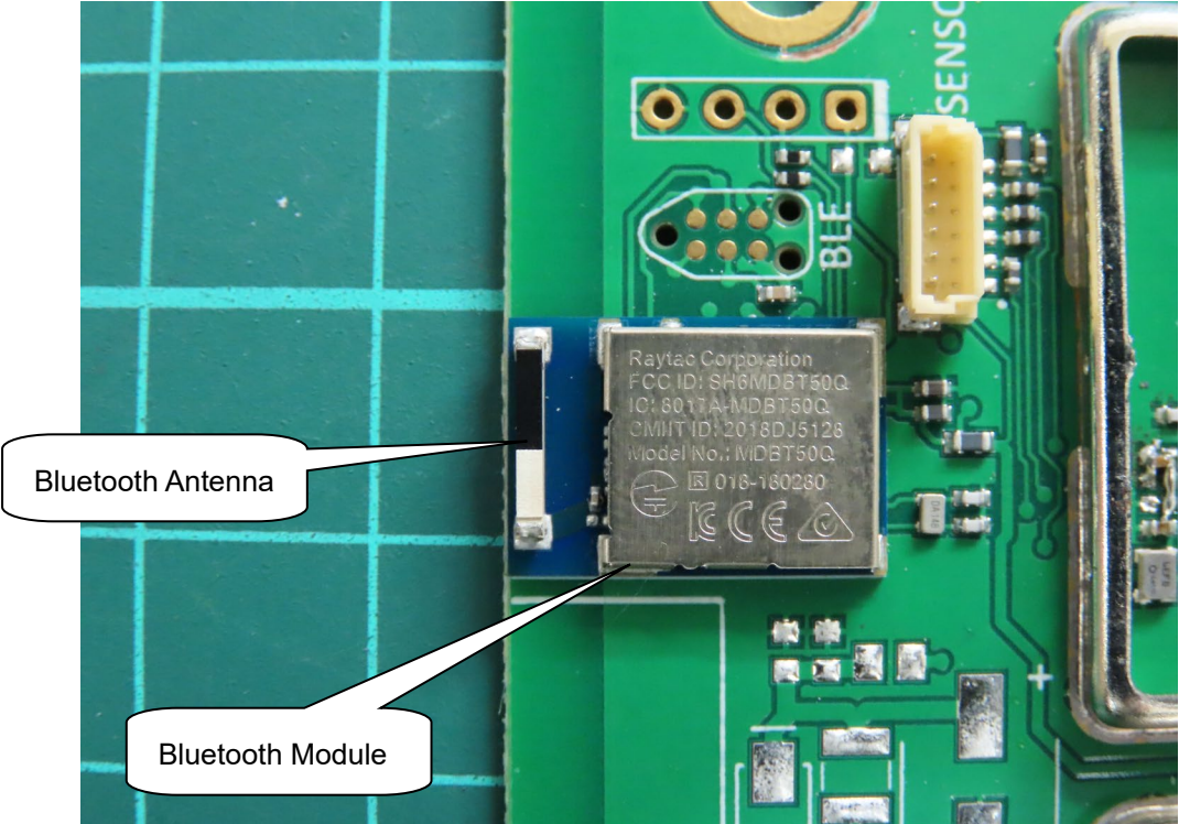
(43) EUT Photo
