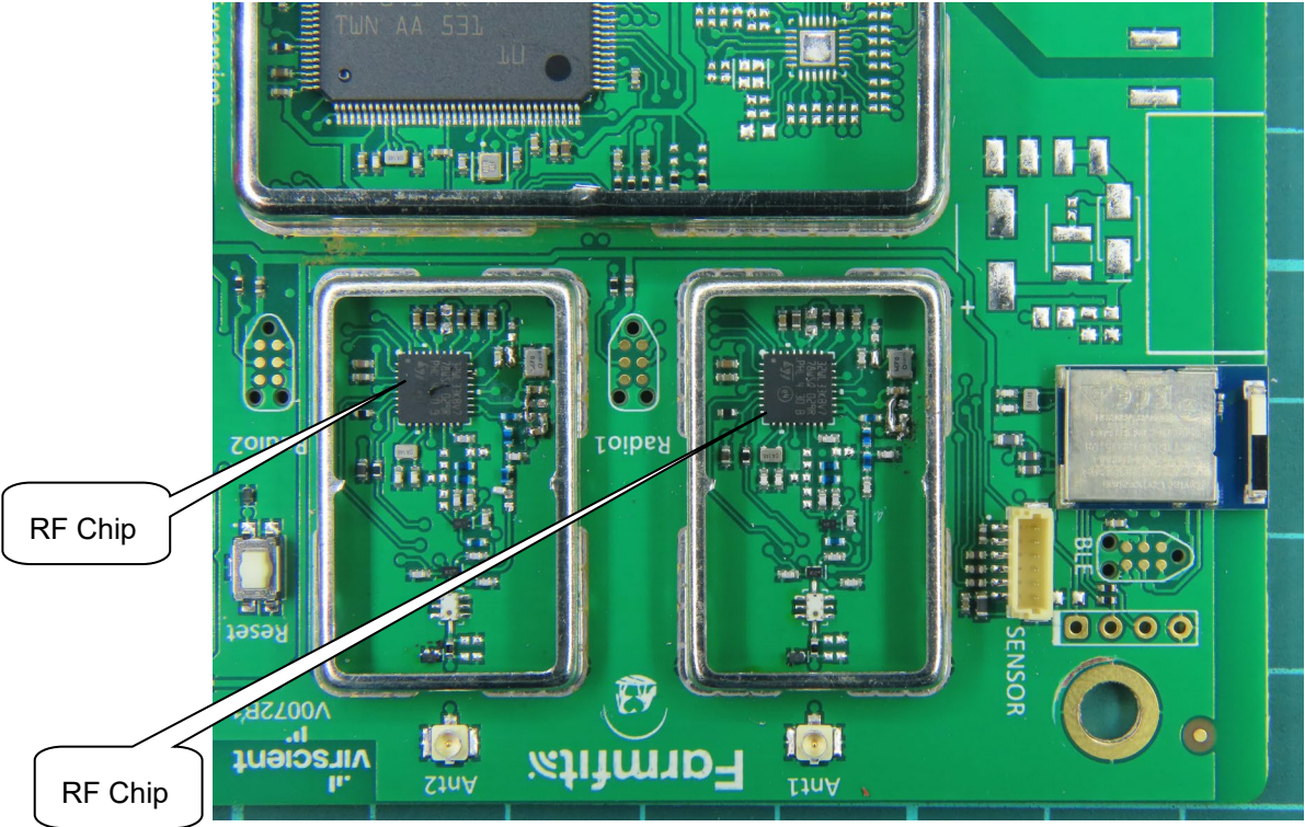
(42) EUT Photo
