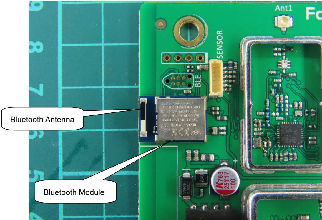
(32) EUT Photo
