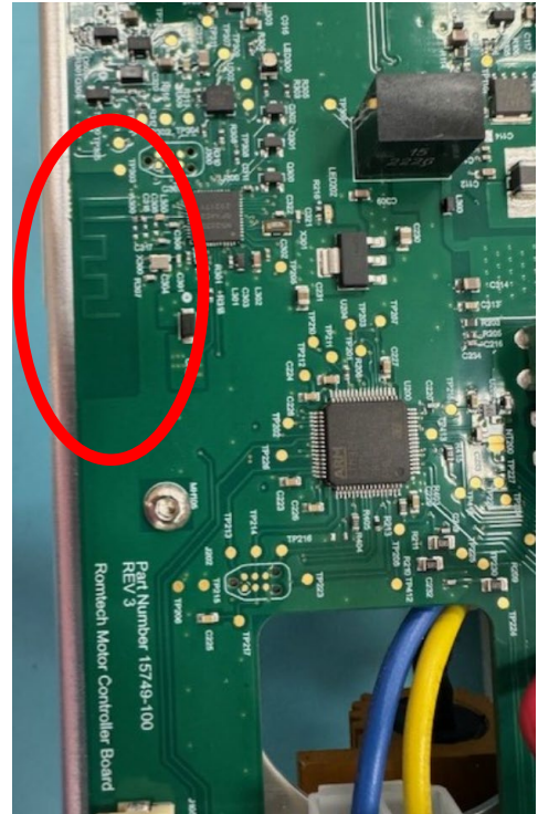
Figure 19; Trace antennae 15749-200 Rev7 for Bluetooth
