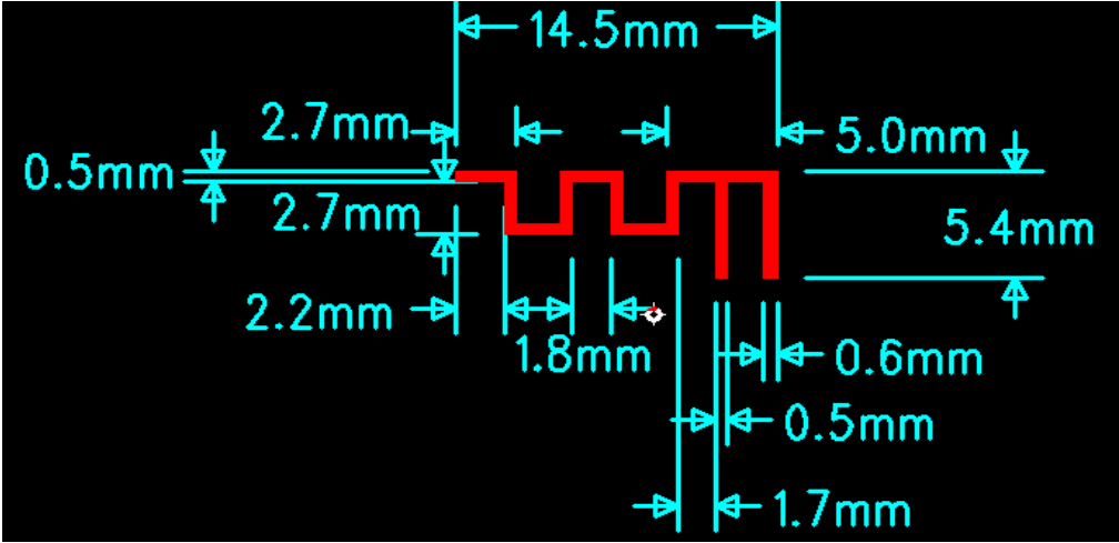
Antenna Dimension
