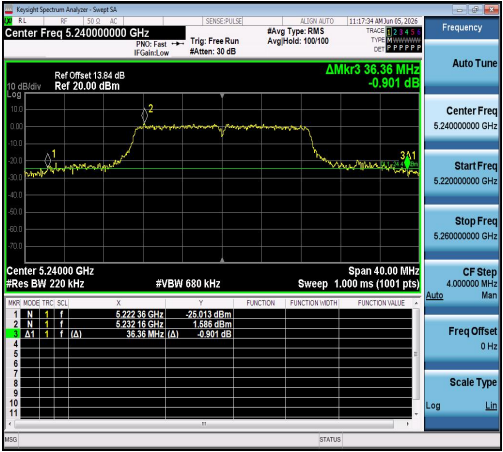
11N20SISO-Ant1-5240
