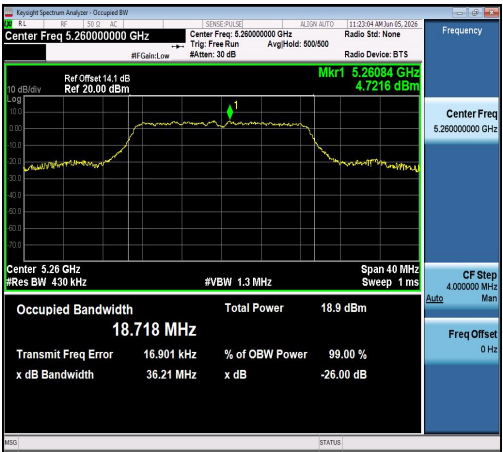
11N20SISO-Ant1-5260
