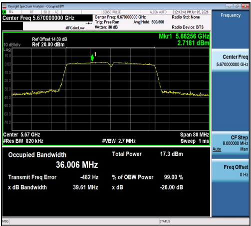
11N40SISO-Ant1-5670
