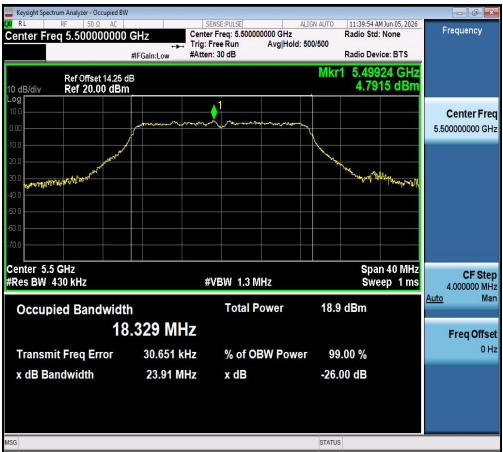
11N20SISO-Ant1-5500
