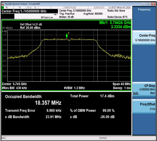
11N20SISO-Ant1-5745
