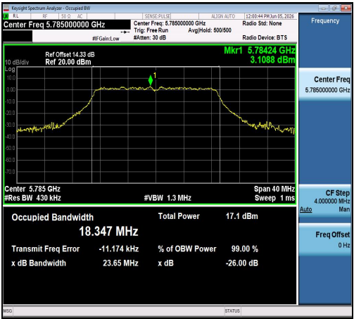
11N20SISO-Ant1-5785
