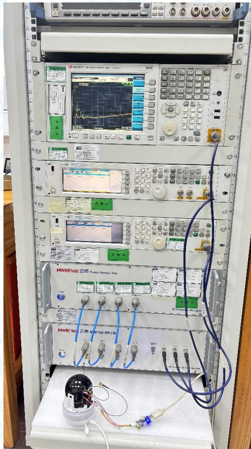
Photo of Setup for RF Conducted----HaLow WIFI
