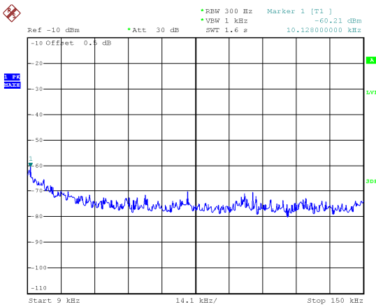
Mode: channel 19
