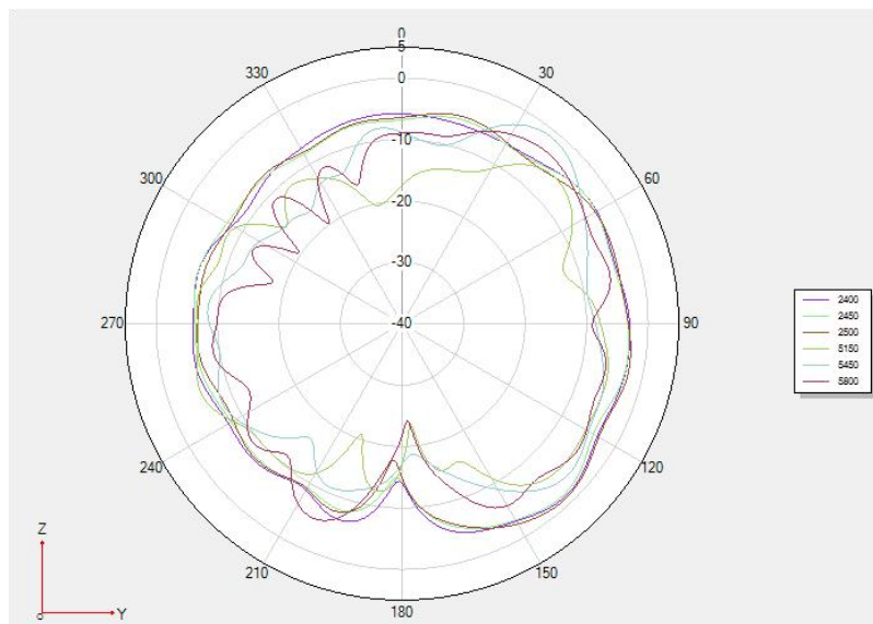
Theta 90 2D
